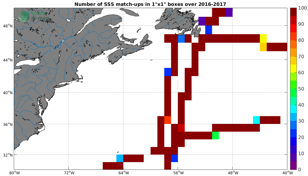
Figure 4: Number of SSS match-ups between TSG-GOSUD-Research-vessel SSS and the SMAP-L3-RSS-V3-MONTHLY-0.25DEG-40KM SSS product for the Gulf Stream Pi-MEP region over 1^\circ \times 1^\circ boxes and for the full satellite product period.
