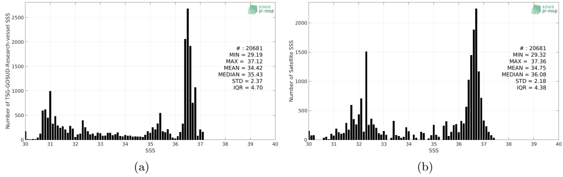
Figure 2: Histograms of SSS from TSG-GOSUD-Research-vessel (a) and SMAP-L3-RSS-V3-MONTHLY-0.25DEG-40KM (b) considering all match-up pairs per bins of 0.1 over the Gulf Stream Pi-MEP region and for the full satellite product period.
