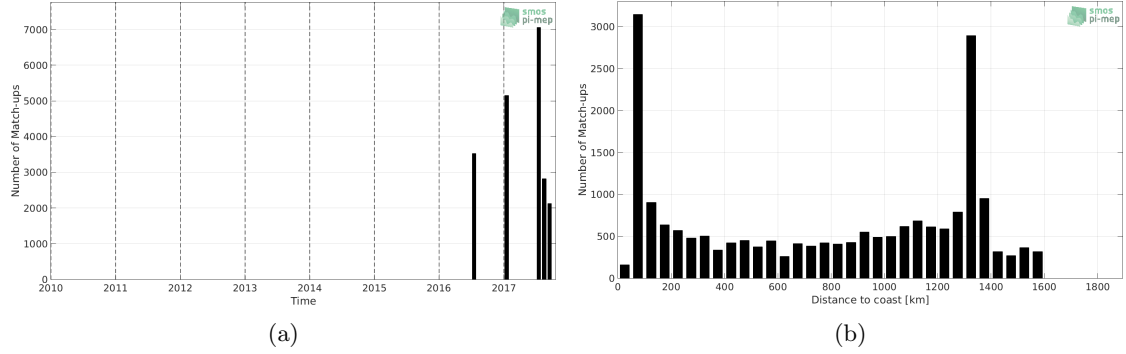
Figure 1: Number of match-ups between TSG-GOSUD-Research-vessel and SMAP-L3-RSS-V3-MONTHLY-0.25DEG-40KM SSS as a function of time (a) and as function of the distance to coast (b) over the Gulf Stream Pi-MEP region and for the full satellite product period.
