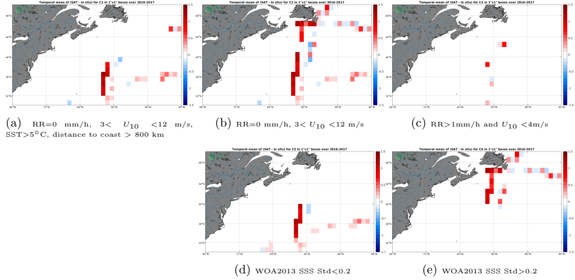
Figure 12: Temporal mean gridded over spatial boxes of size 1^\circ \times 1^\circ of \Delta SSS (SMAP-L3-RSS-V3-MONTHLY-0.25DEG-40KM - TSG-GOSUD-Research-vessel) for 5 different subdatasets corresponding to: RR=0 mm/h, 3 < U_{10} < 12 m/s, SST > 5^\circ C , distance to coast > 800 km (a), RR=0 mm/h, 3 < U_{10} < 12 m/s (b), RR > 1 mm/h and U_{10} < 4 m/s (c), WOA2013 SSS Std < 0.2 (d), WOA2013 SSS Std > 0.2 (e).
