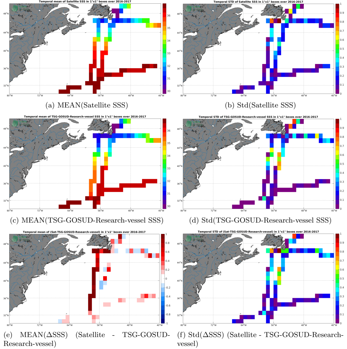
Figure 6: Temporal mean (left) and Std (right) of SSS from SMAP-L3-RSS-V3-MONTHLY-0.25DEG-40KM (top), TSG-GOSUD-Research-vessel (middle), and of \Delta SSS (Satellite - TSG-GOSUD-Research-vessel). Only match-up pairs are used to generate these maps.
