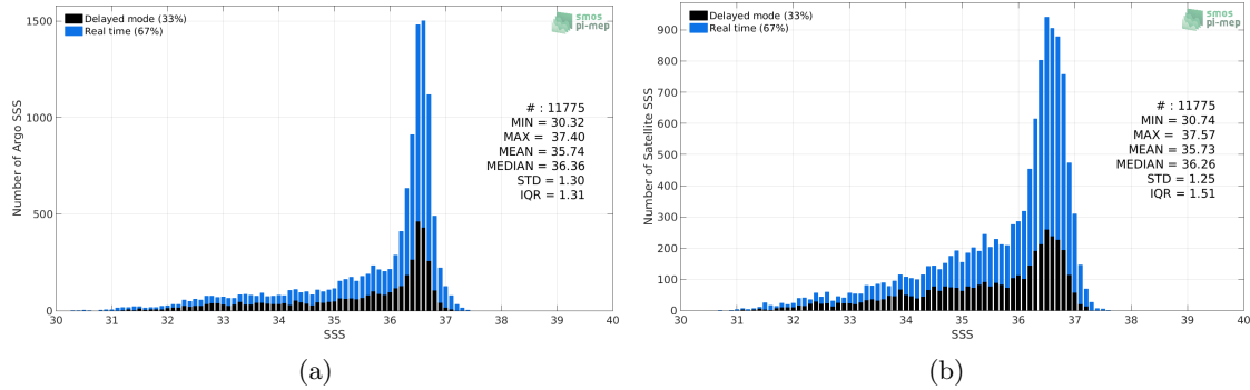
Figure 2: Histograms of SSS from Argo (a) and SMAP-L3-RSS-V3-MONTHLY-0.25DEG-40KM (b) considering all match-up pairs per bins of 0.1 over the Gulf Stream Pi-MEP region and for the full satellite product period.
