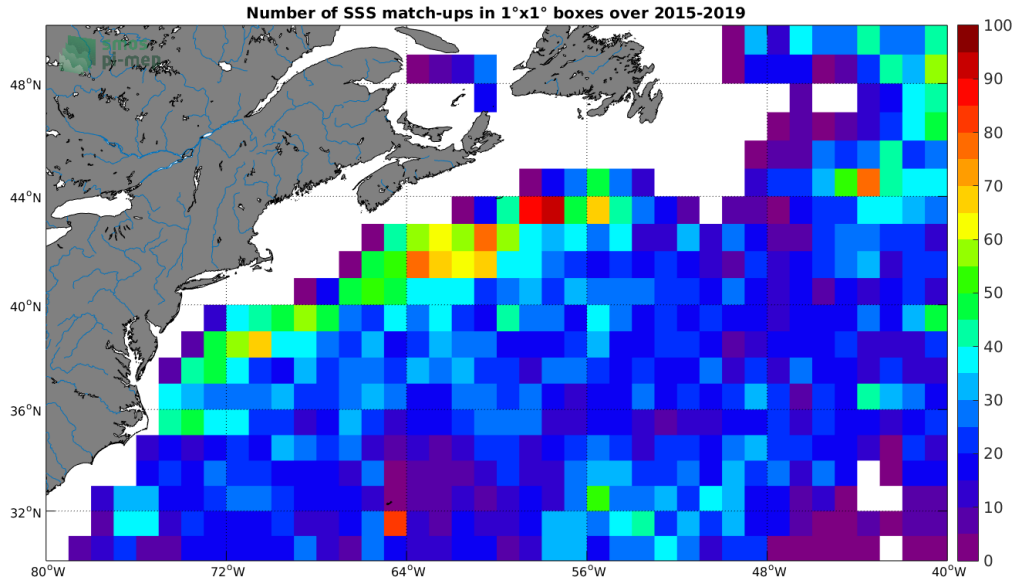
Figure 4: Number of SSS match-ups between Argo SSS and the SMAP-L3-RSS-V3-MONTHLY-0.25DEG-40KM SSS product for the Gulf Stream Pi-MEP region over 1^\circ \times 1^\circ boxes and for the full satellite product period.
