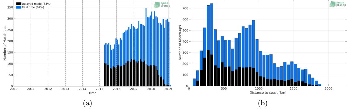
Figure 1: Number of match-ups between Argo and SMAP-L3-RSS-V3-MONTHLY-0.25DEG-40KM SSS as a function of time (a) and as function of the distance to coast (b) over the Gulf Stream Pi-MEP region and for the full satellite product period.
