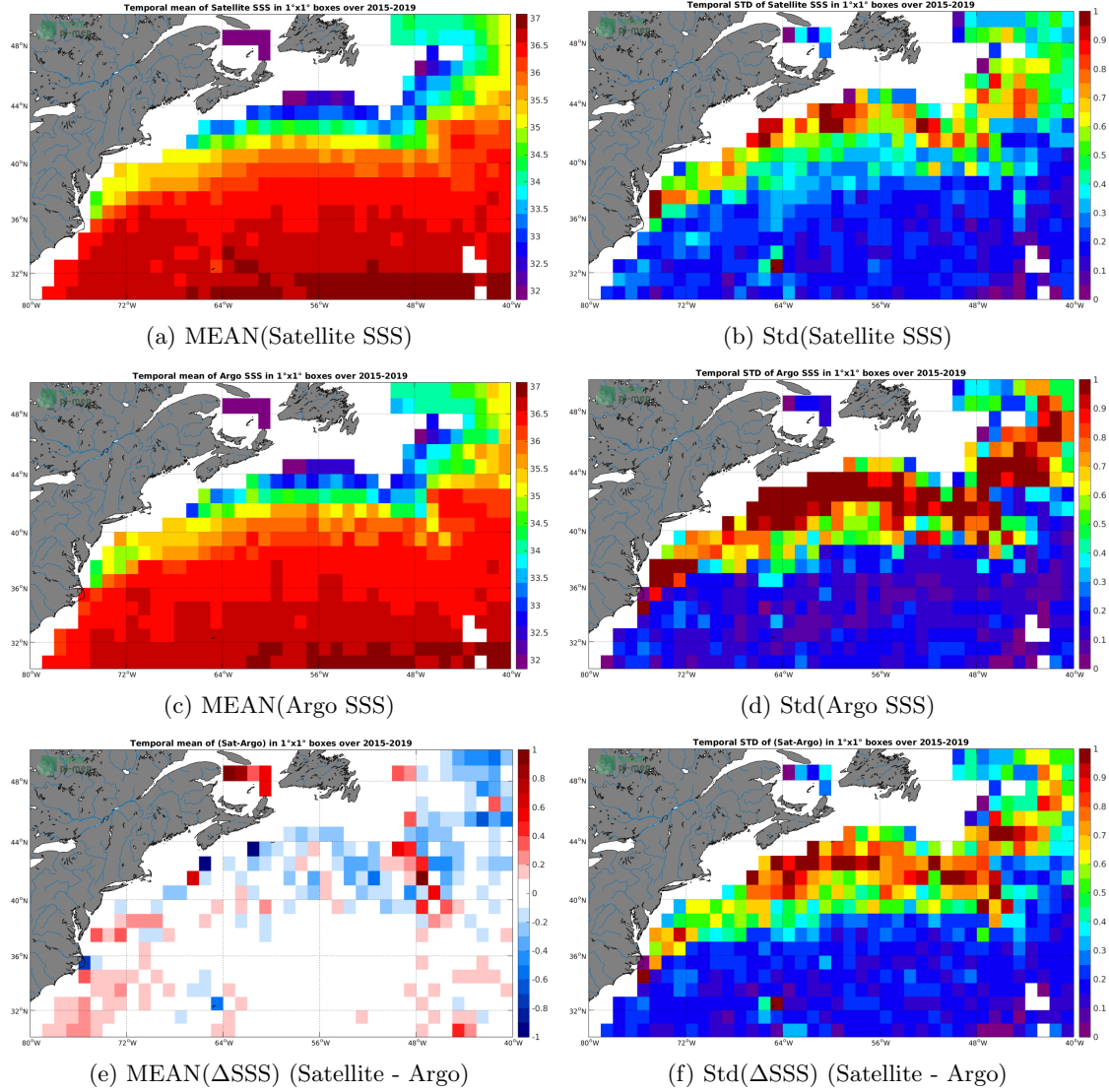
Figure 6: Temporal mean (left) and Std (right) of SSS from SMAP-L3-RSS-V3-MONTHLY-0.25DEG-40KM (top), Argo (middle), and of \Delta SSS (Satellite - Argo). Only match-up pairs are used to generate these maps.
