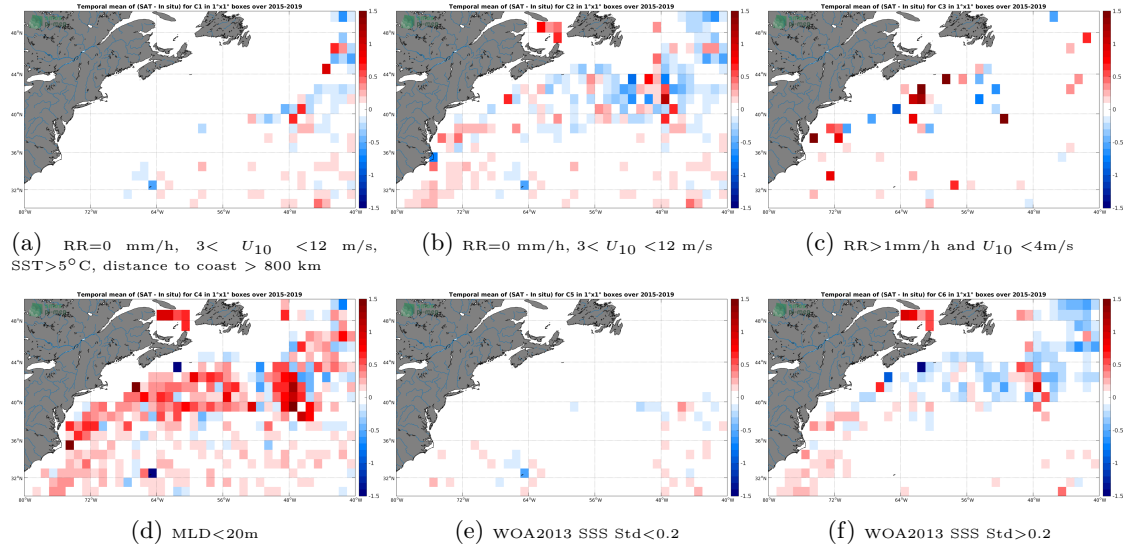
Figure 12: Temporal mean gridded over spatial boxes of size 1^\circ \times 1^\circ of \Delta SSS (SMAP-L3-RSS-V3-MONTHLY-0.25DEG-40KM - Argo) for 6 different subdatasets corresponding to: RR=0 mm/h, 3 < U_{10} < 12 m/s, SST > 5^\circ\text{C} , distance to coast > 800 km (a), RR=0 mm/h, 3 < U_{10} < 12 m/s (b), RR > 1 mm/h and U_{10} < 4 m/s (c), MLD < 20 m (d), WOA2013 SSS Std < 0.2 (e), WOA2013 SSS Std > 0.2 (f).
