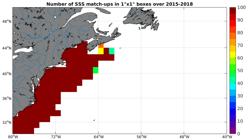
Figure 4: Number of SSS match-ups between TSG-SAMOS SSS and the SMAP-L3-RSS-V2-8DAY-RUNNING-40KM SSS product for the Gulf Stream Pi-MEP region over 1^\circ \times 1^\circ boxes and for the full satellite product period.
