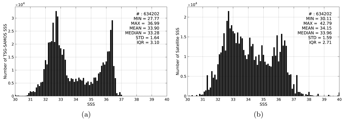
Figure 2: Histograms of SSS from TSG-SAMOS (a) and SMAP-L3-RSS-V2-8DAY-RUNNING-40KM (b) considering all match-up pairs per bins of 0.1 over the Gulf Stream Pi-MEP region and for the full satellite product period.
