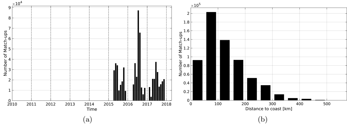
Figure 1: Number of match-ups between TSG-SAMOS and SMAP-L3-RSS-V2-8DAY-RUNNING-40KM SSS as a function of time (a) and as function of the distance to coast (b) over the Gulf Stream Pi-MEP region and for the full satellite product period.
