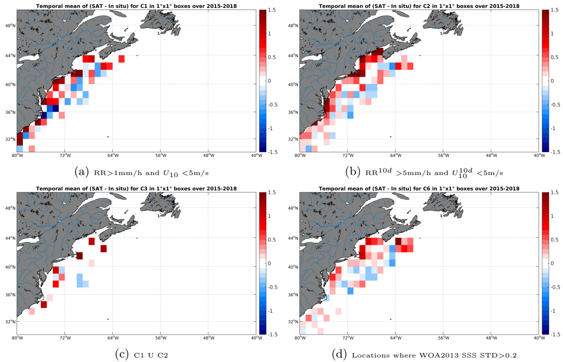
Figure 12: Temporal mean gridded over spatial boxes of size 1^\circ \times 1^\circ of \Delta SSS (SMAP-L3-RSS-V2-8DAY-RUNNING-40KM - TSG-SAMOS) for 4 different subdatasets corresponding to:RR > 1 mm/h and U_{10} < 5 m/s (a), RR^{10d} > 5 mm/h and U_{10}^{10d} < 5 m/s (b), C1 U C2 (c),Locations where WOA2013 SSS STD > 0.2 (d).
