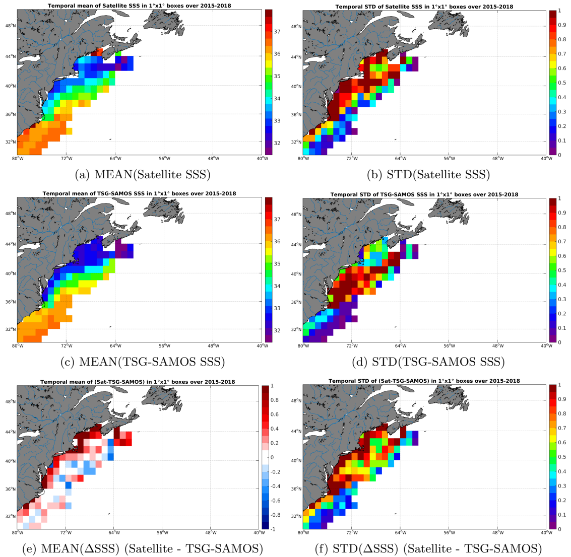
Figure 6: Temporal mean (left) and STD (right) of SSS from SMAP-L3-RSS-V2-8DAY-RUNNING-40KM (top), TSG-SAMOS (middle), and of \Delta SSS (Satellite - TSG-SAMOS). Only match-up pairs are used to generate these maps.
