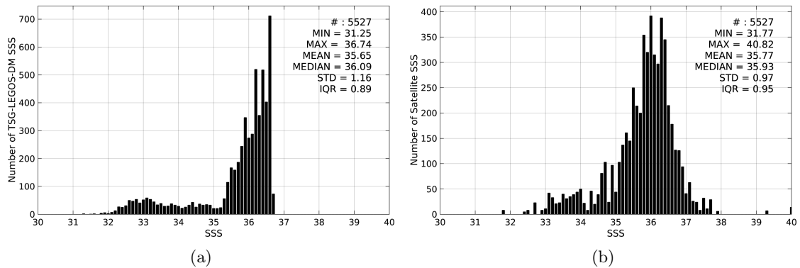
Figure 2: Histograms of SSS from TSG-LEGOS-DM (a) and SMAP-L3-RSS-V2-8DAY-RUNNING-40KM (b) considering all match-up pairs per bins of 0.1 over the Gulf Stream Pi-MEP region and for the full satellite product period.
