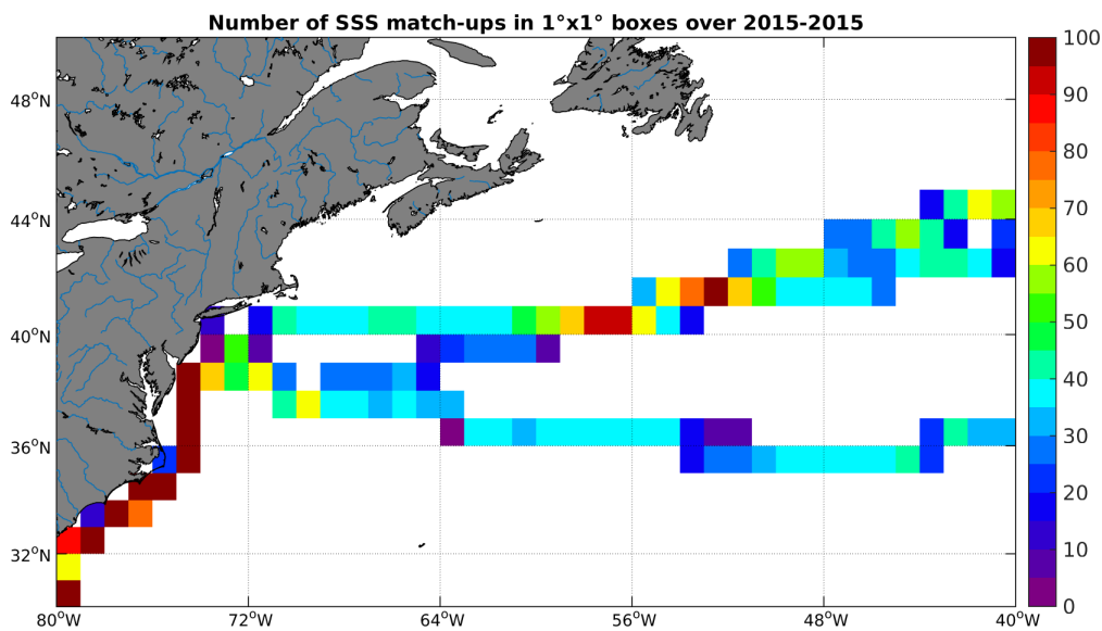
Figure 4: Number of SSS match-ups between TSG-LEGOS-DM SSS and the SMAP-L3-RSS-V2-8DAY-RUNNING-40KM SSS product for the Gulf Stream Pi-MEP region over 1^\circ \times 1^\circ boxes and for the full satellite product period.
