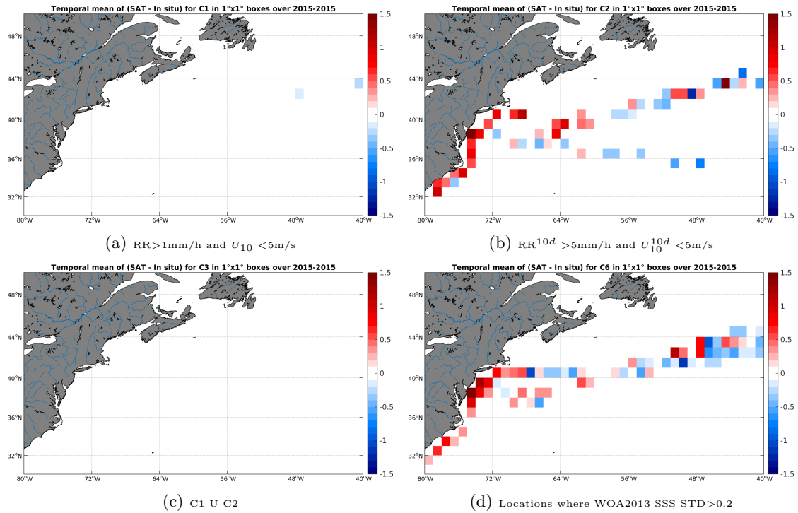
Figure 12: Temporal mean gridded over spatial boxes of size 1^\circ \times 1^\circ of \Delta SSS (SMAP-L3-RSS-V2-8DAY-RUNNING-40KM - TSG-LEGOS-DM) for 4 different subdatasets corresponding to: RR > 1\text{mm/h} and U_{10} < 5\text{m/s} (a), RR^{10d} > 5\text{mm/h} and U_{10}^{10d} < 5\text{m/s} (b), C1 U C2 (c), Locations where WOA2013 SSS STD > 0.2 (d).
