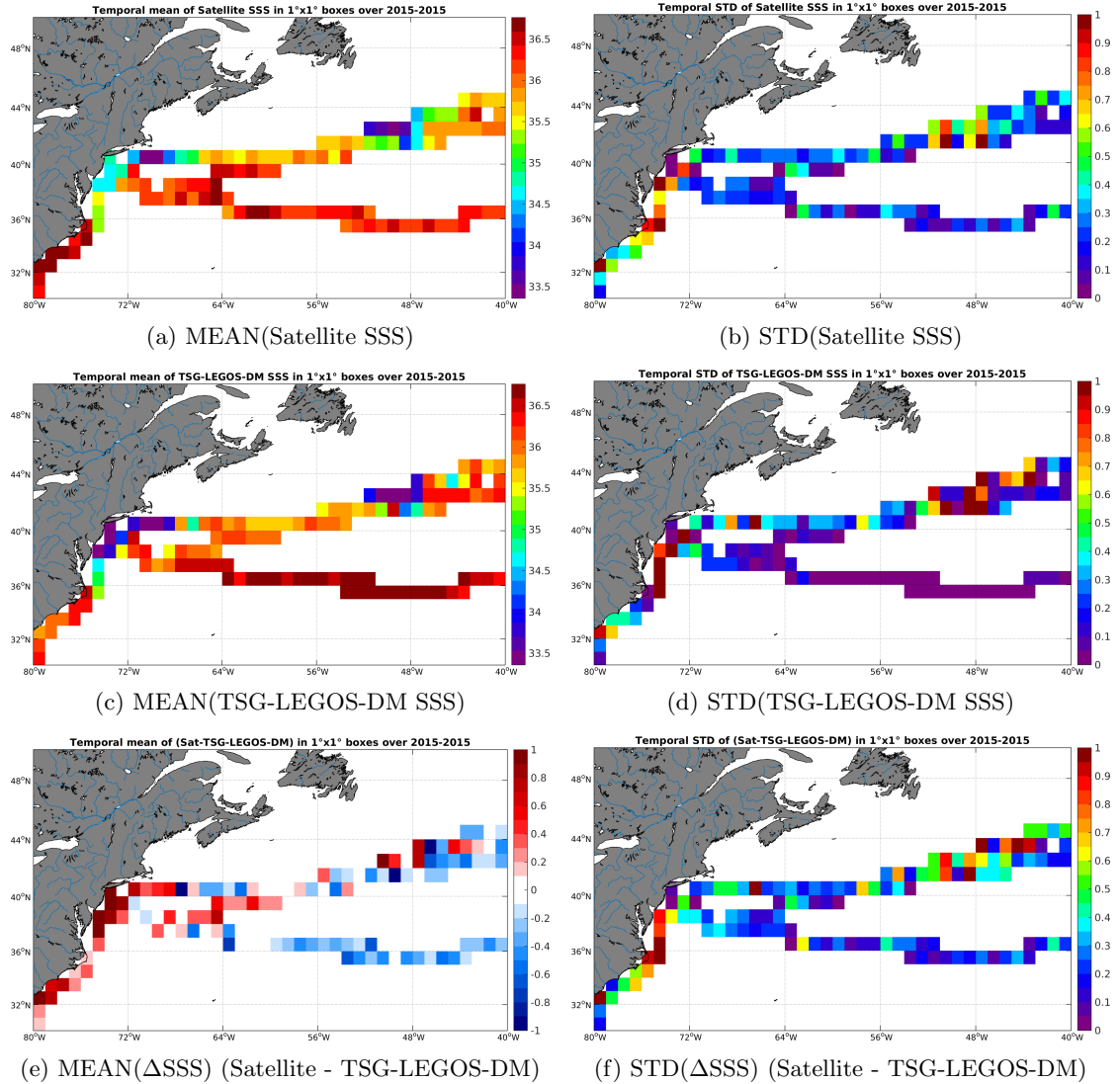
Figure 6: Temporal mean (left) and STD (right) of SSS from SMAP-L3-RSS-V2-8DAY-RUNNING-40KM (top), TSG-LEGOS-DM (middle), and of \Delta SSS (Satellite - TSG-LEGOS-DM). Only match-up pairs are used to generate these maps.
