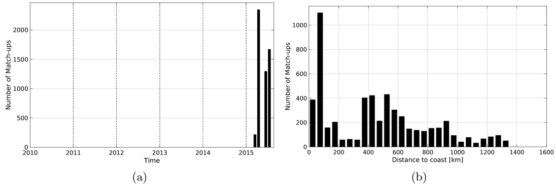
Figure 1: Number of match-ups between TSG-LEGOS-DM and SMAP-L3-RSS-V2-8DAY-RUNNING-40KM SSS as a function of time (a) and as function of the distance to coast (b) over the Gulf Stream Pi-MEP region and for the full satellite product period.
