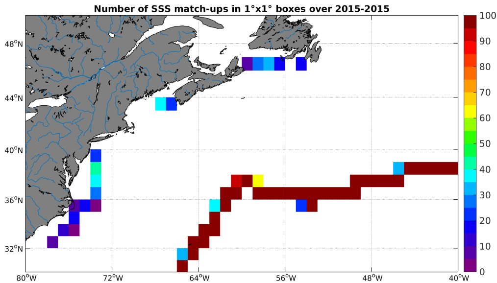
Figure 4: Number of SSS match-ups between TSG-GOSUD-Sailing-ship SSS and the SMAP-L3-RSS-V2-8DAY-RUNNING-40KM SSS product for the Gulf Stream Pi-MEP region over 1^\circ \times 1^\circ boxes and for the full satellite product period.
