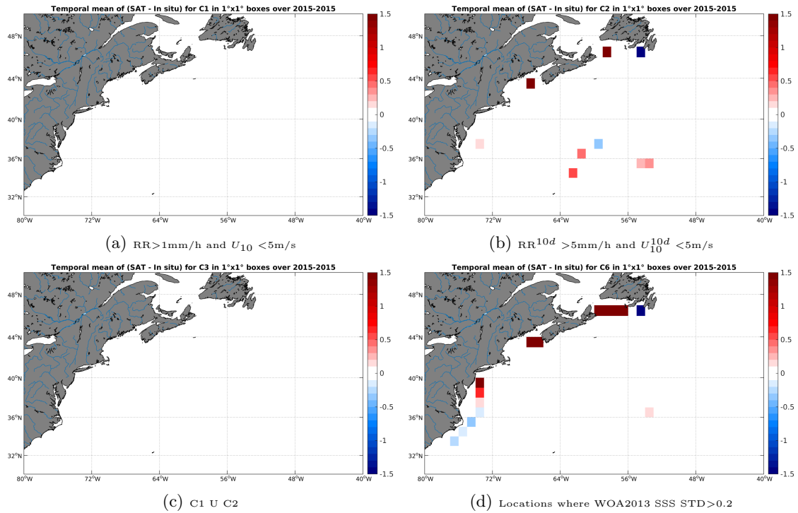
Figure 12: Temporal mean gridded over spatial boxes of size 1^\circ \times 1^\circ of \Delta SSS (SMAP-L3-RSS-V2-8DAY-RUNNING-40KM - TSG-GOSUD-Sailing-ship) for 4 different subdatasets corresponding to: RR > 1mm/h and U_{10} < 5m/s (a), RR 10d > 5mm/h and U_{10}^{10d} < 5m/s (b), C1 U C2 (c), Locations where WOA2013 SSS STD > 0.2 (d).
