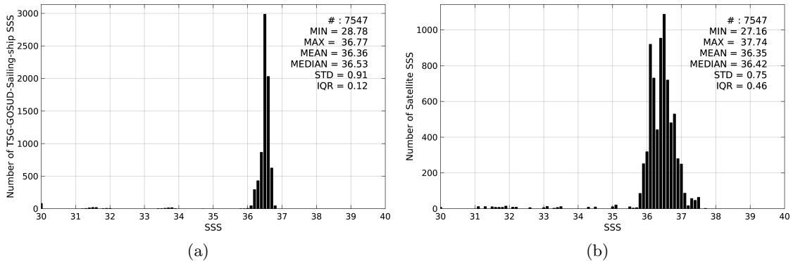
Figure 2: Histograms of SSS from TSG-GOSUD-Sailing-ship (a) and SMAP-L3-RSS-V2-8DAY-RUNNING-40KM (b) considering all match-up pairs per bins of 0.1 over the Gulf Stream Pi-MEP region and for the full satellite product period.
