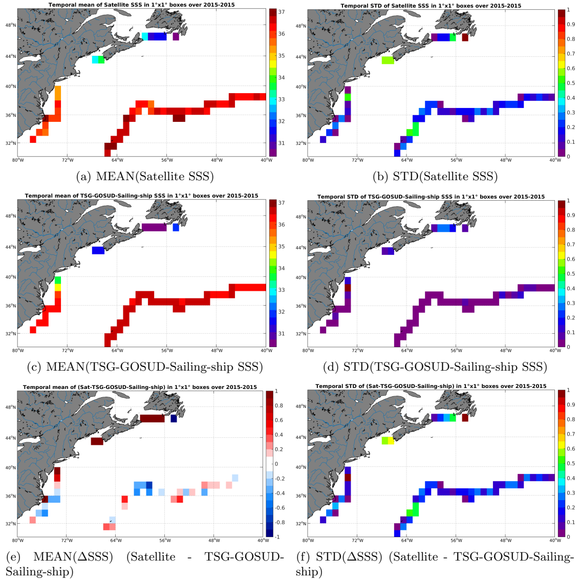
Figure 6: Temporal mean (left) and STD (right) of SSS from SMAP-L3-RSS-V2-8DAY-RUNNING-40KM (top), TSG-GOSUD-Sailing-ship (middle), and of \Delta SSS (Satellite - TSG-GOSUD-Sailing-ship). Only match-up pairs are used to generate these maps.
