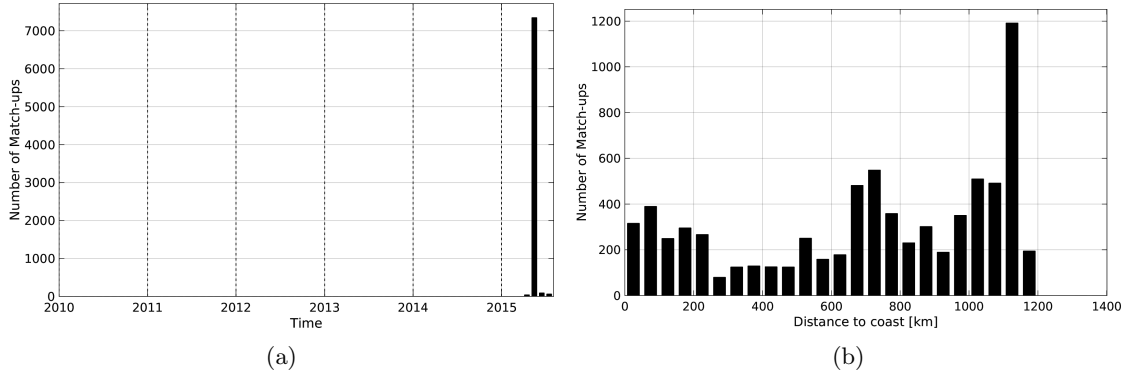
Figure 1: Number of match-ups between TSG-GOSUD-Sailing-ship and SMAP-L3-RSS-V2-8DAY-RUNNING-40KM SSS as a function of time (a) and as function of the distance to coast (b) over the Gulf Stream Pi-MEP region and for the full satellite product period.
