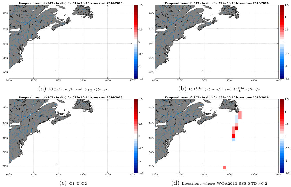
Figure 12: Temporal mean gridded over spatial boxes of size 1^\circ \times 1^\circ of \Delta SSS (SMAP-L3-RSS-V2-8DAY-RUNNING-40KM - TSG-GOSUD-Research-vessel) for 4 different subdatasets corresponding to:RR >1 mm/h and U_{10} < 5 m/s (a), RR^{10d} > 5 mm/h and U_{10}^{10d} < 5 m/s (b), C1 U C2 (c),Locations where WOA2013 SSS STD >0.2 (d).
