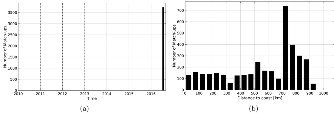
Figure 1: Number of match-ups between TSG-GOSUD-Research-vessel and SMAP-L3-RSS-V2-8DAY-RUNNING-40KM SSS as a function of time (a) and as function of the distance to coast (b) over the Gulf Stream Pi-MEP region and for the full satellite product period.
