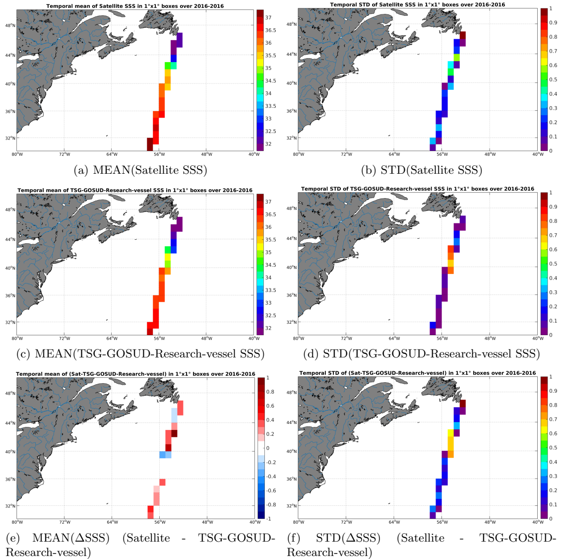
Figure 6: Temporal mean (left) and STD (right) of SSS from SMAP-L3-RSS-V2-8DAY-RUNNING-40KM (top), TSG-GOSUD-Research-vessel (middle), and of \Delta SSS (Satellite - TSG-GOSUD-Research-vessel). Only match-up pairs are used to generate these maps.
