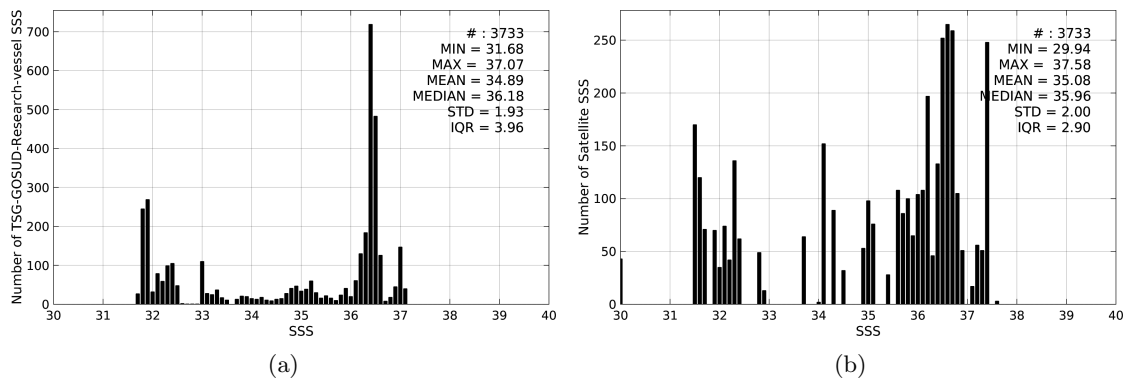
Figure 2: Histograms of SSS from TSG-GOSUD-Research-vessel (a) and SMAP-L3-RSS-V2-8DAY-RUNNING-40KM (b) considering all match-up pairs per bins of 0.1 over the Gulf Stream Pi-MEP region and for the full satellite product period.
