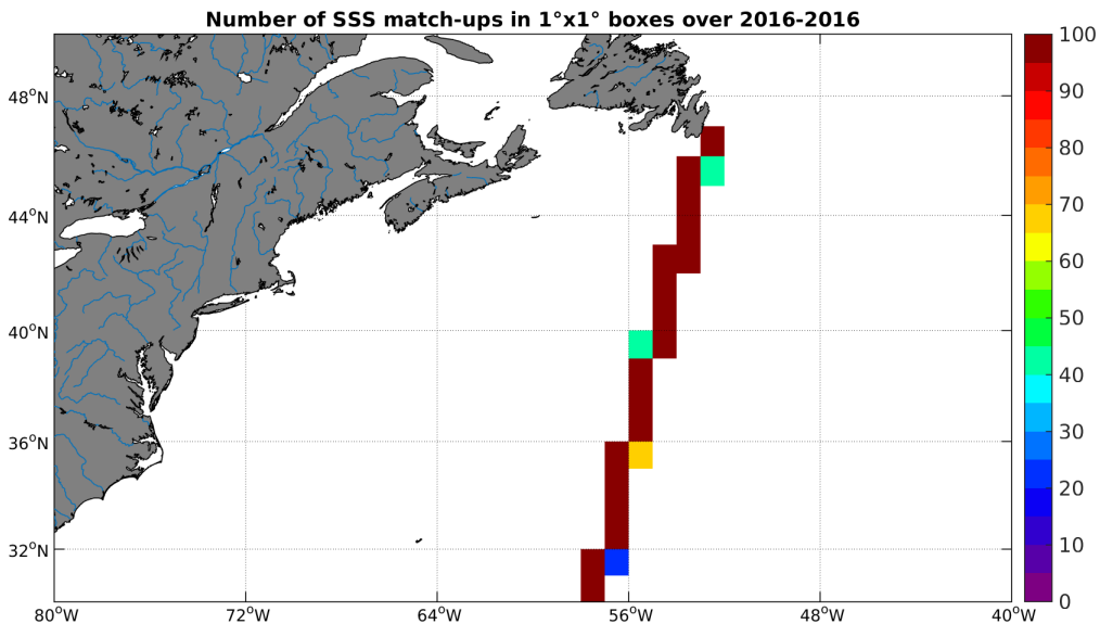
Figure 4: Number of SSS match-ups between TSG-GOSUD-Research-vessel SSS and the SMAP-L3-RSS-V2-8DAY-RUNNING-40KM SSS product for the Gulf Stream Pi-MEP region over 1^\circ \times 1^\circ boxes and for the full satellite product period.
