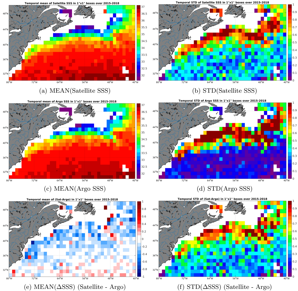
Figure 6: Temporal mean (left) and STD (right) of SSS from SMAP-L3-RSS-V2-8DAY-RUNNING-40KM (top), Argo (middle), and of \Delta SSS (Satellite - Argo). Only match-up pairs are used to generate these maps.
