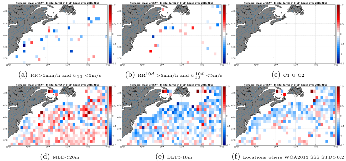
Figure 12: Temporal mean gridded over spatial boxes of size 1^\circ \times 1^\circ of \Delta SSS (SMAP-L3-RSS-V2-8DAY-RUNNING-40KM - Argo) for 6 different subdatasets corresponding to:RR>1mm/h and U_{10} < 5\text{m/s} (a), RR^{10d} > 5\text{mm/h} and U_{10}^{10d} < 5\text{m/s} (b), C1 U C2 (c),MLD<20m (d),BLT>10m (e),Locations where WOA2013 SSS STD>0.2 (f).
