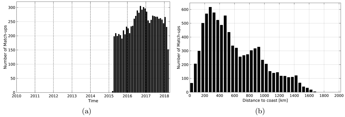
Figure 1: Number of match-ups between Argo and SMAP-L3-RSS-V2-8DAY-RUNNING-40KM SSS as a function of time (a) and as function of the distance to coast (b) over the Gulf Stream Pi-MEP region and for the full satellite product period.
