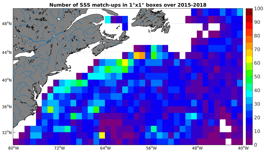
Figure 4: Number of SSS match-ups between Argo SSS and the SMAP-L3-RSS-V2-8DAY-RUNNING-40KM SSS product for the Gulf Stream Pi-MEP region over 1^\circ \times 1^\circ boxes and for the full satellite product period.
