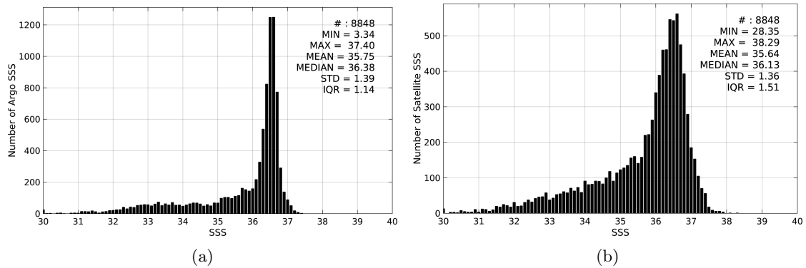
Figure 2: Histograms of SSS from Argo (a) and SMAP-L3-RSS-V2-8DAY-RUNNING-40KM (b) considering all match-up pairs per bins of 0.1 over the Gulf Stream Pi-MEP region and for the full satellite product period.
