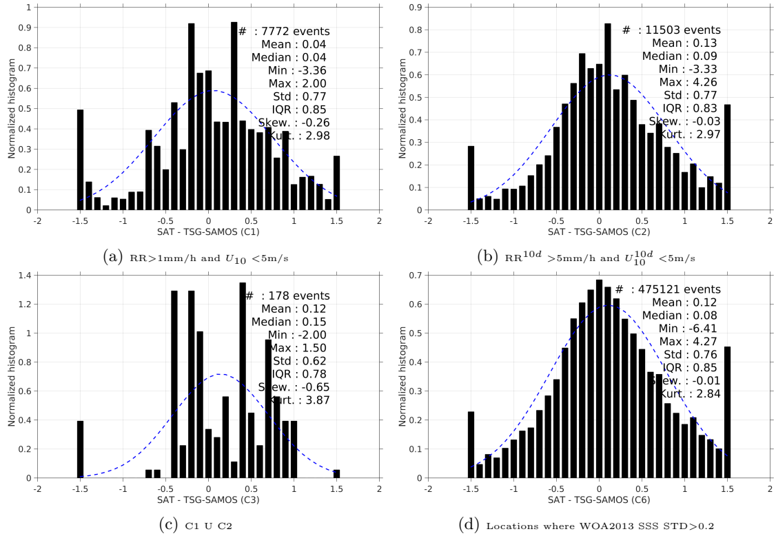
Figure 13: Normalized histogram of \Delta\text{SSS} (SMAP-L3-RSS-V2-8DAY-RUNNING-70KM - TSG-SAMOS) for 6 different subdatasets corresponding to: RR > 1\text{mm/h} and U_{10} < 5\text{m/s} (a), RR^{10d} > 5\text{mm/h} and U_{10}^{10d} < 5\text{m/s} (b), C1 U C2 (c), Locations where WOA2013 SSS STD > 0.2 (d).
