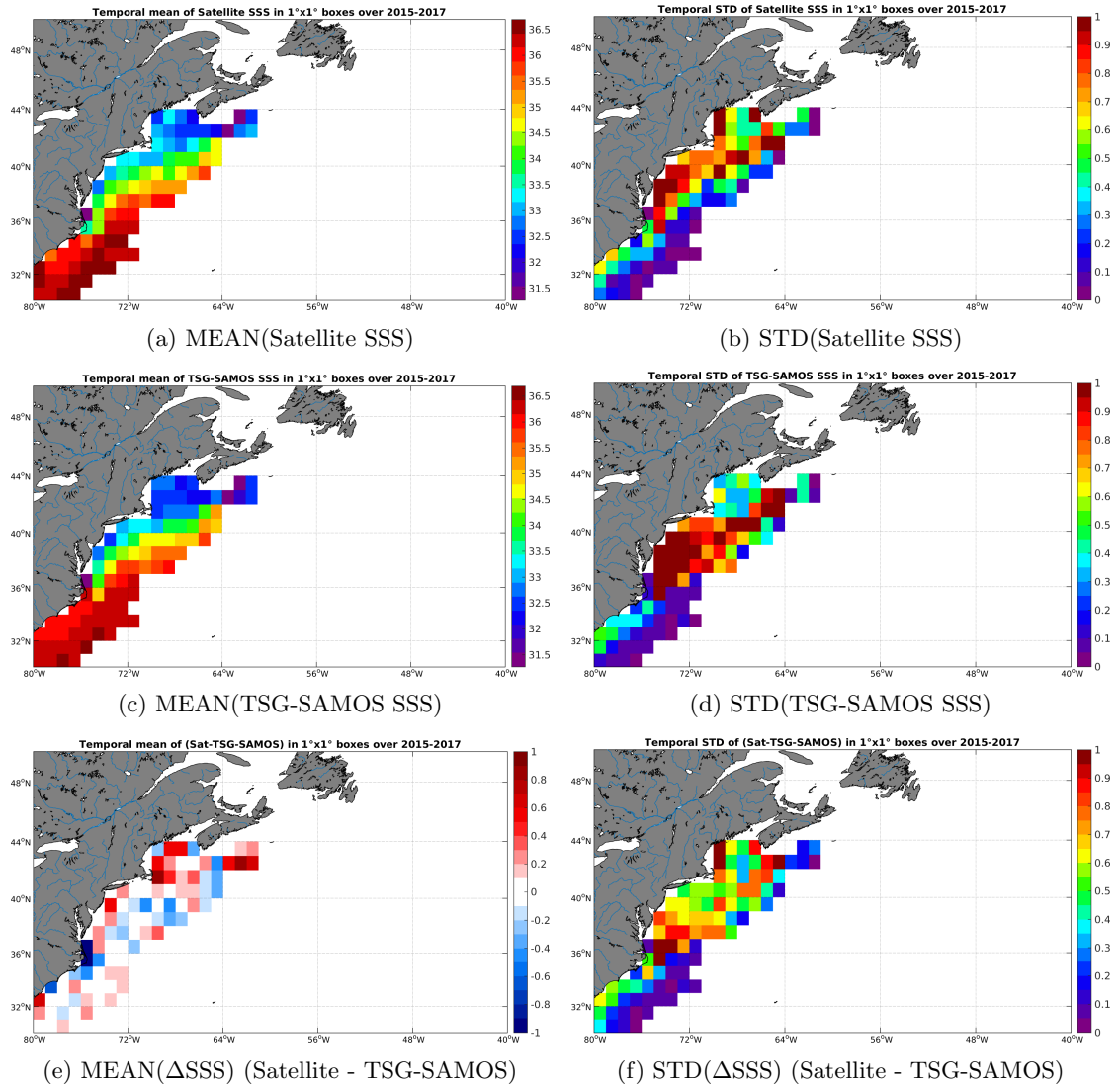
Figure 6: Temporal mean (left) and STD (right) of SSS from SMAP-L3-RSS-V2-8DAY-RUNNING-70KM (top), TSG-SAMOS (middle), and of \Delta SSS (Satellite - TSG-SAMOS). Only match-up pairs are used to generate these maps.
