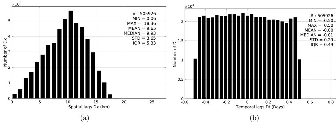
Figure 5: Histograms of the spatial (a) and temporal (b) lags between the time of the TSG-SAMOS measurements and the date of the corresponding SMAP-L3-RSS-V2-8DAY-RUNNING-70KM SSS product.
