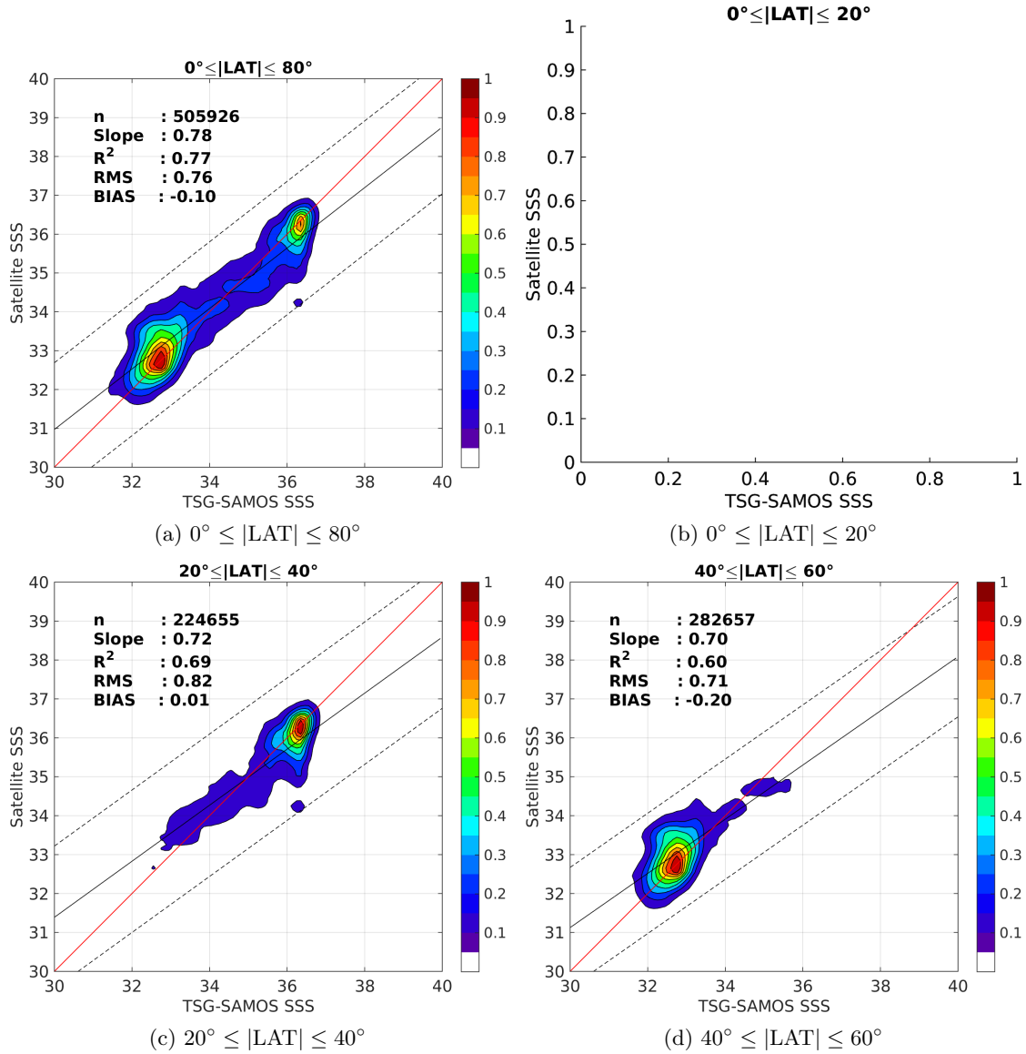
Figure 9: Contour maps of the concentration of SMAP-L3-RSS-V2-8DAY-RUNNING-70KM SSS (y-axis) versus TSG-SAMOS SSS (x-axis) at match-up pairs for different latitude bands. For each plot, the red line shows x=y . The black thin and dashed lines indicate a linear fit through the data cloud and the \pm 95\% confidence levels, respectively. The number match-up pairs n , the slope and R^2 coefficient of the linear fit, the root mean square (RMS) and the mean bias between satellite and in situ data are indicated for each latitude band in each plots.
