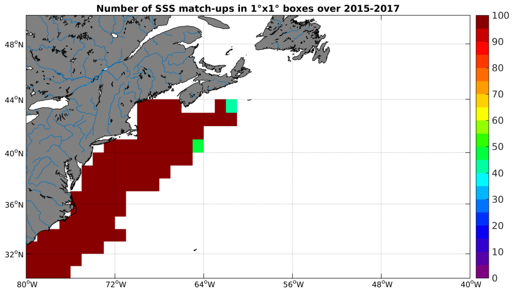
Figure 4: Number of SSS match-ups between TSG-SAMOS SSS and the SMAP-L3-RSS-V2-8DAY-RUNNING-70KM SSS product for the Gulf Stream Pi-MEP region over 1^\circ \times 1^\circ boxes and for the full satellite product period.
