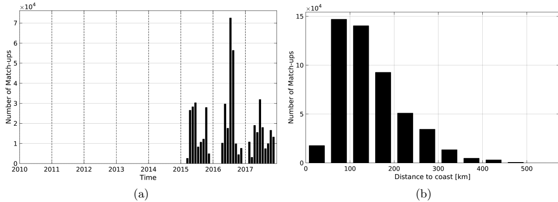
Figure 1: Number of match-ups between TSG-SAMOS and SMAP-L3-RSS-V2-8DAY-RUNNING-70KM SSS as a function of time (a) and as function of the distance to coast (b) over the Gulf Stream Pi-MEP region and for the full satellite product period.
