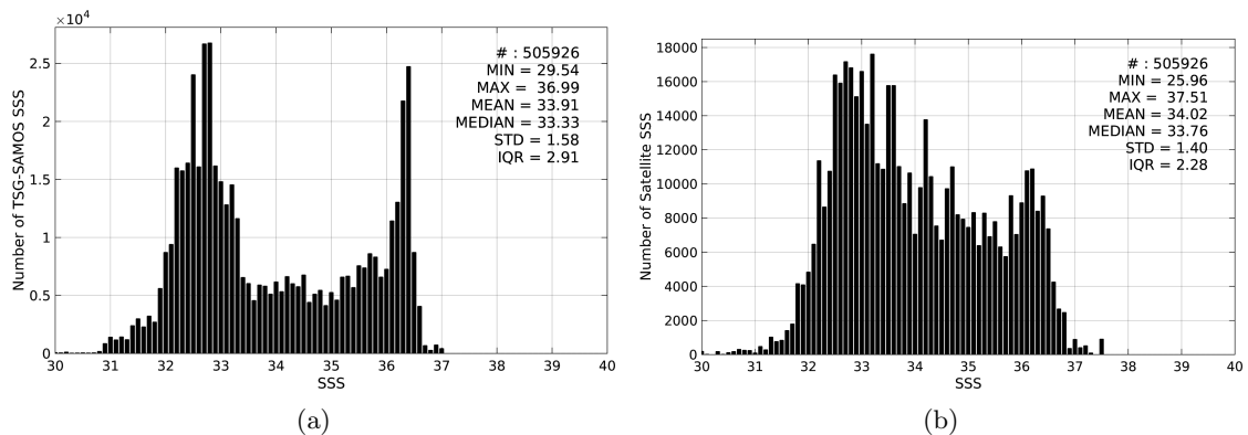
Figure 2: Histograms of SSS from TSG-SAMOS (a) and SMAP-L3-RSS-V2-8DAY-RUNNING-70KM (b) considering all match-up pairs per bins of 0.1 over the Gulf Stream Pi-MEP region and for the full satellite product period.
