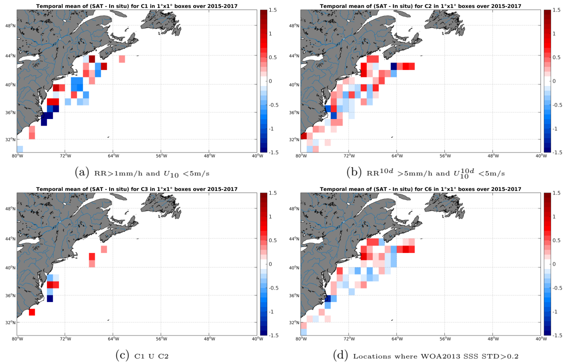
Figure 12: Temporal mean gridded over spatial boxes of size 1^\circ \times 1^\circ of \Delta SSS (SMAP-L3-RSS-V2-8DAY-RUNNING-70KM - TSG-SAMOS) for 4 different subdatasets corresponding to:RR > 1 mm/h and U_{10} < 5 m/s (a), RR^{10d} > 5 mm/h and U_{10}^{10d} < 5 m/s (b), C1 U C2 (c),Locations where WOA2013 SSS STD > 0.2 (d).
