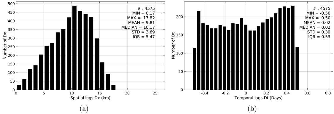
Figure 5: Histograms of the spatial (a) and temporal (b) lags between the time of the TSG-LEGOS-DM measurements and the date of the corresponding SMAP-L3-RSS-V2-8DAY-RUNNING-70KM SSS product.
