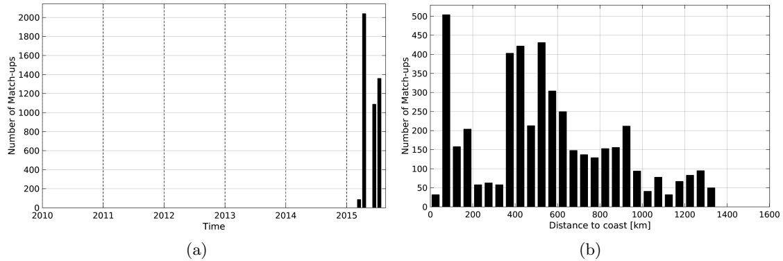
Figure 1: Number of match-ups between TSG-LEGOS-DM and SMAP-L3-RSS-V2-8DAY-RUNNING-70KM SSS as a function of time (a) and as function of the distance to coast (b) over the Gulf Stream Pi-MEP region and for the full satellite product period.
