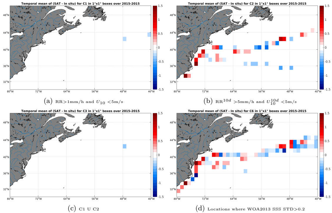
Figure 12: Temporal mean gridded over spatial boxes of size 1^\circ \times 1^\circ of \Delta SSS (SMAP-L3-RSS-V2-8DAY-RUNNING-70KM - TSG-LEGOS-DM) for 4 different subdatasets corresponding to: RR > 1\text{mm/h} and U_{10} < 5\text{m/s} (a), RR^{10d} > 5\text{mm/h} and U_{10}^{10d} < 5\text{m/s} (b), C1 U C2 (c), Locations where WOA2013 SSS STD > 0.2 (d).
