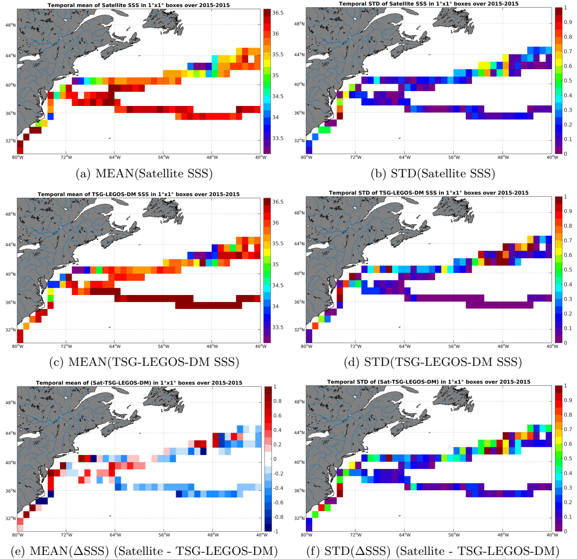
Figure 6: Temporal mean (left) and STD (right) of SSS from SMAP-L3-RSS-V2-8DAY-RUNNING-70KM (top), TSG-LEGOS-DM (middle), and of \Delta SSS (Satellite - TSG-LEGOS-DM). Only match-up pairs are used to generate these maps.
