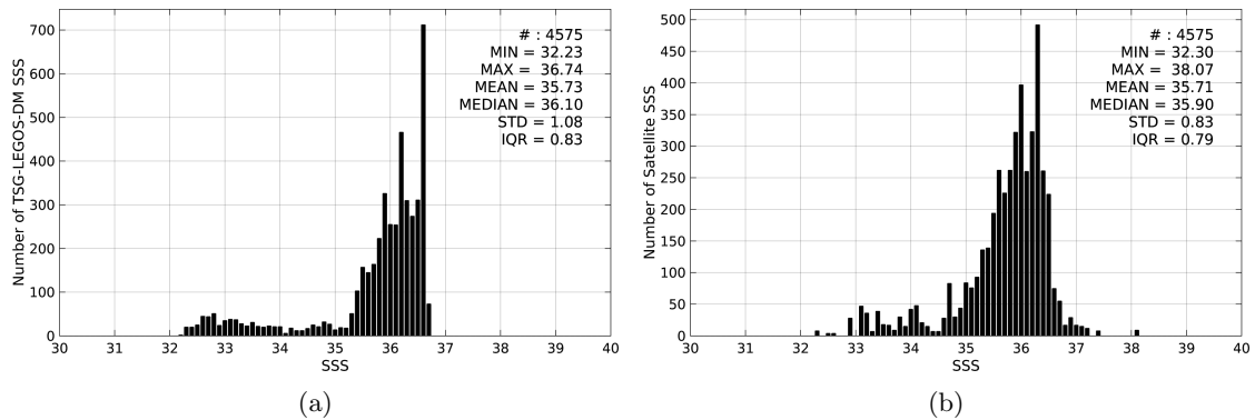
Figure 2: Histograms of SSS from TSG-LEGOS-DM (a) and SMAP-L3-RSS-V2-8DAY-RUNNING-70KM (b) considering all match-up pairs per bins of 0.1 over the Gulf Stream Pi-MEP region and for the full satellite product period.
