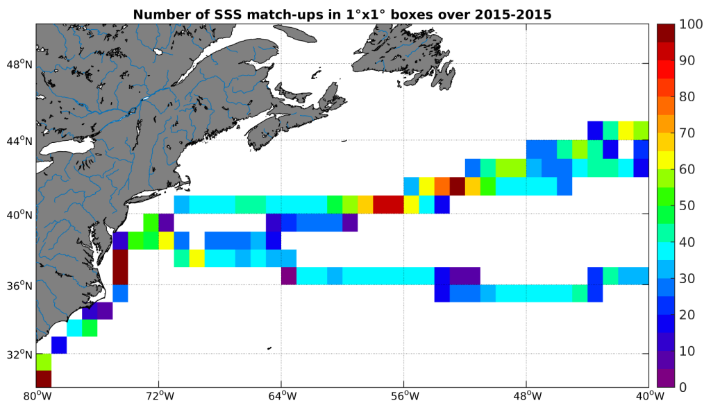
Figure 4: Number of SSS match-ups between TSG-LEGOS-DM SSS and the SMAP-L3-RSS-V2-8DAY-RUNNING-70KM SSS product for the Gulf Stream Pi-MEP region over 1^\circ \times 1^\circ boxes and for the full satellite product period.
