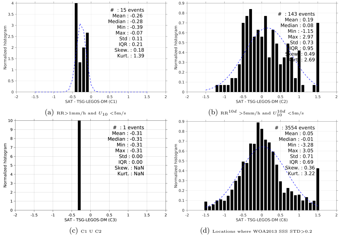
Figure 13: Normalized histogram of \Delta\text{SSS} (SMAP-L3-RSS-V2-8DAY-RUNNING-70KM - TSG-LEGOS-DM) for 6 different subdatasets corresponding to: RR > 1\text{mm/h} and U_{10} < 5\text{m/s} (a), RR^{10d} > 5\text{mm/h} and U_{10}^{10d} < 5\text{m/s} (b), C1 U C2 (c), Locations where WOA2013 SSS STD > 0.2 (d).
