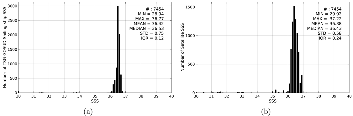
Figure 2: Histograms of SSS from TSG-GOSUD-Sailing-ship (a) and SMAP-L3-RSS-V2-8DAY-RUNNING-70KM (b) considering all match-up pairs per bins of 0.1 over the Gulf Stream Pi-MEP region and for the full satellite product period.
