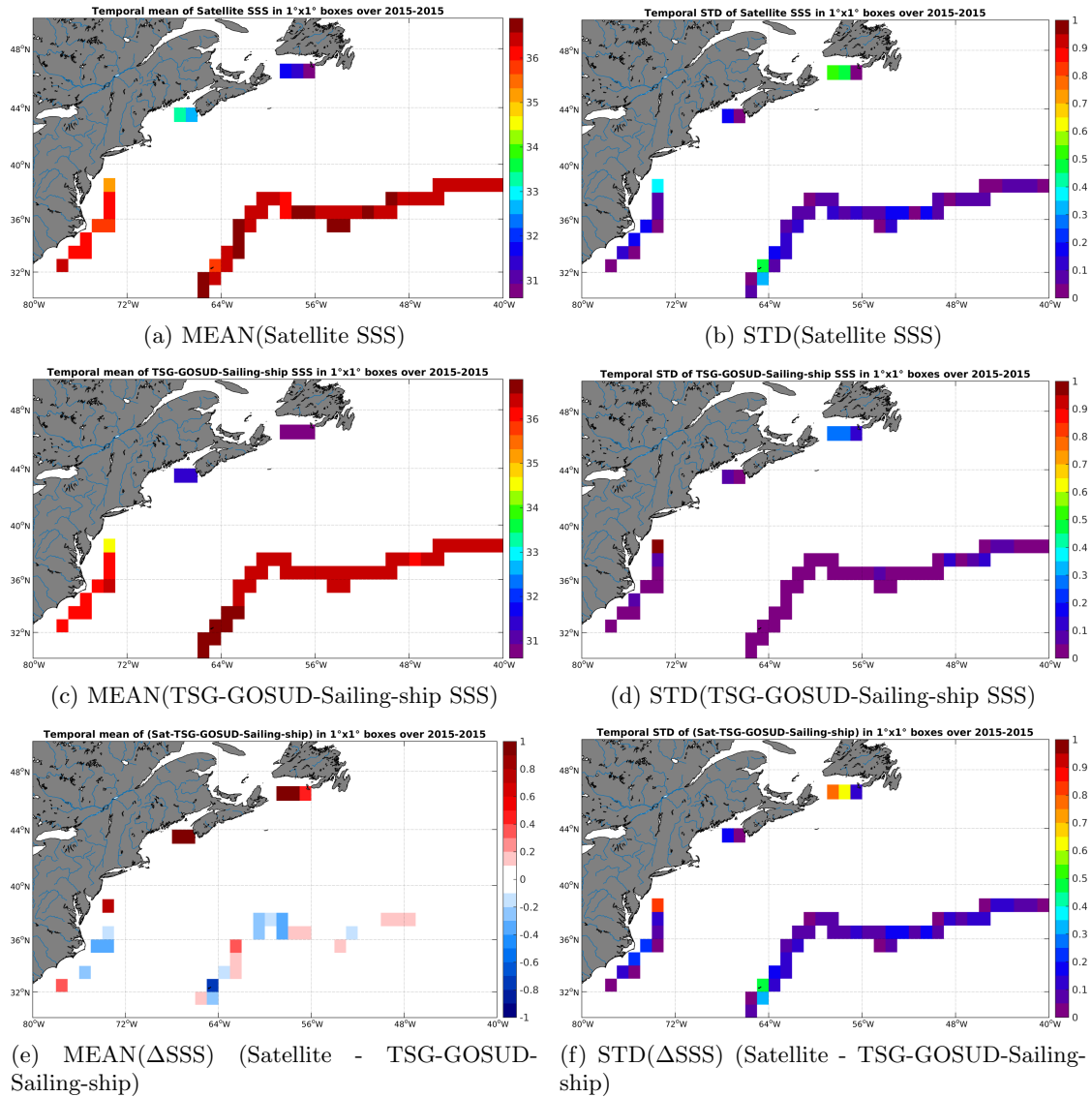
Figure 6: Temporal mean (left) and STD (right) of SSS from SMAP-L3-RSS-V2-8DAY-RUNNING-70KM (top), TSG-GOSUD-Sailing-ship (middle), and of \Delta SSS (Satellite - TSG-GOSUD-Sailing-ship). Only match-up pairs are used to generate these maps.
