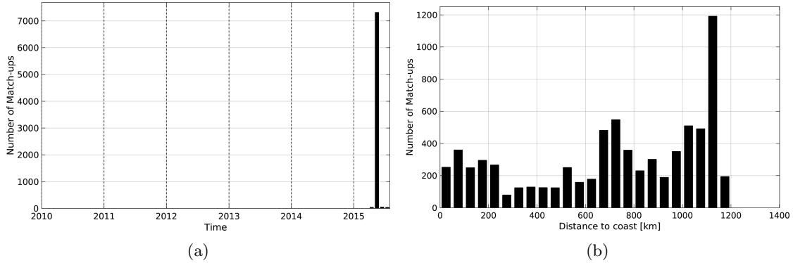
Figure 1: Number of match-ups between TSG-GOSUD-Sailing-ship and SMAP-L3-RSS-V2-8DAY-RUNNING-70KM SSS as a function of time (a) and as function of the distance to coast (b) over the Gulf Stream Pi-MEP region and for the full satellite product period.
