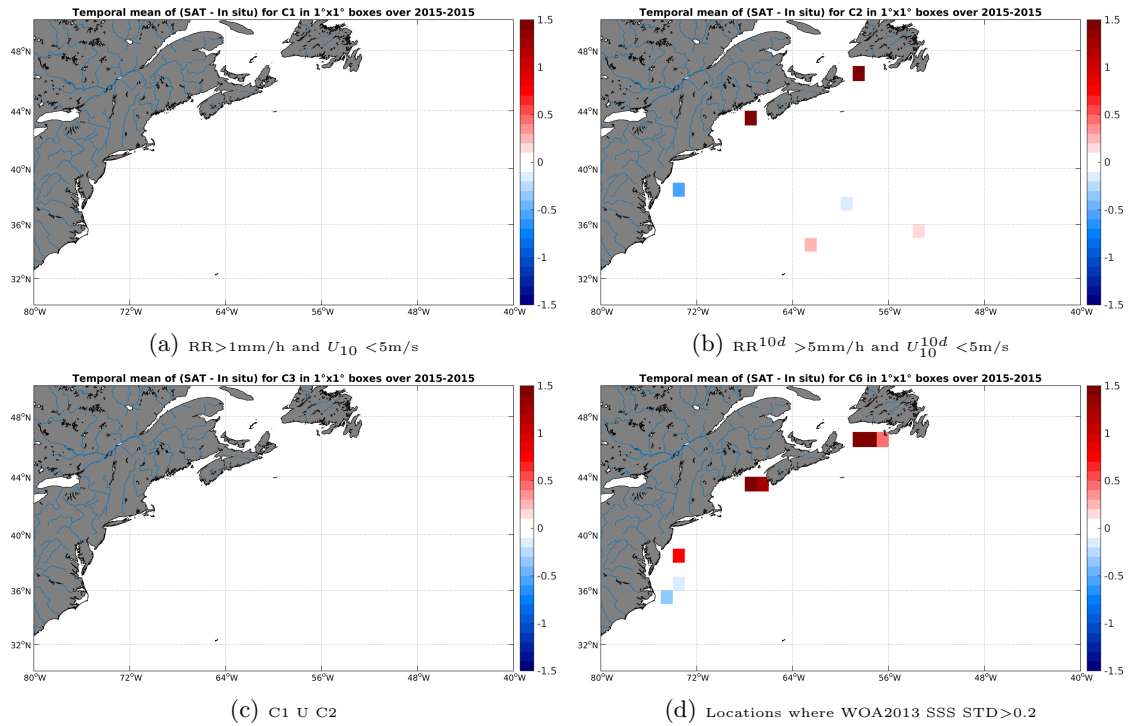
Figure 12: Temporal mean gridded over spatial boxes of size 1^\circ \times 1^\circ of \Delta SSS (SMAP-L3-RSS-V2-8DAY-RUNNING-70KM - TSG-GOSUD-Sailing-ship) for 4 different subdatasets corresponding to: RR > 1\text{mm/h} and U_{10} < 5\text{m/s} (a), RR^{10d} > 5\text{mm/h} and U_{10}^{10d} < 5\text{m/s} (b), C1 U C2 (c), Locations where WOA2013 SSS STD > 0.2 (d).
