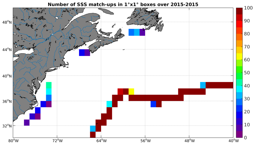
Figure 4: Number of SSS match-ups between TSG-GOSUD-Sailing-ship SSS and the SMAP-L3-RSS-V2-8DAY-RUNNING-70KM SSS product for the Gulf Stream Pi-MEP region over 1°x1° boxes and for the full satellite product period.
