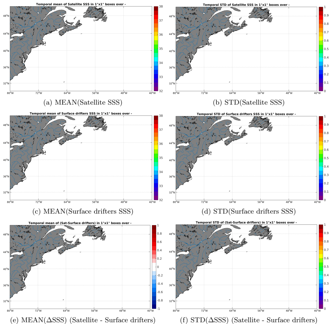
Figure 5: Temporal mean (left) and STD (right) of SSS from SMAP-L3-RSS-V2-8DAY-RUNNING-70KM (top), Surface drifters (middle), and of \Delta SSS (Satellite - Surface drifters). Only match-up pairs are used to generate these maps.
