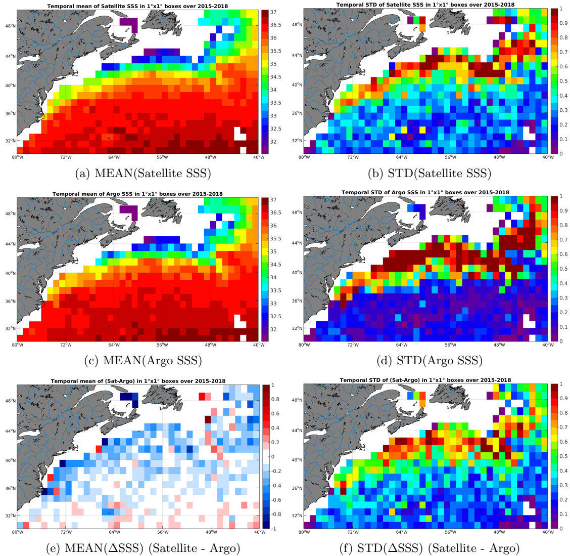
Figure 6: Temporal mean (left) and STD (right) of SSS from SMAP-L3-RSS-V2-8DAY-RUNNING-70KM (top), Argo (middle), and of \Delta SSS (Satellite - Argo). Only match-up pairs are used to generate these maps.
