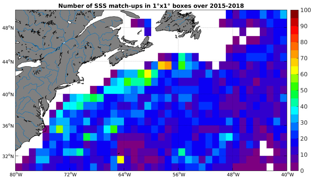
Figure 4: Number of SSS match-ups between Argo SSS and the SMAP-L3-RSS-V2-8DAY-RUNNING-70KM SSS product for the Gulf Stream Pi-MEP region over 1^\circ \times 1^\circ boxes and for the full satellite product period.
