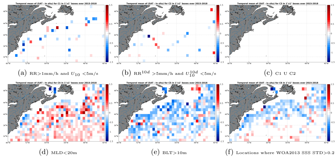
Figure 12: Temporal mean gridded over spatial boxes of size 1^\circ \times 1^\circ of \Delta SSS (SMAP-L3-RSS-V2-8DAY-RUNNING-70KM - Argo) for 6 different subdatasets corresponding to: RR > 1\text{mm/h} and U_{10} < 5\text{m/s} (a), RR^{10d} > 5\text{mm/h} and U_{10}^{10d} < 5\text{m/s} (b), C1 U C2 (c), MLD < 20\text{m} (d), BLT > 10\text{m} (e), Locations where WOA2013 SSS STD > 0.2 (f).
