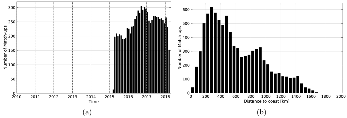
Figure 1: Number of match-ups between Argo and SMAP-L3-RSS-V2-8DAY-RUNNING-70KM SSS as a function of time (a) and as function of the distance to coast (b) over the Gulf Stream Pi-MEP region and for the full satellite product period.
