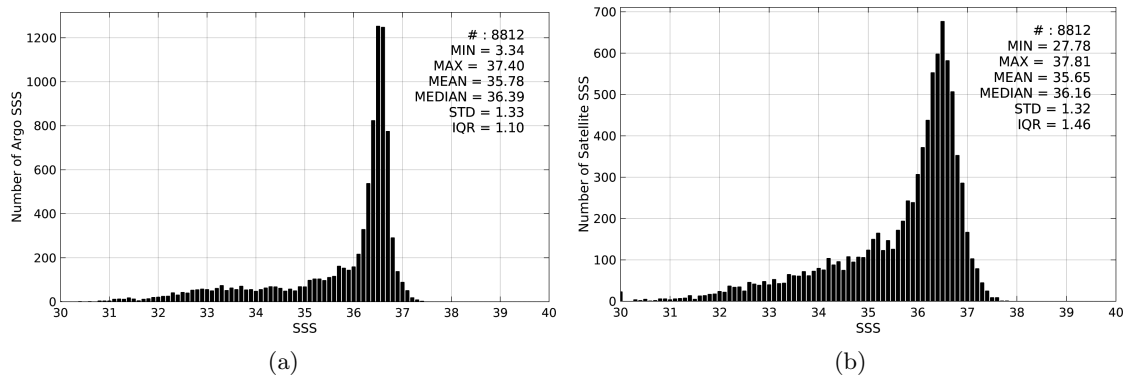
Figure 2: Histograms of SSS from Argo (a) and SMAP-L3-RSS-V2-8DAY-RUNNING-70KM (b) considering all match-up pairs per bins of 0.1 over the Gulf Stream Pi-MEP region and for the full satellite product period.
