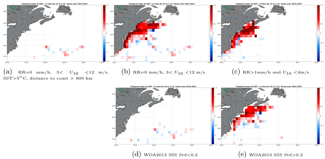
Figure 12: Temporal mean gridded over spatial boxes of size 1^\circ \times 1^\circ of \Delta SSS (SMAP SSS L3 v5.0 - Monthly (JPL) - TSG (SAMOS)) for 5 different subdatasets corresponding to: RR=0 mm/h, 3 < U_{10} < 12 m/s, SST > 5°C, distance to coast > 800 km (a), RR=0 mm/h, 3 < U_{10} < 12 m/s (b), RR > 1mm/h and U_{10} < 4 m/s (c), WOA2013 SSS Std < 0.2 (d), WOA2013 SSS Std > 0.2 (e).
