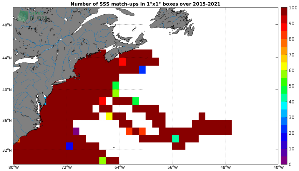
Figure 4: Number of SSS match-ups between TSG (SAMOS) SSS and the SMAP SSS L3 v5.0 - Monthly (JPL) SSS product for the Gulf Stream Pi-MEP region over 1^\circ \times 1^\circ boxes and for the full satellite product period.
