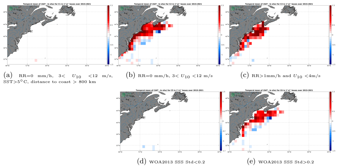
Figure 12: Temporal mean gridded over spatial boxes of size 1°x1° of \Delta SSS (SMAP SSS L3 v5.0 - Monthly (JPL) - TSG (SAMOS)) for 5 different subdatasets corresponding to:RR=0 mm/h, 3 < U_{10} < 12 m/s, SST>5°C, distance to coast > 800 km (a), RR=0 mm/h, 3 < U_{10} < 12 m/s (b), RR>1mm/h and U_{10} < 4 m/s (c), WOA2013 SSS Std<0.2 (d), WOA2013 SSS Std>0.2 (e).
