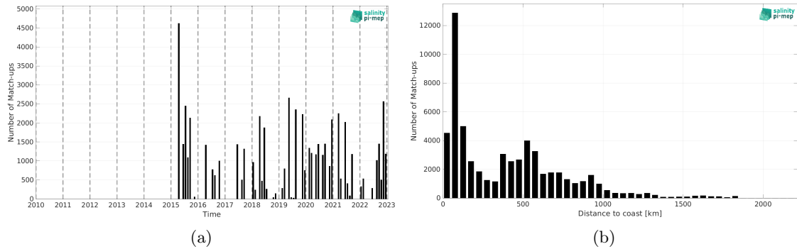
Figure 2: Number of match-ups between TSG (LEGOS-DM) and SMAP SSS L3 v5.0 - Monthly (JPL) SSS as a function of time (a) and as function of the distance to coast (b) over the Gulf Stream Pi-MEP region and for the full satellite product period.
