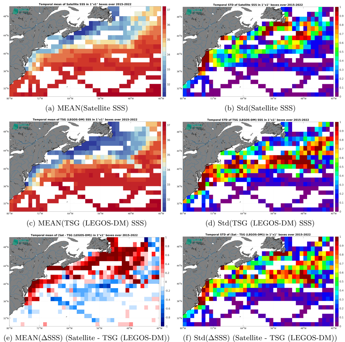
Figure 7: Temporal mean (left) and Std (right) of SSS from SMAP SSS L3 v5.0 - Monthly (JPL) (top), TSG (LEGOS-DM) (middle), and of \Delta SSS (Satellite - TSG (LEGOS-DM)). Only match-up pairs are used to generate these maps.
