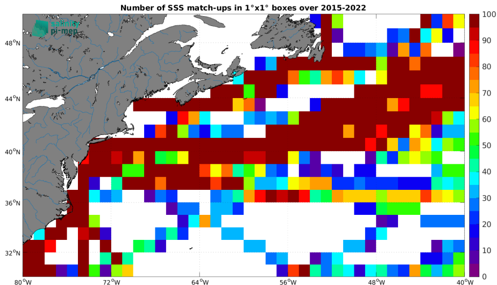
Figure 5: Number of SSS match-ups between TSG (LEGOS-DM) SSS and the SMAP SSS L3 v5.0 - Monthly (JPL) SSS product for the Gulf Stream Pi-MEP region over 1^\circ \times 1^\circ boxes and for the full satellite product period.
