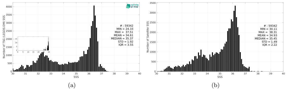
Figure 3: Histograms of SSS from TSG (LEGOS-DM) (a) and SMAP SSS L3 v5.0 - Monthly (JPL) (b) considering all match-up pairs per bins of 0.1 over the Gulf Stream Pi-MEP region and for the full satellite product period.
