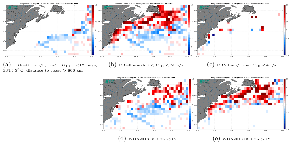
Figure 14: Temporal mean gridded over spatial boxes of size 1^\circ \times 1^\circ of \Delta SSS (SMAP SSS L3 v5.0 - Monthly (JPL) - TSG (LEGOS-DM)) for 5 different subdatasets corresponding to:RR=0 mm/h, 3 < U_{10} < 12 m/s, SST > 5^\circ\text{C} , distance to coast > 800 km (a), RR=0 mm/h, 3 < U_{10} < 12 m/s (b), RR > 1 mm/h and U_{10} < 4 m/s (c), WOA2013 SSS Std < 0.2 (d), WOA2013 SSS Std > 0.2 (e).
