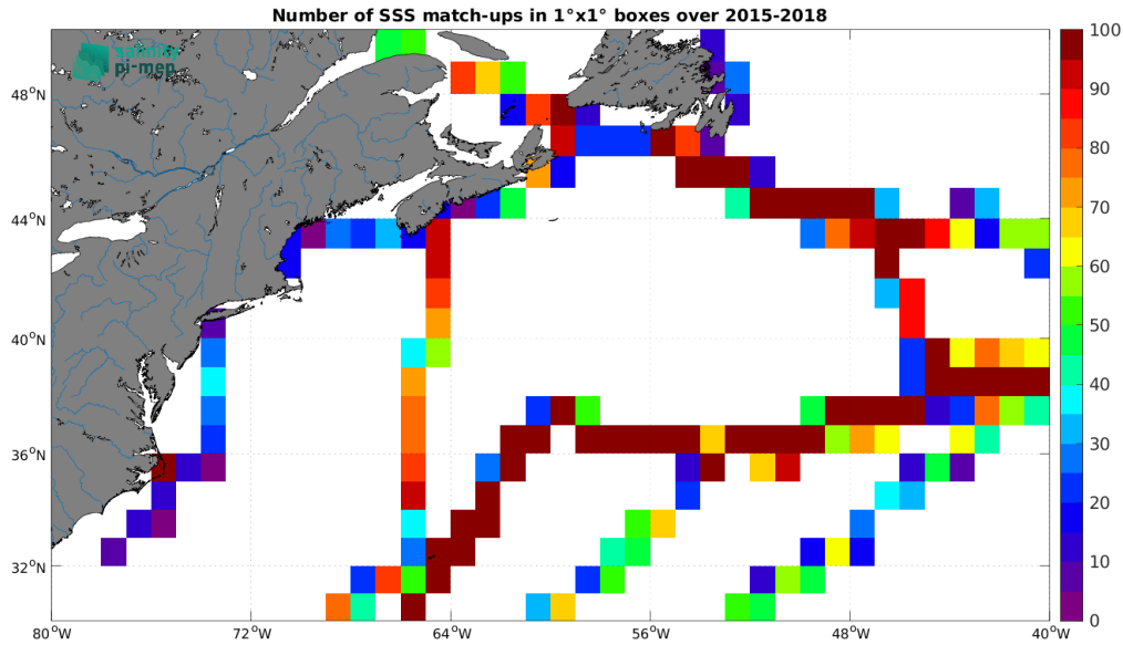
Figure 5: Number of SSS match-ups between TSG (GOSUD-Sailing-ship) SSS and the SMAP SSS L3 v5.0 - Monthly (JPL) SSS product for the Gulf Stream Pi-MEP region over 1^\circ \times 1^\circ boxes and for the full satellite product period.
