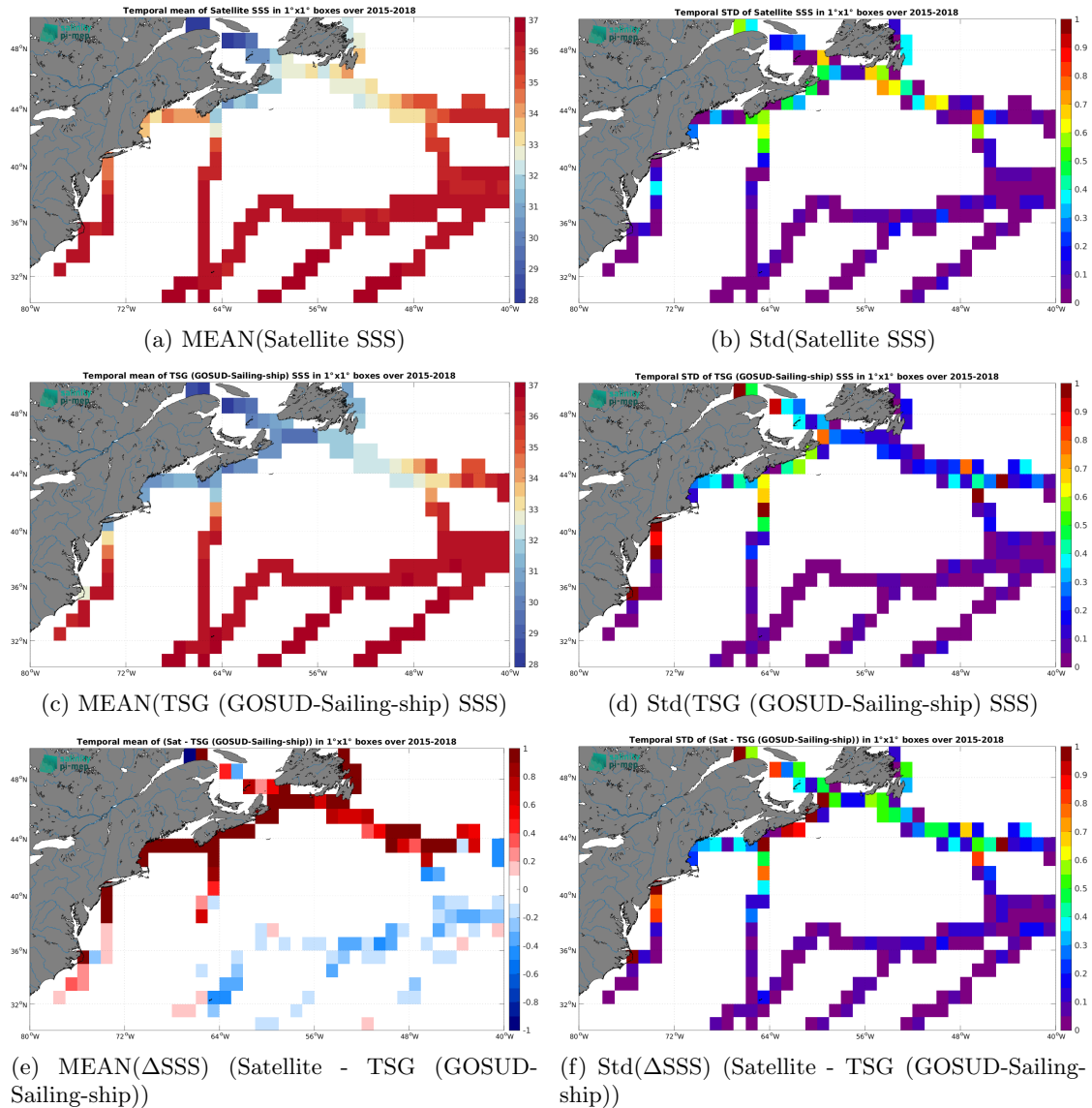
Figure 7: Temporal mean (left) and Std (right) of SSS from SMAP SSS L3 v5.0 - Monthly (JPL) (top), TSG (GOSUD-Sailing-ship) (middle), and of \Delta SSS (Satellite - TSG (GOSUD-Sailing-ship)). Only match-up pairs are used to generate these maps.
