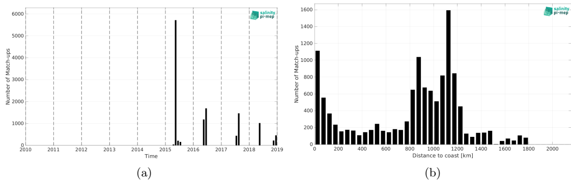
Figure 2: Number of match-ups between TSG (GOSUD-Sailing-ship) and SMAP SSS L3 v5.0 - Monthly (JPL) SSS as a function of time (a) and as function of the distance to coast (b) over the Gulf Stream Pi-MEP region and for the full satellite product period.
