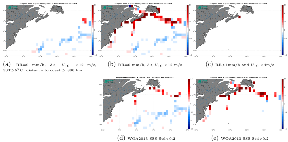
Figure 14: Temporal mean gridded over spatial boxes of size 1^\circ \times 1^\circ of \Delta SSS (SMAP SSS L3 v5.0 - Monthly (JPL) - TSG (GOSUD-Sailing-ship)) for 5 different subdatasets corresponding to:RR=0 mm/h, 3 < U_{10} < 12 m/s, SST >5^\circ\text{C} , distance to coast > 800 km (a), RR=0 mm/h, 3 < U_{10} < 12 m/s (b), RR >1 mm/h and U_{10} < 4 m/s (c), WOA2013 SSS Std <0.2 (d), WOA2013 SSS Std >0.2 (e).
