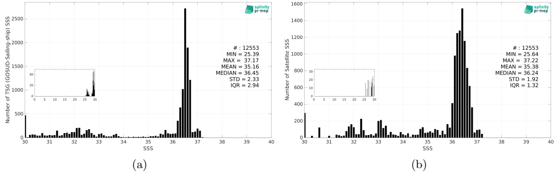
Figure 3: Histograms of SSS from TSG (GOSUD-Sailing-ship) (a) and SMAP SSS L3 v5.0 - Monthly (JPL) (b) considering all match-up pairs per bins of 0.1 over the Gulf Stream Pi-MEP region and for the full satellite product period.
