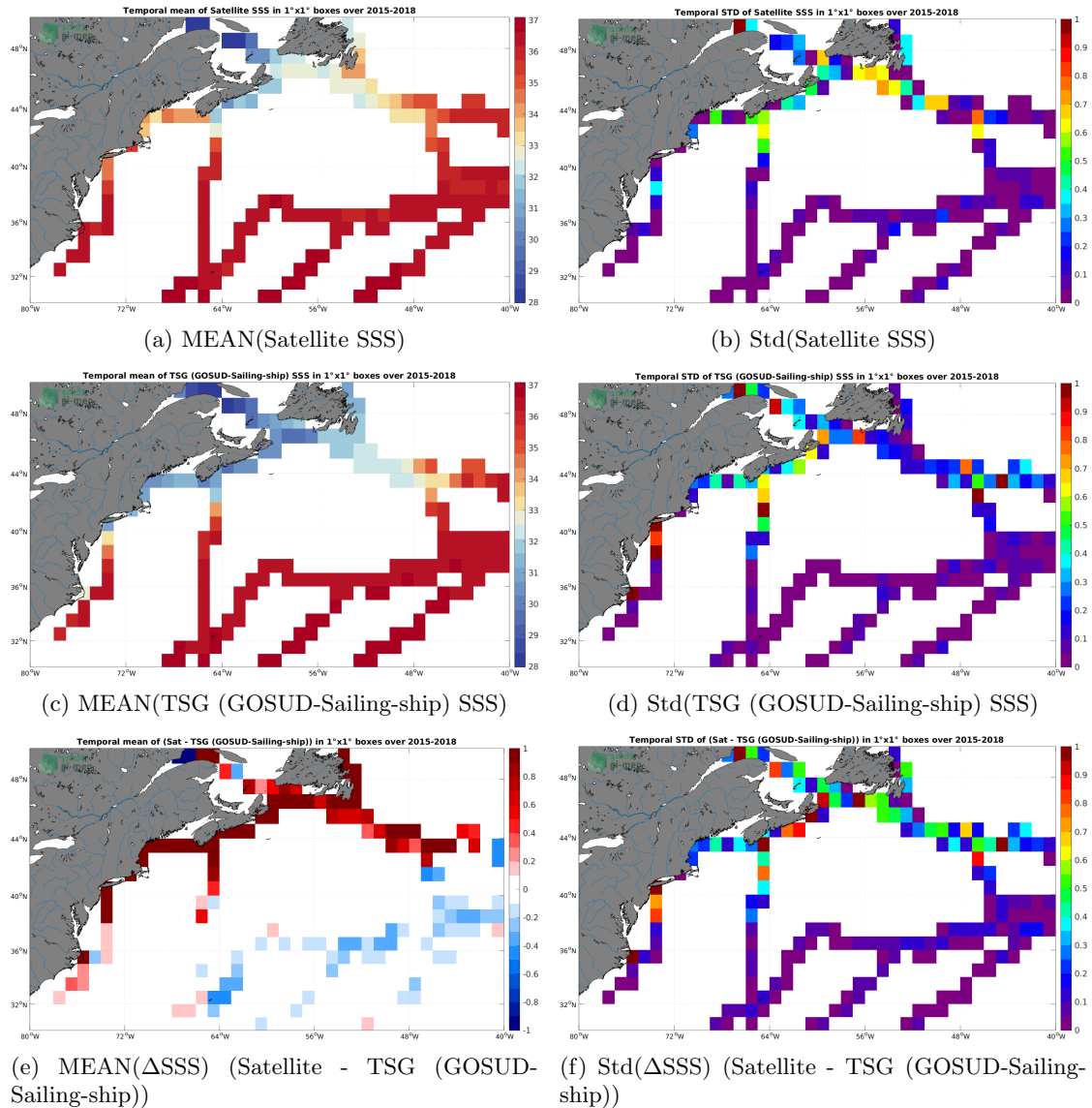
Figure 6: Temporal mean (left) and Std (right) of SSS from SMAP SSS L3 v5.0 - Monthly (JPL) (top), TSG (GOSUD-Sailing-ship) (middle), and of \Delta SSS (Satellite - TSG (GOSUD-Sailing-ship)). Only match-up pairs are used to generate these maps.
