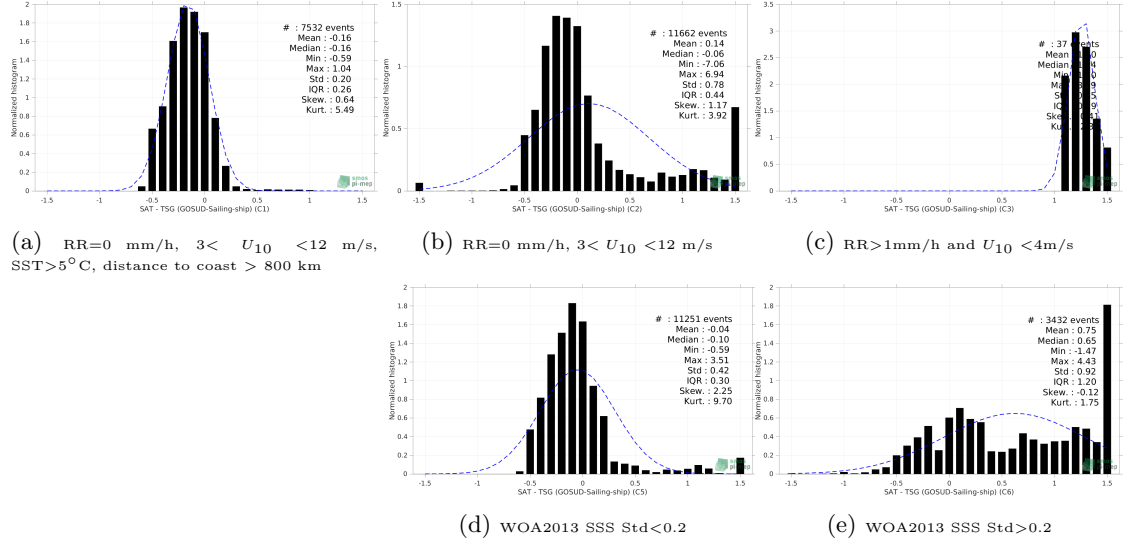
Figure 13: Normalized histogram of \Delta SSS (SMAP SSS L3 v5.0 - Monthly (JPL) - TSG (GOSUD-Sailing-ship)) for 5 different subdatasets corresponding to: RR=0 mm/h, 3 < U_{10} < 12 m/s, SST > 5°C, distance to coast > 800 km (a), RR=0 mm/h, 3 < U_{10} < 12 m/s (b), RR > 1mm/h and U_{10} < 4 m/s (c), WOA2013 SSS Std < 0.2 (d), WOA2013 SSS Std > 0.2 (e).
