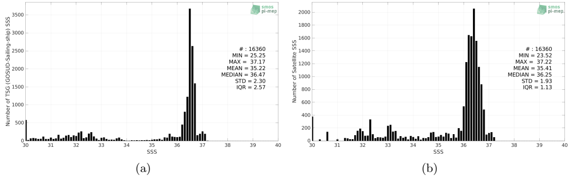
Figure 2: Histograms of SSS from TSG (GOSUD-Sailing-ship) (a) and SMAP SSS L3 v5.0 - Monthly (JPL) (b) considering all match-up pairs per bins of 0.1 over the Gulf Stream Pi-MEP region and for the full satellite product period.
