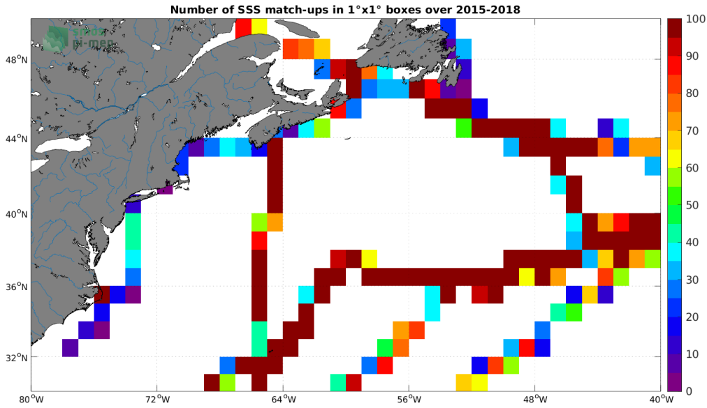
Figure 4: Number of SSS match-ups between TSG (GOSUD-Sailing-ship) SSS and the SMAP SSS L3 v5.0 - Monthly (JPL) SSS product for the Gulf Stream Pi-MEP region over 1^\circ \times 1^\circ boxes and for the full satellite product period.
