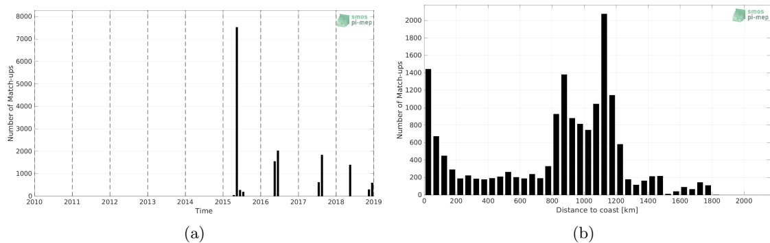
Figure 1: Number of match-ups between TSG (GOSUD-Sailing-ship) and SMAP SSS L3 v5.0 - Monthly (JPL) SSS as a function of time (a) and as function of the distance to coast (b) over the Gulf Stream Pi-MEP region and for the full satellite product period.
