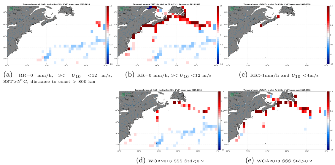
Figure 12: Temporal mean gridded over spatial boxes of size 1^\circ \times 1^\circ of \Delta SSS (SMAP SSS L3 v5.0 - Monthly (JPL) - TSG (GOSUD-Sailing-ship)) for 5 different subdatasets corresponding to:RR=0 mm/h, 3 < U_{10} < 12 m/s, SST>5°C, distance to coast > 800 km (a), RR=0 mm/h, 3 < U_{10} < 12 m/s (b), RR>1mm/h and U_{10} < 4 m/s (c), WOA2013 SSS Std<0.2 (d), WOA2013 SSS Std>0.2 (e).
