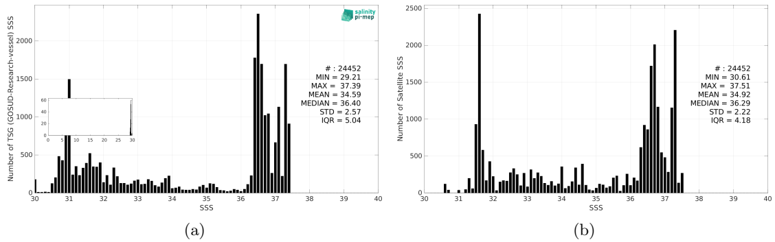
Figure 3: Histograms of SSS from TSG (GOSUD-Research-vessel) (a) and SMAP SSS L3 v5.0 - Monthly (JPL) (b) considering all match-up pairs per bins of 0.1 over the Gulf Stream Pi-MEP region and for the full satellite product period.
