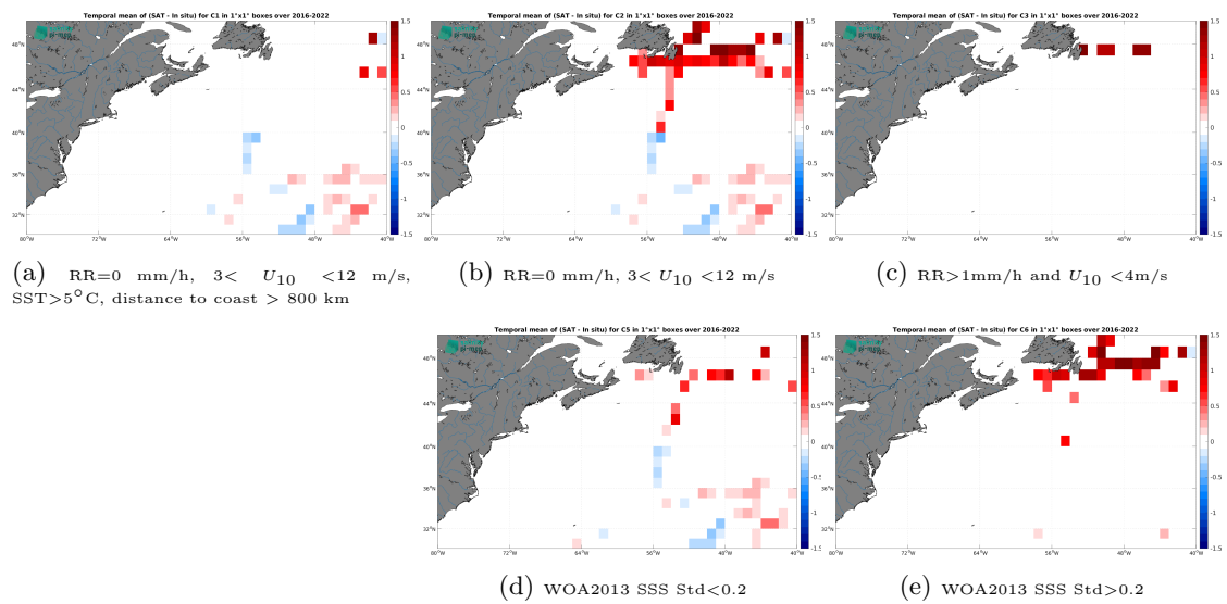
Figure 14: Temporal mean gridded over spatial boxes of size 1^\circ \times 1^\circ of \Delta SSS (SMAP SSS L3 v5.0 - Monthly (JPL) - TSG (GOSUD-Research-vessel)) for 5 different subdatasets corresponding to: RR=0 mm/h, 3 < U_{10} < 12 m/s, SST > 5°C, distance to coast > 800 km (a), RR=0 mm/h, 3 < U_{10} < 12 m/s (b), RR > 1mm/h and U_{10} < 4 m/s (c), WOA2013 SSS Std < 0.2 (d), WOA2013 SSS Std > 0.2 (e).
