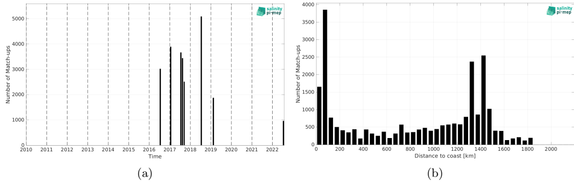
Figure 2: Number of match-ups between TSG (GOSUD-Research-vessel) and SMAP SSS L3 v5.0 - Monthly (JPL) SSS as a function of time (a) and as function of the distance to coast (b) over the Gulf Stream Pi-MEP region and for the full satellite product period.
