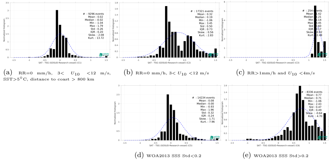
Figure 15: Normalized histogram of \Delta\text{SSS} (SMAP SSS L3 v5.0 - Monthly (JPL) - TSG (GOSUD-Research-vessel)) for 5 different subdatasets corresponding to: RR=0 mm/h, 3 < U_{10} < 12 m/s, SST>5°C, distance to coast > 800 km (a), RR=0 mm/h, 3 < U_{10} < 12 m/s (b), RR>1mm/h and U_{10} < 4 m/s (c), WOA2013 SSS Std<0.2 (d), WOA2013 SSS Std>0.2 (e).
