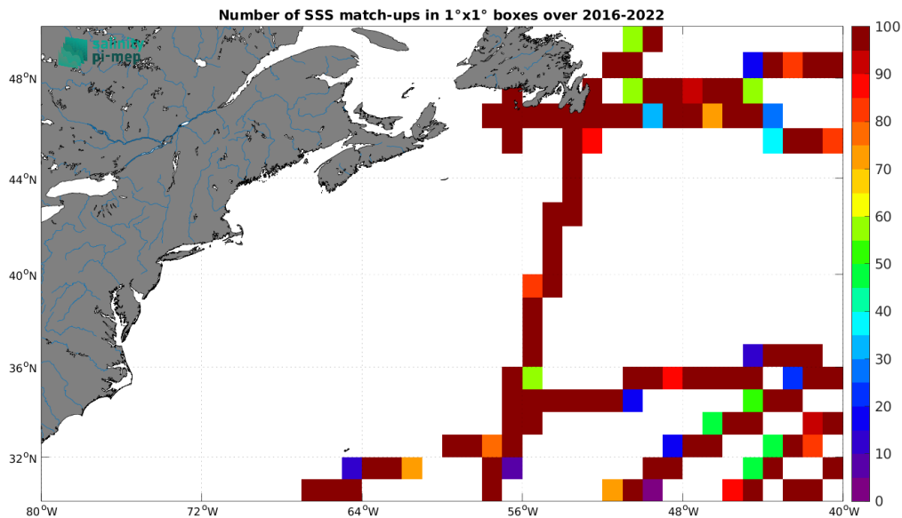
Figure 5: Number of SSS match-ups between TSG (GOSUD-Research-vessel) SSS and the SMAP SSS L3 v5.0 - Monthly (JPL) SSS product for the Gulf Stream Pi-MEP region over 1^\circ \times 1^\circ boxes and for the full satellite product period.
