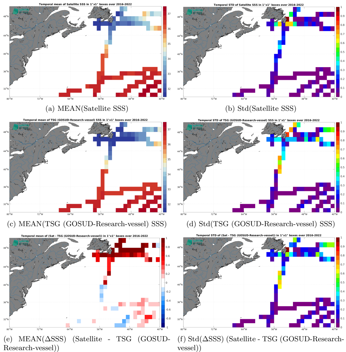
Figure 7: Temporal mean (left) and Std (right) of SSS from SMAP SSS L3 v5.0 - Monthly (JPL) (top), TSG (GOSUD-Research-vessel) (middle), and of \Delta SSS (Satellite - TSG (GOSUD-Research-vessel)). Only match-up pairs are used to generate these maps.
