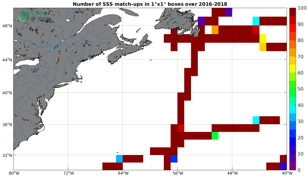
Figure 4: Number of SSS match-ups between TSG (GOSUD-Research-vessel) SSS and the SMAP SSS L3 v5.0 - Monthly (JPL) SSS product for the Gulf Stream Pi-MEP region over 1°x1° boxes and for the full satellite product period.
