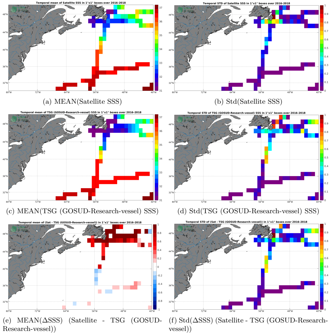
Figure 6: Temporal mean (left) and Std (right) of SSS from SMAP SSS L3 v5.0 - Monthly (JPL) (top), TSG (GOSUD-Research-vessel) (middle), and of \Delta\text{SSS} (Satellite - TSG (GOSUD-Research-vessel)). Only match-up pairs are used to generate these maps.
