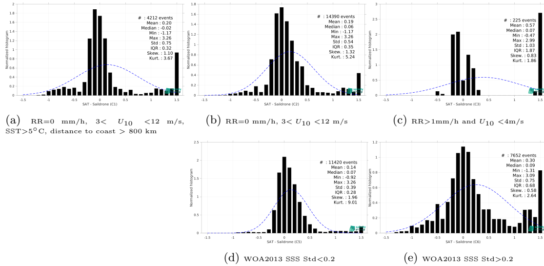
Figure 13: Normalized histogram of \Delta\text{SSS} (SMAP SSS L3 v5.0 - Monthly (JPL) - Saildrone) for 5 different subdatasets corresponding to: RR=0 mm/h, 3 < U_{10} < 12 m/s, SST>5°C, distance to coast > 800 km (a), RR=0 mm/h, 3 < U_{10} < 12 m/s (b), RR>1mm/h and U_{10} < 4 m/s (c), WOA2013 SSS Std<0.2 (d), WOA2013 SSS Std>0.2 (e).
