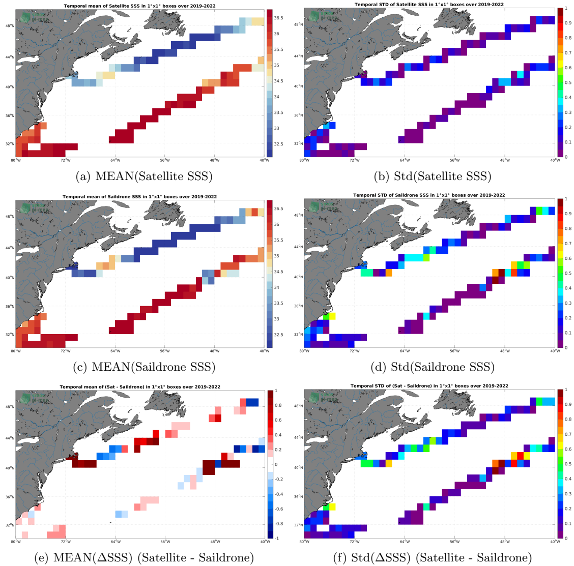
Figure 6: Temporal mean (left) and Std (right) of SSS from SMAP SSS L3 v5.0 - Monthly (JPL) (top), Saildrone (middle), and of \Delta SSS (Satellite - Saildrone). Only match-up pairs are used to generate these maps.
