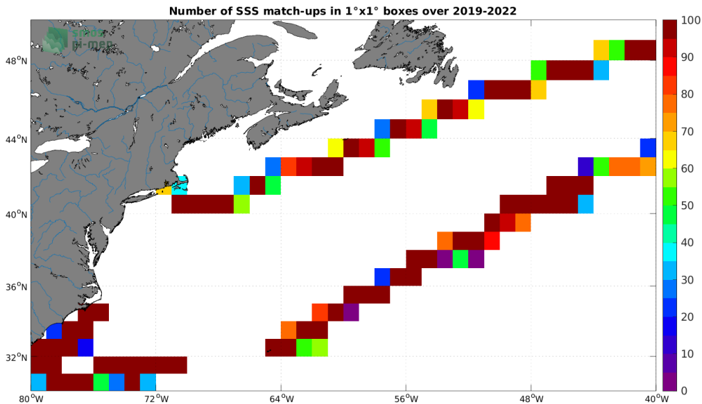
Figure 4: Number of SSS match-ups between Saildrone SSS and the SMAP SSS L3 v5.0 - Monthly (JPL) SSS product for the Gulf Stream Pi-MEP region over 1^\circ \times 1^\circ boxes and for the full satellite product period.
