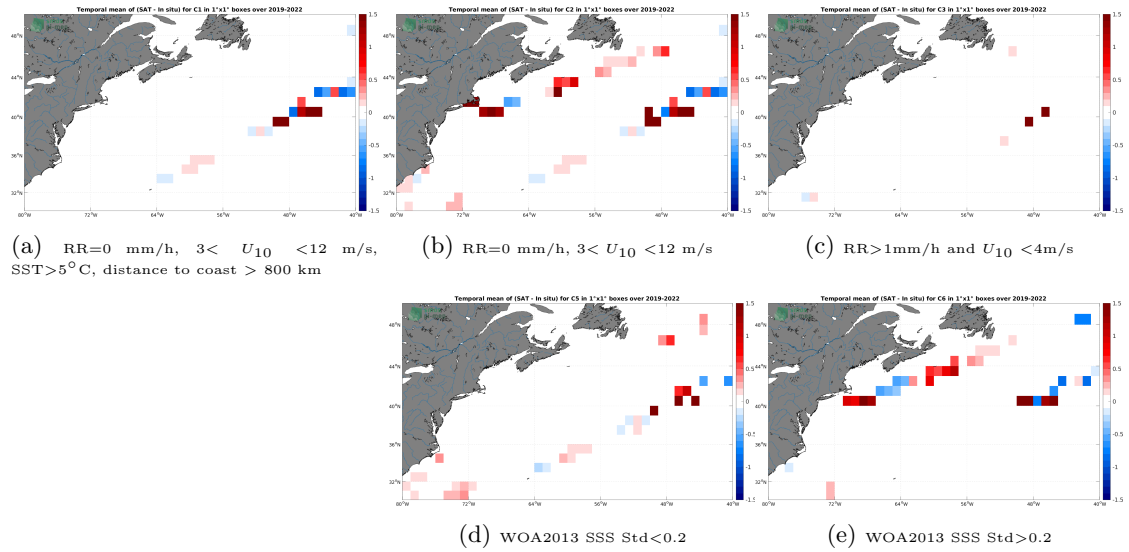
Figure 12: Temporal mean gridded over spatial boxes of size 1^\circ \times 1^\circ of \Delta SSS (SMAP SSS L3 v5.0 - Monthly (JPL) - Sairdrone) for 5 different subdatasets corresponding to:RR=0 mm/h, 3 < U_{10} < 12 m/s, SST >5^\circ C, distance to coast > 800 km (a), RR=0 mm/h, 3 < U_{10} < 12 m/s (b), RR >1 mm/h and U_{10} < 4 m/s (c), WOA2013 SSS Std <0.2 (d), WOA2013 SSS Std >0.2 (e).
