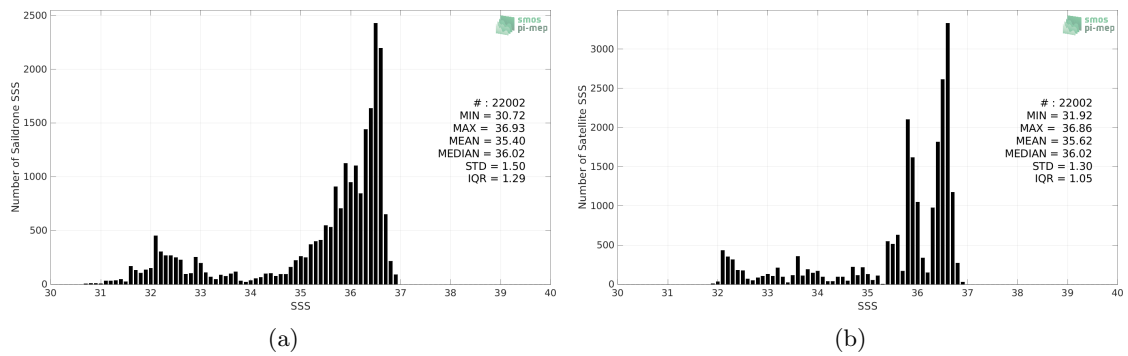
Figure 2: Histograms of SSS from Saildrone (a) and SMAP SSS L3 v5.0 - Monthly (JPL) (b) considering all match-up pairs per bins of 0.1 over the Gulf Stream Pi-MEP region and for the full satellite product period.
