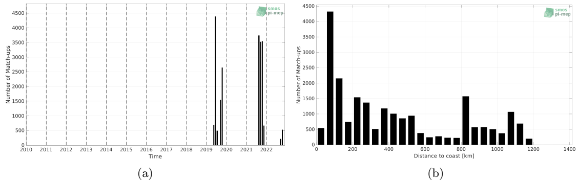
Figure 1: Number of match-ups between Saildrone and SMAP SSS L3 v5.0 - Monthly (JPL) SSS as a function of time (a) and as function of the distance to coast (b) over the Gulf Stream Pi-MEP region and for the full satellite product period.
