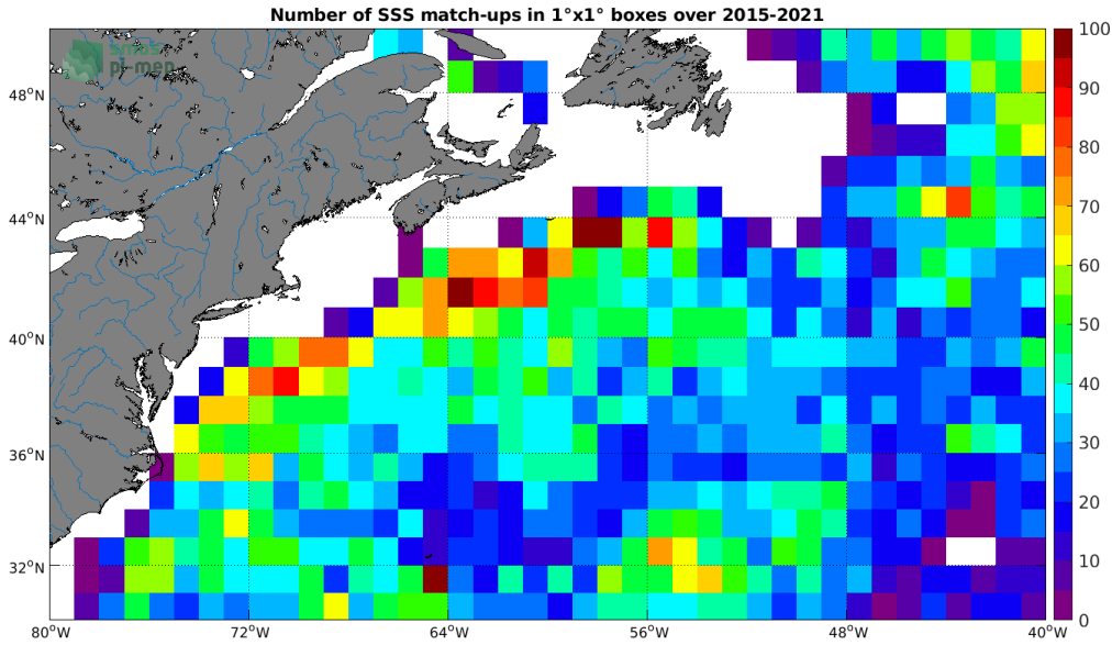
Figure 4: Number of SSS match-ups between Argo SSS and the SMAP SSS L3 v5.0 - Monthly (JPL) SSS product for the Gulf Stream Pi-MEP region over 1°x1° boxes and for the full satellite product period.
