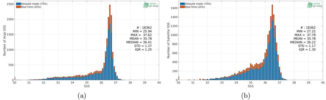
Figure 2: Histograms of SSS from Argo (a) and SMAP SSS L3 v5.0 - Monthly (JPL) (b) considering all match-up pairs per bins of 0.1 over the Gulf Stream Pi-MEP region and for the full satellite product period.
