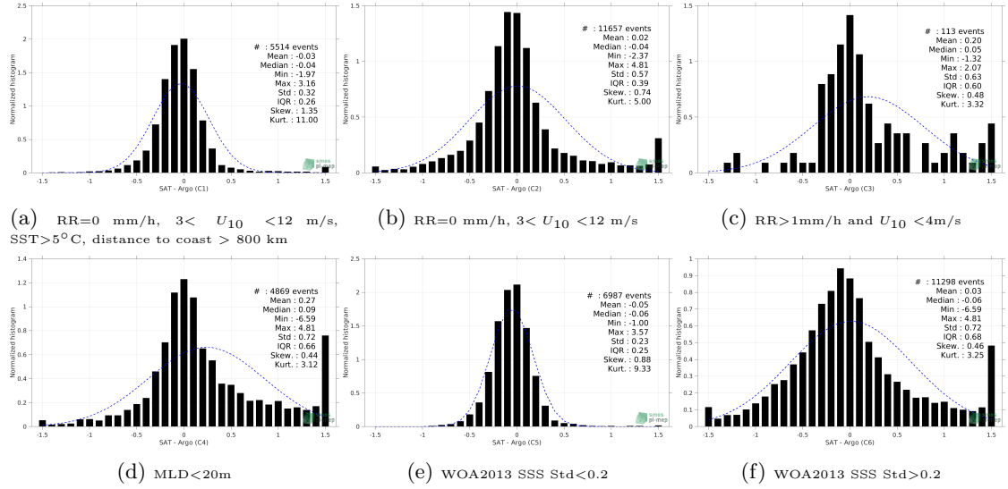
Figure 13: Normalized histogram of \Delta\text{SSS} (SMAP SSS L3 v5.0 - Monthly (JPL) - Argo) for 6 different subdatasets corresponding to: RR=0 mm/h, 3 < U_{10} < 12 m/s, SST>5°C, distance to coast > 800 km (a), RR=0 mm/h, 3 < U_{10} < 12 m/s (b), RR>1mm/h and U_{10} < 4 m/s (c), MLD<20m (d), WOA2013 SSS Std<0.2 (e), WOA2013 SSS Std>0.2 (f).
