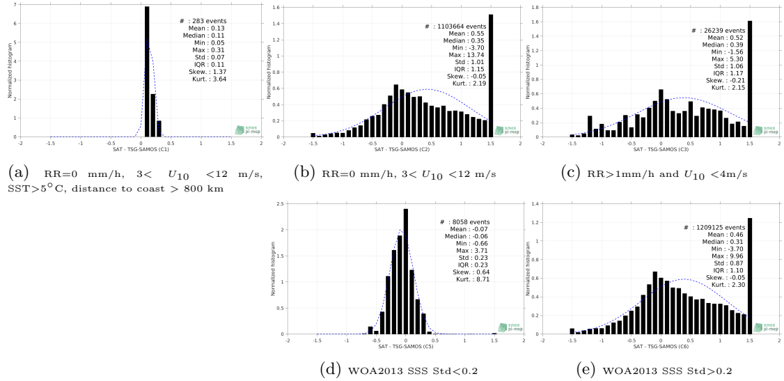
Figure 13: Normalized histogram of \Delta SSS (SMAP-L3-JPL-V4.3-8DAY-RUNNING-60KM - TSG-SAMOS) for 5 different subdatasets corresponding to: RR=0 mm/h, 3 < U_{10} < 12 m/s, SST > 5°C, distance to coast > 800 km (a), RR=0 mm/h, 3 < U_{10} < 12 m/s (b), RR > 1mm/h and U_{10} < 4 m/s (c), WOA2013 SSS Std < 0.2 (d), WOA2013 SSS Std > 0.2 (e).
