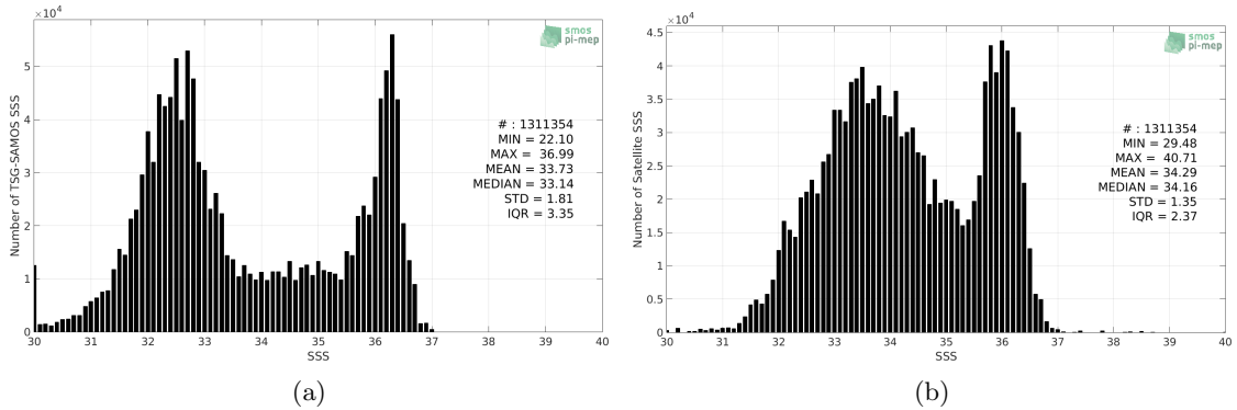
Figure 2: Histograms of SSS from TSG-SAMOS (a) and SMAP-L3-JPL-V4.3-8DAY-RUNNING-60KM (b) considering all match-up pairs per bins of 0.1 over the Gulf Stream Pi-MEP region and for the full satellite product period.
