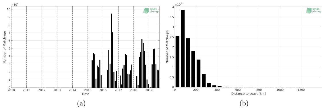
Figure 1: Number of match-ups between TSG-SAMOS and SMAP-L3-JPL-V4.3-8DAY-RUNNING-60KM SSS as a function of time (a) and as function of the distance to coast (b) over the Gulf Stream Pi-MEP region and for the full satellite product period.
