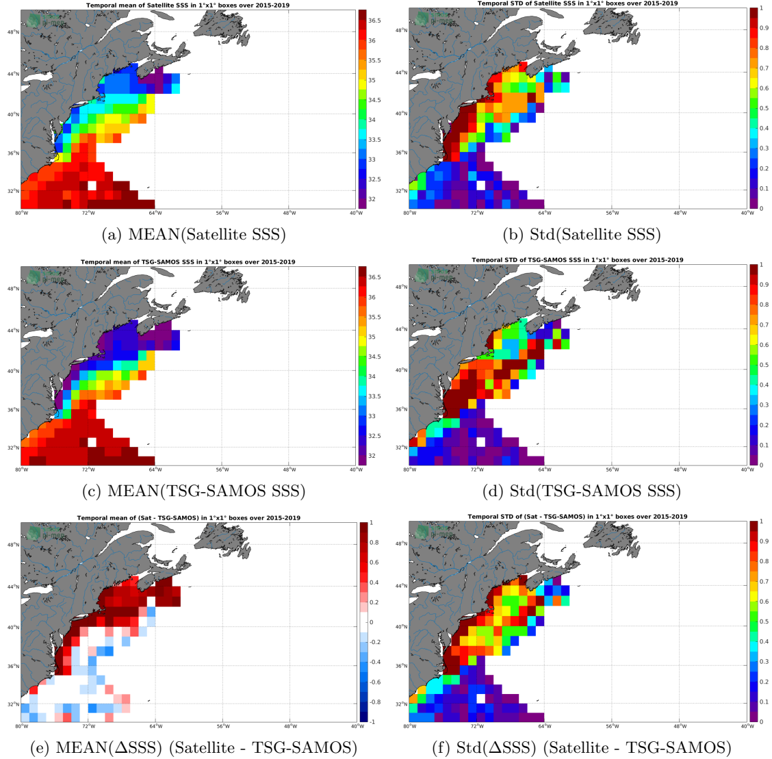
Figure 6: Temporal mean (left) and Std (right) of SSS from SMAP-L3-JPL-V4.3-8DAY-RUNNING-60KM (top), TSG-SAMOS (middle), and of \Delta SSS (Satellite - TSG-SAMOS). Only match-up pairs are used to generate these maps.
