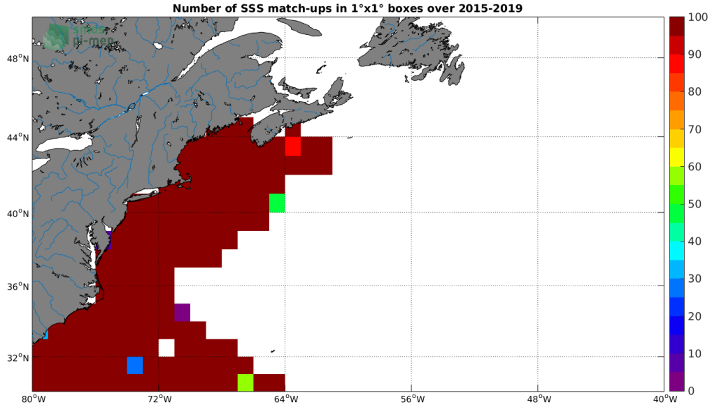
Figure 4: Number of SSS match-ups between TSG-SAMOS SSS and the SMAP-L3-JPL-V4.3-8DAY-RUNNING-60KM SSS product for the Gulf Stream Pi-MEP region over 1°x1° boxes and for the full satellite product period.
