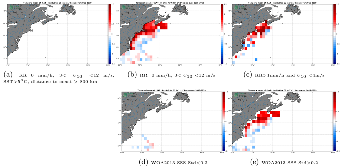
Figure 12: Temporal mean gridded over spatial boxes of size 1^\circ \times 1^\circ of \Delta SSS (SMAP-L3-JPL-V4.3-8DAY-RUNNING-60KM - TSG-SAMOS) for 5 different subdatasets corresponding to:RR=0 mm/h, 3 < U_{10} < 12 m/s, SST >5^\circ C, distance to coast > 800 km (a), RR=0 mm/h, 3 < U_{10} < 12 m/s (b), RR >1 mm/h and U_{10} < 4 m/s (c), WOA2013 SSS Std <0.2 (d), WOA2013 SSS Std >0.2 (e).
