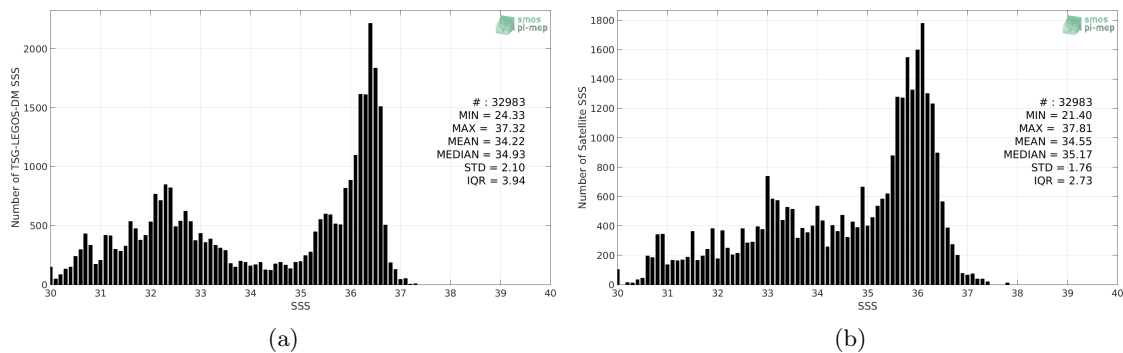
Figure 2: Histograms of SSS from TSG-LEGOS-DM (a) and SMAP-L3-JPL-V4.3-8DAY-RUNNING-60KM (b) considering all match-up pairs per bins of 0.1 over the Gulf Stream Pi-MEP region and for the full satellite product period.
