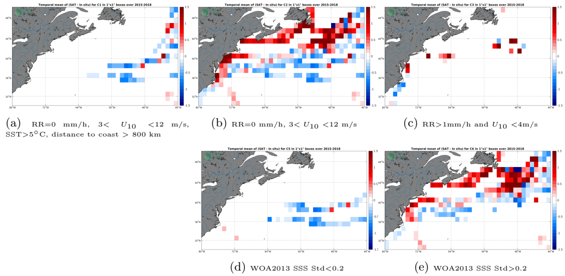
Figure 12: Temporal mean gridded over spatial boxes of size 1^\circ \times 1^\circ of \Delta SSS (SMAP-L3-JPL-V4.3-8DAY-RUNNING-60KM - TSG-LEGOS-DM) for 5 different subdatasets corresponding to:RR=0 mm/h, 3 < U_{10} < 12 m/s, SST >5^\circ C, distance to coast > 800 km (a), RR=0 mm/h, 3 < U_{10} < 12 m/s (b), RR >1 mm/h and U_{10} < 4 m/s (c), WOA2013 SSS Std <0.2 (d), WOA2013 SSS Std >0.2 (e).
