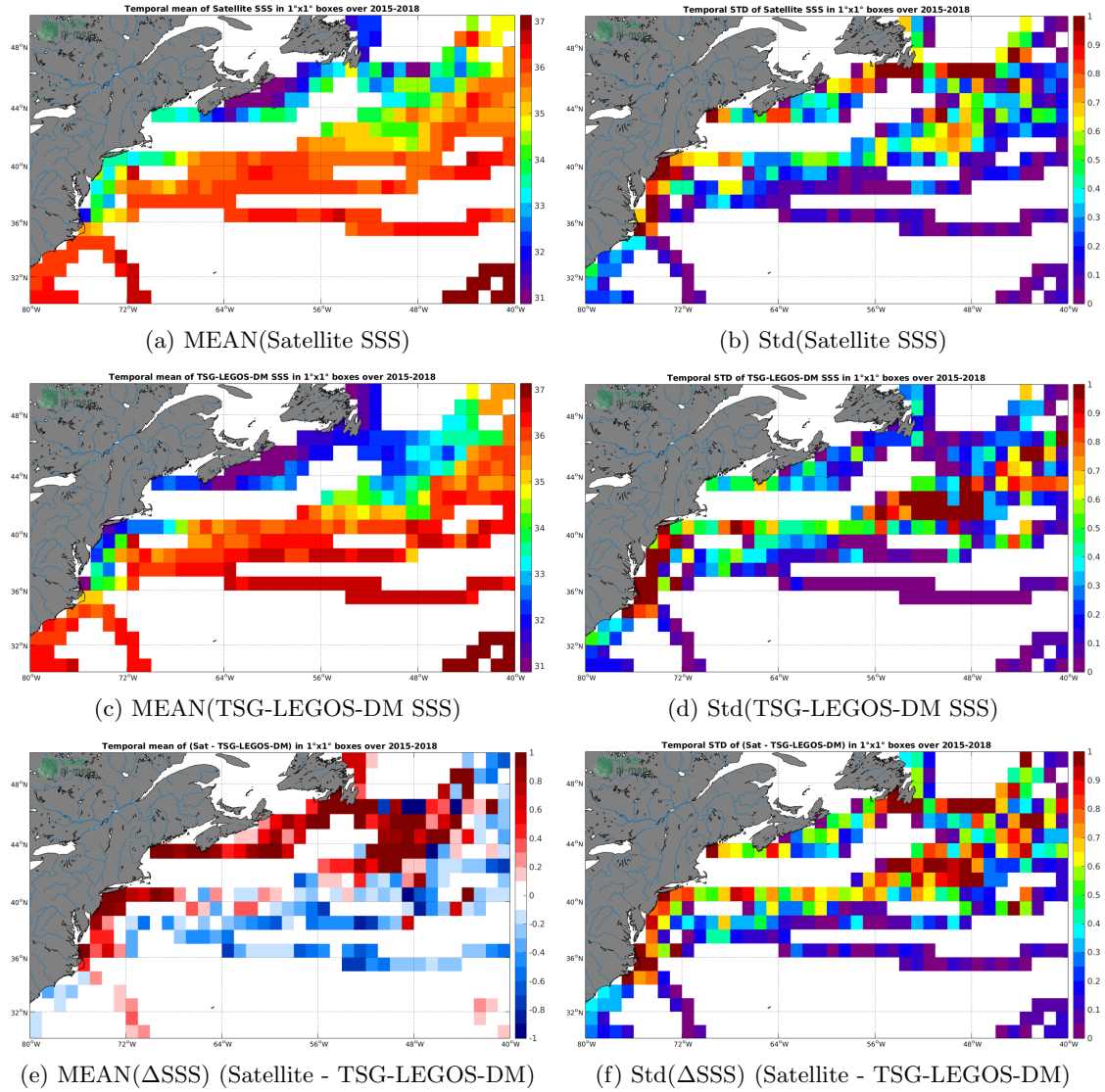
Figure 6: Temporal mean (left) and Std (right) of SSS from SMAP-L3-JPL-V4.3-8DAY-RUNNING-60KM (top), TSG-LEGOS-DM (middle), and of \Delta SSS (Satellite - TSG-LEGOS-DM). Only match-up pairs are used to generate these maps.
