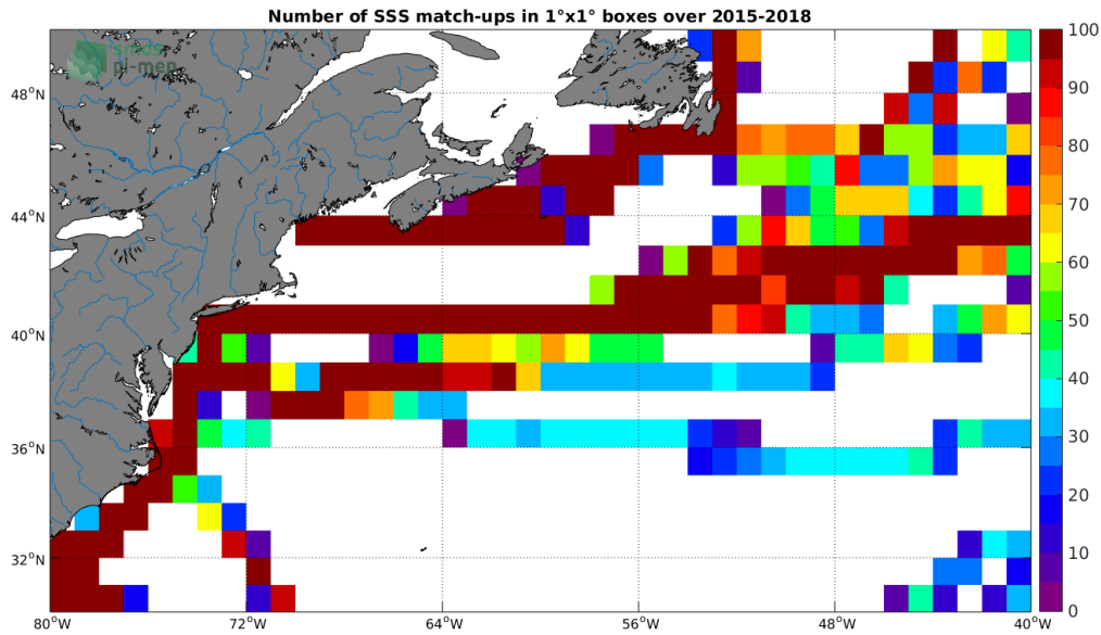
Figure 4: Number of SSS match-ups between TSG-LEGOS-DM SSS and the SMAP-L3-JPL-V4.3-8DAY-RUNNING-60KM SSS product for the Gulf Stream Pi-MEP region over 1°x1° boxes and for the full satellite product period.
