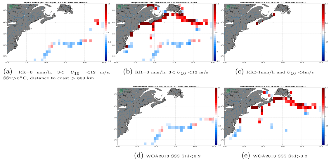
Figure 12: Temporal mean gridded over spatial boxes of size 1^{\circ}\times 1^{\circ} of \Delta SSS (SMAP-L3-JPL-V4.3-8DAY-RUNNING-60KM - TSG-GOSUD-Sailing-ship) for 5 different subdatasets corresponding to:RR=0 mm/h, 3 < U_{10} < 12 m/s, SST >5^{\circ}\text{C} , distance to coast > 800 km (a), RR=0 mm/h, 3 < U_{10} < 12 m/s (b), RR >1 mm/h and U_{10} < 4 m/s (c), WOA2013 SSS Std <0.2 (d), WOA2013 SSS Std >0.2 (e).
