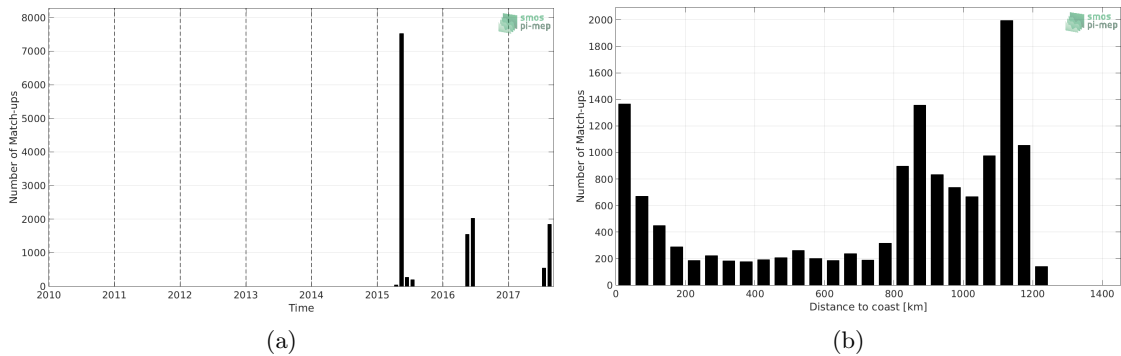
Figure 1: Number of match-ups between TSG-GOSUD-Sailing-ship and SMAP-L3-JPL-V4.3-8DAY-RUNNING-60KM SSS as a function of time (a) and as function of the distance to coast (b) over the Gulf Stream Pi-MEP region and for the full satellite product period.
