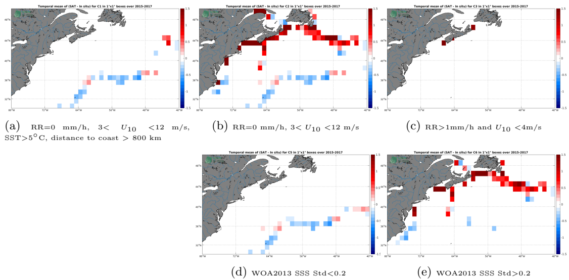
Figure 12: Temporal mean gridded over spatial boxes of size 1^\circ \times 1^\circ of \Delta SSS (SMAP-L3-JPL-V4.3-8DAY-RUNNING-60KM - TSG-GOSUD-Sailing-ship) for 5 different subdatasets corresponding to: RR=0 mm/h, 3 < U_{10} < 12 m/s, SST>5°C, distance to coast > 800 km (a), RR=0 mm/h, 3 < U_{10} < 12 m/s (b), RR>1mm/h and U_{10} < 4 m/s (c), WOA2013 SSS Std<0.2 (d), WOA2013 SSS Std>0.2 (e).
