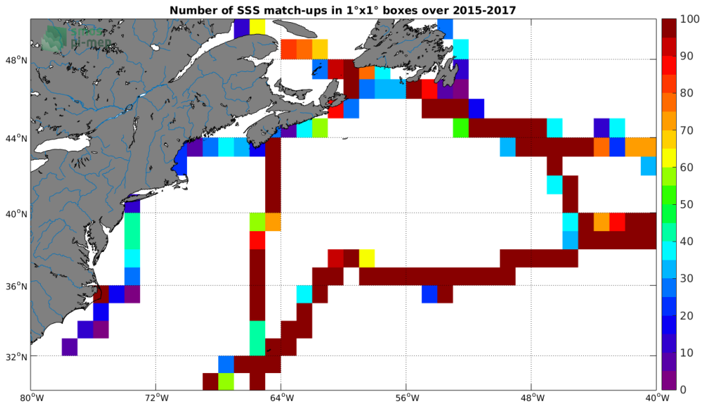
Figure 4: Number of SSS match-ups between TSG-GOSUD-Sailing-ship SSS and the SMAP-L3-JPL-V4.3-8DAY-RUNNING-60KM SSS product for the Gulf Stream Pi-MEP region over 1°x1° boxes and for the full satellite product period.
