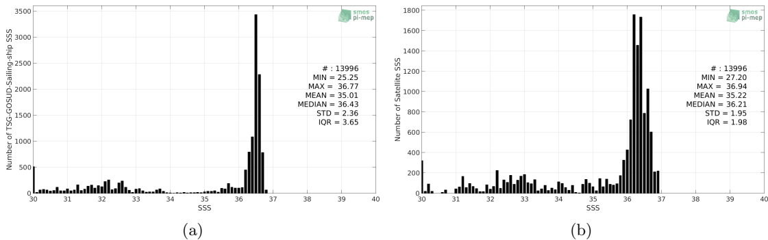
Figure 2: Histograms of SSS from TSG-GOSUD-Sailing-ship (a) and SMAP-L3-JPL-V4.3-8DAY-RUNNING-60KM (b) considering all match-up pairs per bins of 0.1 over the Gulf Stream Pi-MEP region and for the full satellite product period.
