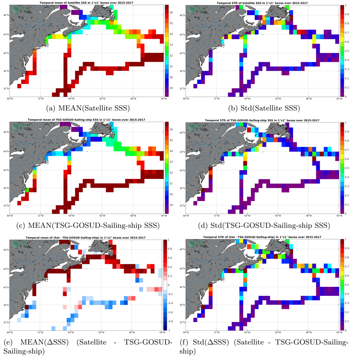
Figure 6: Temporal mean (left) and Std (right) of SSS from SMAP-L3-JPL-V4.3-8DAY-RUNNING-60KM (top), TSG-GOSUD-Sailing-ship (middle), and of \Delta SSS (Satellite - TSG-GOSUD-Sailing-ship). Only match-up pairs are used to generate these maps.
