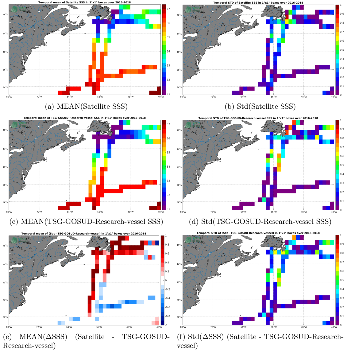
Figure 6: Temporal mean (left) and Std (right) of SSS from SMAP-L3-JPL-V4.3-8DAY-RUNNING-60KM (top), TSG-GOSUD-Research-vessel (middle), and of \Delta SSS (Satellite - TSG-GOSUD-Research-vessel). Only match-up pairs are used to generate these maps.
