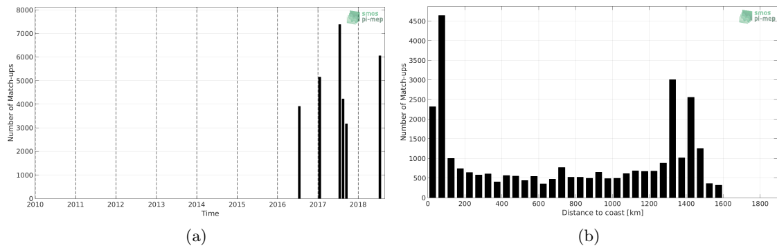
Figure 1: Number of match-ups between TSG-GOSUD-Research-vessel and SMAP-L3-JPL-V4.3-8DAY-RUNNING-60KM SSS as a function of time (a) and as function of the distance to coast (b) over the Gulf Stream Pi-MEP region and for the full satellite product period.
