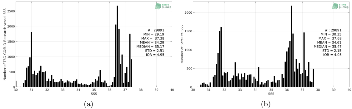
Figure 2: Histograms of SSS from TSG-GOSUD-Research-vessel (a) and SMAP-L3-JPL-V4.3-8DAY-RUNNING-60KM (b) considering all match-up pairs per bins of 0.1 over the Gulf Stream Pi-MEP region and for the full satellite product period.
