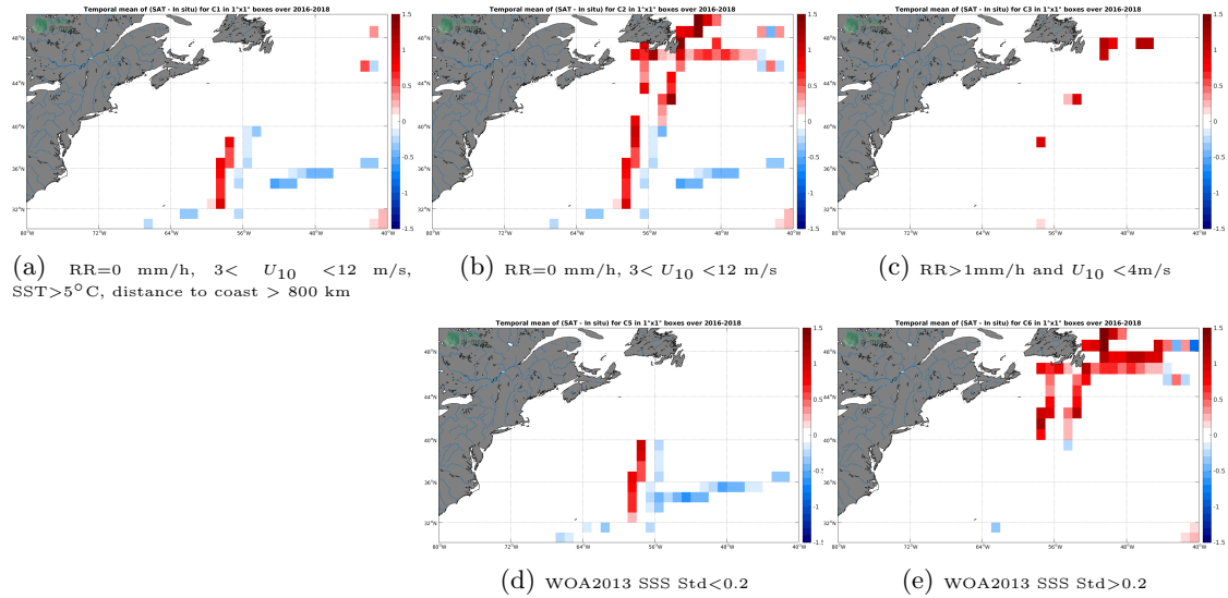
Figure 12: Temporal mean gridded over spatial boxes of size 1^\circ \times 1^\circ of \Delta SSS (SMAP-L3-JPL-V4.3-8DAY-RUNNING-60KM - TSG-GOSUD-Research-vessel) for 5 different subdatasets corresponding to: RR=0 mm/h, 3 < U_{10} < 12 m/s, SST > 5^\circ\text{C} , distance to coast > 800 km (a), RR=0 mm/h, 3 < U_{10} < 12 m/s (b), RR > 1 mm/h and U_{10} < 4 m/s (c), WOA2013 SSS Std < 0.2 (d), WOA2013 SSS Std > 0.2 (e).
