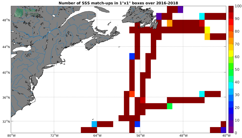
Figure 4: Number of SSS match-ups between TSG-GOSUD-Research-vessel SSS and the SMAP-L3-JPL-V4.3-8DAY-RUNNING-60KM SSS product for the Gulf Stream Pi-MEP region over 1^\circ \times 1^\circ boxes and for the full satellite product period.
