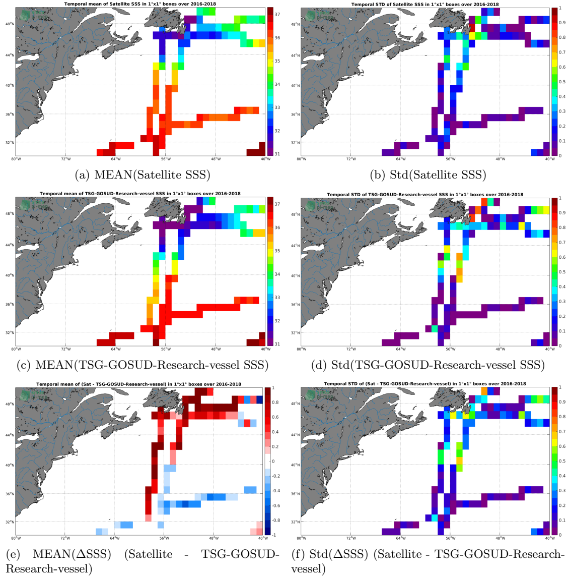
Figure 6: Temporal mean (left) and Std (right) of SSS from SMAP-L3-JPL-V4.3-8DAY-RUNNING-60KM (top), TSG-GOSUD-Research-vessel (middle), and of \Delta\text{SSS} (Satellite - TSG-GOSUD-Research-vessel). Only match-up pairs are used to generate these maps.
