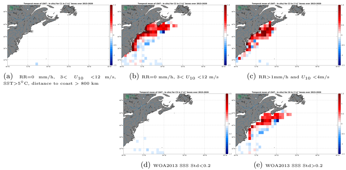
Figure 12: Temporal mean gridded over spatial boxes of size 1^\circ \times 1^\circ of \Delta SSS (SMAP-L3-JPL-V4.3-MONTHLY-60KM - TSG-SAMOS) for 5 different subdatasets corresponding to:RR=0 mm/h, 3 < U_{10} < 12 m/s, SST >5^\circ C, distance to coast > 800 km (a), RR=0 mm/h, 3 < U_{10} < 12 m/s (b), RR >1 mm/h and U_{10} < 4 m/s (c), WOA2013 SSS Std <0.2 (d), WOA2013 SSS Std >0.2 (e).
