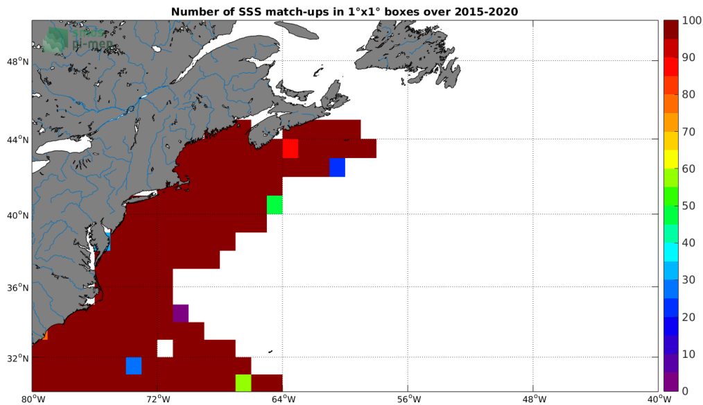
Figure 4: Number of SSS match-ups between TSG-SAMOS SSS and the SMAP-L3-JPL-V4.3-MONTHLY-60KM SSS product for the Gulf Stream Pi-MEP region over 1^\circ \times 1^\circ boxes and for the full satellite product period.
