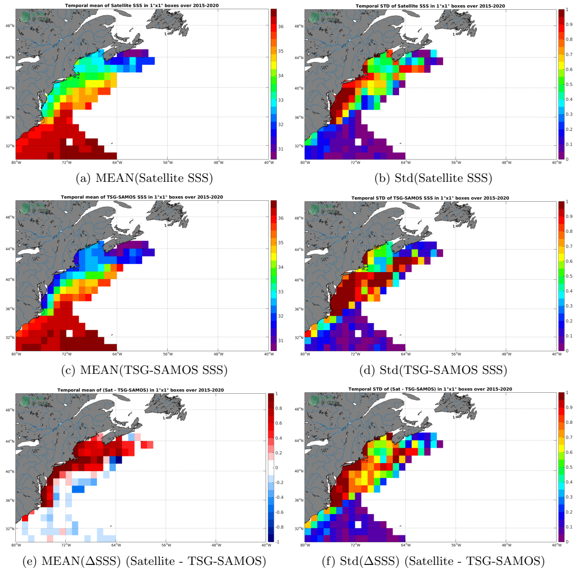
Figure 6: Temporal mean (left) and Std (right) of SSS from SMAP-L3-JPL-V4.3-MONTHLY-60KM (top), TSG-SAMOS (middle), and of \Delta SSS (Satellite - TSG-SAMOS). Only match-up pairs are used to generate these maps.
