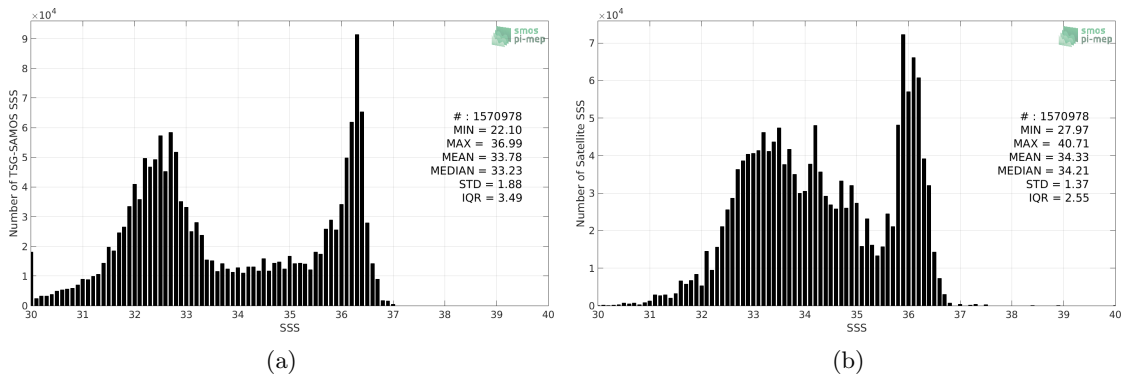
Figure 2: Histograms of SSS from TSG-SAMOS (a) and SMAP-L3-JPL-V4.3-MONTHLY-60KM (b) considering all match-up pairs per bins of 0.1 over the Gulf Stream Pi-MEP region and for the full satellite product period.
