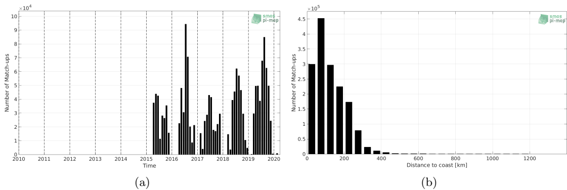
Figure 1: Number of match-ups between TSG-SAMOS and SMAP-L3-JPL-V4.3-MONTHLY-60KM SSS as a function of time (a) and as function of the distance to coast (b) over the Gulf Stream Pi-MEP region and for the full satellite product period.
