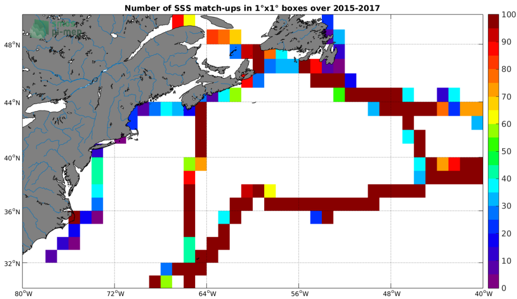
Figure 4: Number of SSS match-ups between TSG-GOSUD-Sailing-ship SSS and the SMAP-L3-JPL-V4.3-MONTHLY-60KM SSS product for the Gulf Stream Pi-MEP region over 1^\circ \times 1^\circ boxes and for the full satellite product period.
