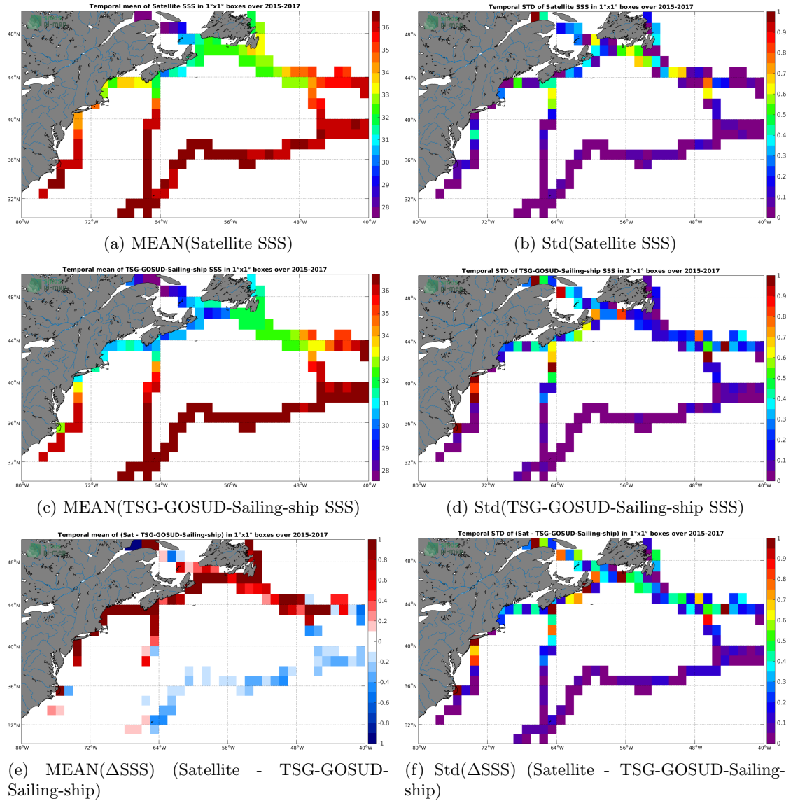
Figure 6: Temporal mean (left) and Std (right) of SSS from SMAP-L3-JPL-V4.3-MONTHLY-60KM (top), TSG-GOSUD-Sailing-ship (middle), and of \Delta SSS (Satellite - TSG-GOSUD-Sailing-ship). Only match-up pairs are used to generate these maps.
