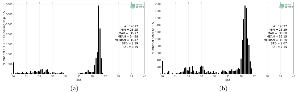
Figure 2: Histograms of SSS from TSG-GOSUD-Sailing-ship (a) and SMAP-L3-JPL-V4.3-MONTHLY-60KM (b) considering all match-up pairs per bins of 0.1 over the Gulf Stream Pi-MEP region and for the full satellite product period.
