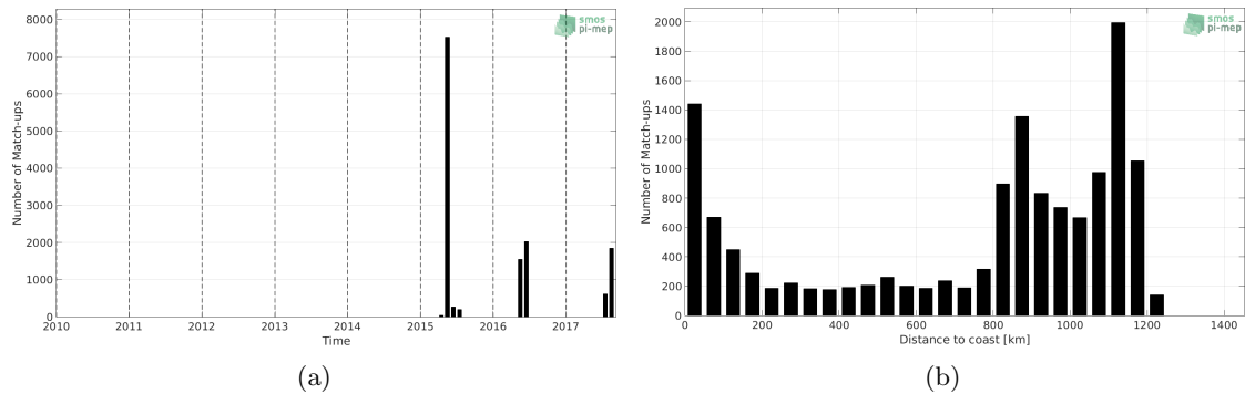
Figure 1: Number of match-ups between TSG-GOSUD-Sailing-ship and SMAP-L3-JPL-V4.3-MONTHLY-60KM SSS as a function of time (a) and as function of the distance to coast (b) over the Gulf Stream Pi-MEP region and for the full satellite product period.
