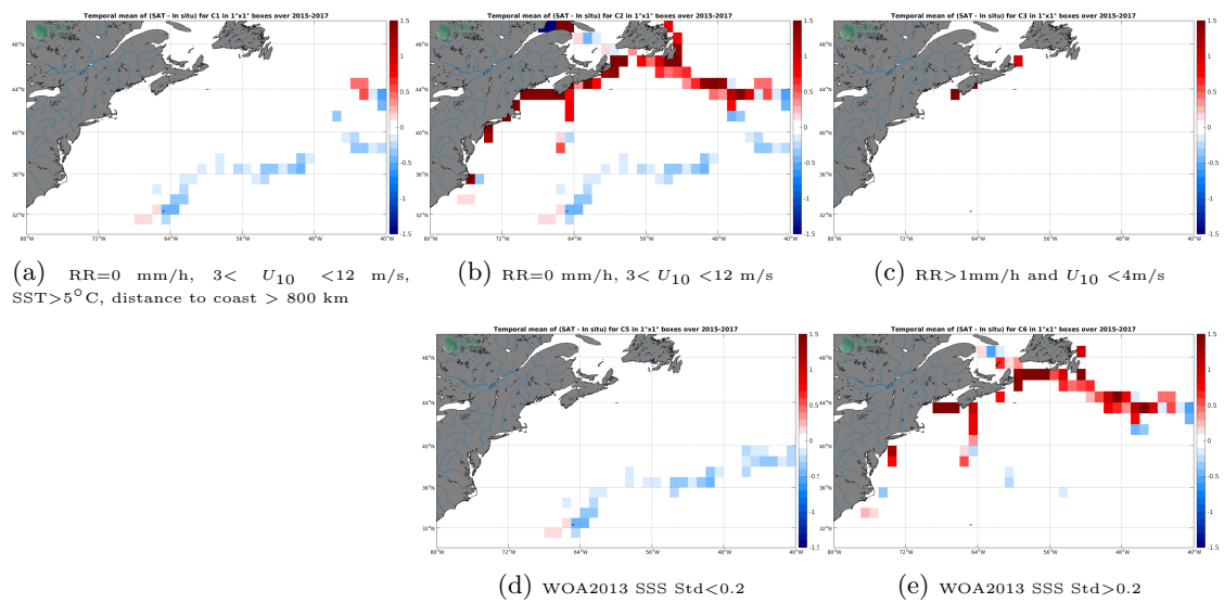
Figure 12: Temporal mean gridded over spatial boxes of size 1^\circ \times 1^\circ of \Delta SSS (SMAP-L3-JPL-V4.3-MONTHLY-60KM - TSG-GOSUD-Sailing-ship) for 5 different subdatasets corresponding to: RR=0 mm/h, 3 < U_{10} < 12 m/s, SST > 5°C, distance to coast > 800 km (a), RR=0 mm/h, 3 < U_{10} < 12 m/s (b), RR > 1mm/h and U_{10} < 4 m/s (c), WOA2013 SSS Std < 0.2 (d), WOA2013 SSS Std > 0.2 (e).
