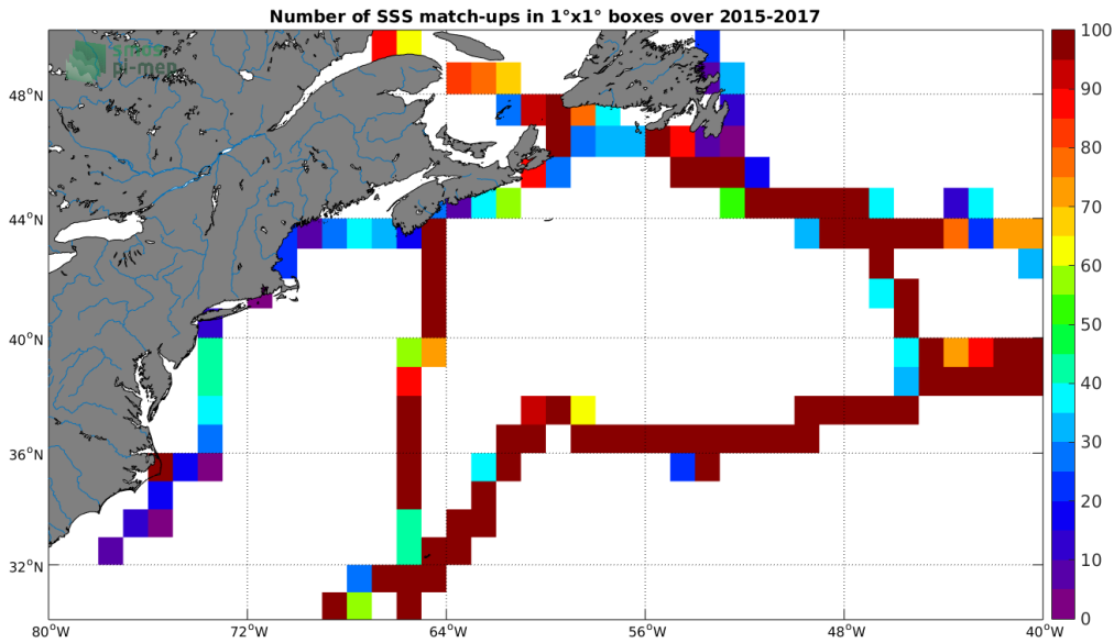
Figure 4: Number of SSS match-ups between TSG-GOSUD-Sailing-ship SSS and the SMAP-L3-JPL-V4.3-MONTHLY-60KM SSS product for the Gulf Stream Pi-MEP region over 1°x1° boxes and for the full satellite product period.
