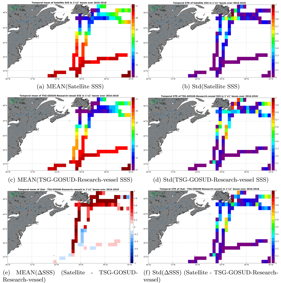
Figure 6: Temporal mean (left) and Std (right) of SSS from SMAP-L3-JPL-V4.3-MONTHLY-60KM (top), TSG-GOSUD-Research-vessel (middle), and of \Delta SSS (Satellite - TSG-GOSUD-Research-vessel). Only match-up pairs are used to generate these maps.
