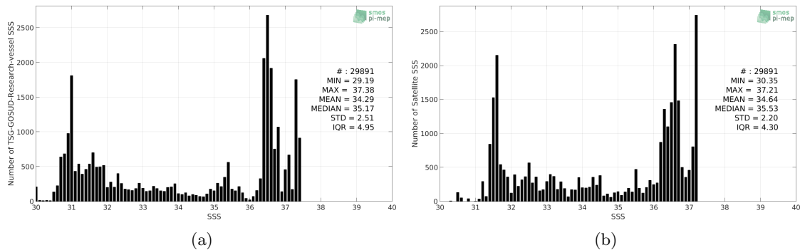
Figure 2: Histograms of SSS from TSG-GOSUD-Research-vessel (a) and SMAP-L3-JPL-V4.3-MONTHLY-60KM (b) considering all match-up pairs per bins of 0.1 over the Gulf Stream Pi-MEP region and for the full satellite product period.
