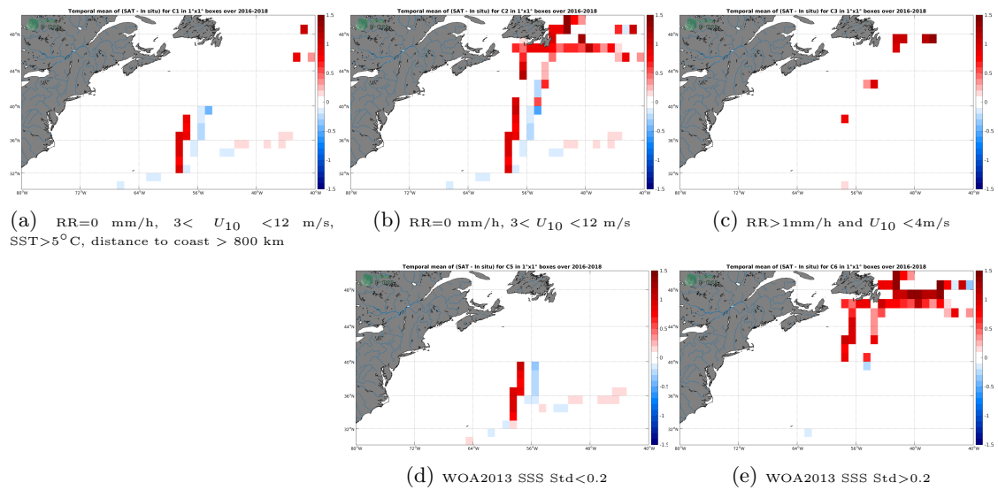
Figure 12: Temporal mean gridded over spatial boxes of size 1^\circ \times 1^\circ of \Delta SSS (SMAP-L3-JPL-V4.3-MONTHLY-60KM - TSG-GOSUD-Research-vessel) for 5 different subdatasets corresponding to: RR=0 mm/h, 3 < U_{10} < 12 m/s, SST > 5°C, distance to coast > 800 km (a), RR=0 mm/h, 3 < U_{10} < 12 m/s (b), RR > 1mm/h and U_{10} < 4 m/s (c), WOA2013 SSS Std < 0.2 (d), WOA2013 SSS Std > 0.2 (e).
