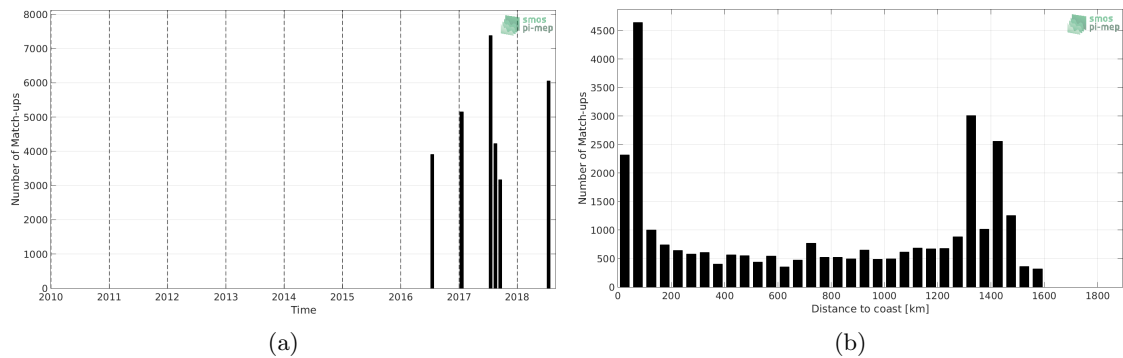
Figure 1: Number of match-ups between TSG-GOSUD-Research-vessel and SMAP-L3-JPL-V4.3-MONTHLY-60KM SSS as a function of time (a) and as function of the distance to coast (b) over the Gulf Stream Pi-MEP region and for the full satellite product period.
