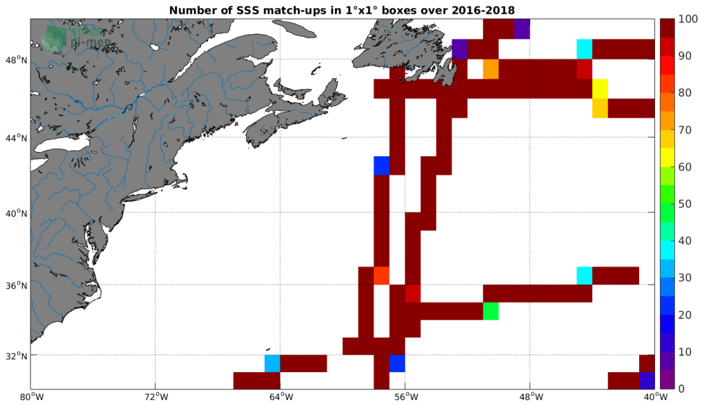
Figure 4: Number of SSS match-ups between TSG-GOSUD-Research-vessel SSS and the SMAP-L3-JPL-V4.3-MONTHLY-60KM SSS product for the Gulf Stream Pi-MEP region over 1°x1° boxes and for the full satellite product period.
