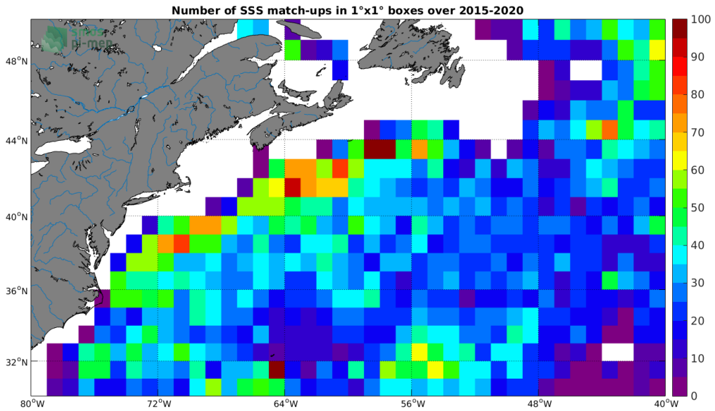
Figure 4: Number of SSS match-ups between Argo SSS and the SMAP-L3-JPL-V4.3-MONTHLY-60KM SSS product for the Gulf Stream Pi-MEP region over 1°x1° boxes and for the full satellite product period.
