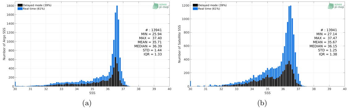
Figure 2: Histograms of SSS from Argo (a) and SMAP-L3-JPL-V4.3-MONTHLY-60KM (b) considering all match-up pairs per bins of 0.1 over the Gulf Stream Pi-MEP region and for the full satellite product period.
