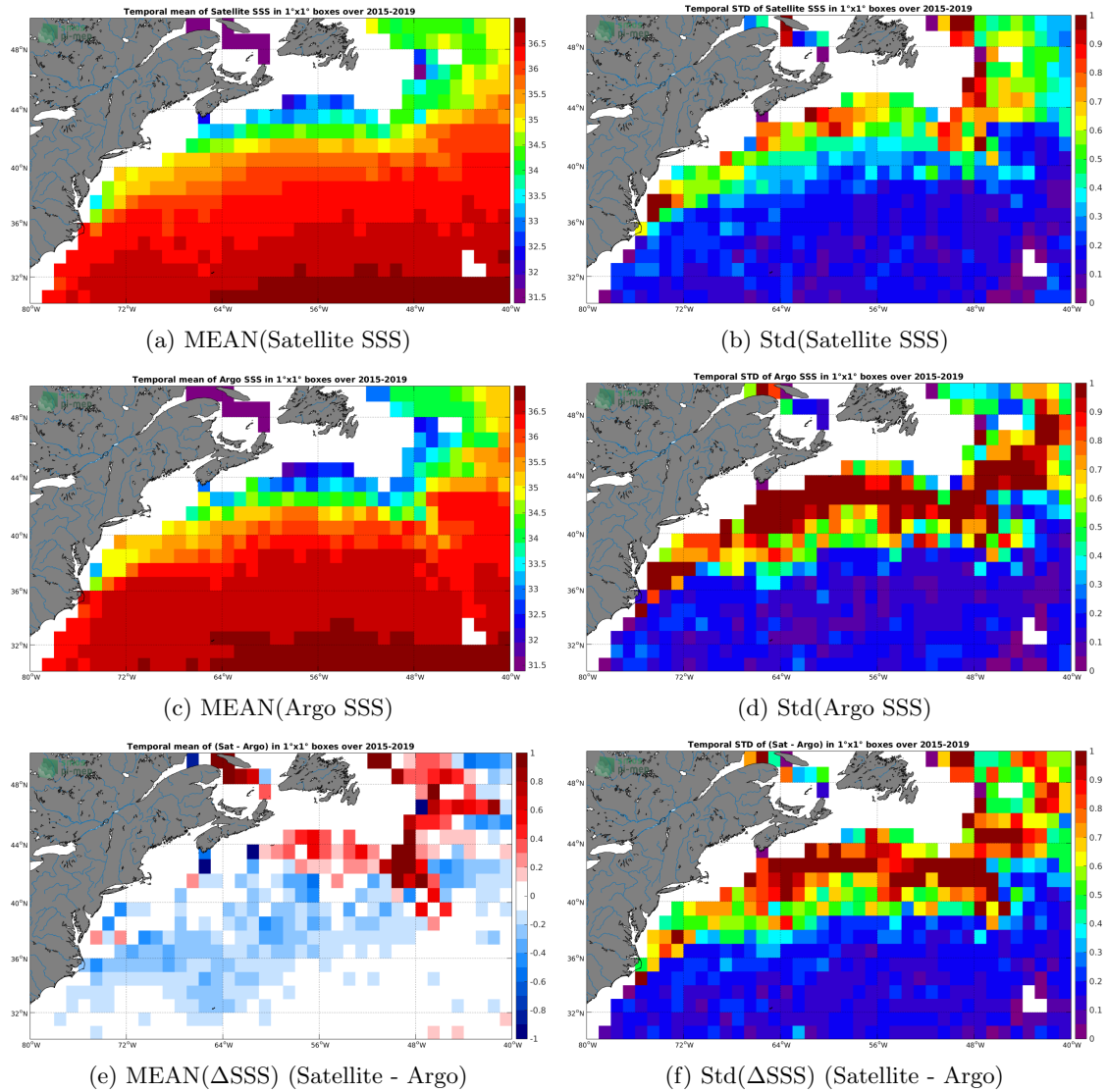
Figure 6: Temporal mean (left) and Std (right) of SSS from SMAP-L3-JPL-V4.3-MONTHLY-60KM (top), Argo (middle), and of \Delta SSS (Satellite - Argo). Only match-up pairs are used to generate these maps.
