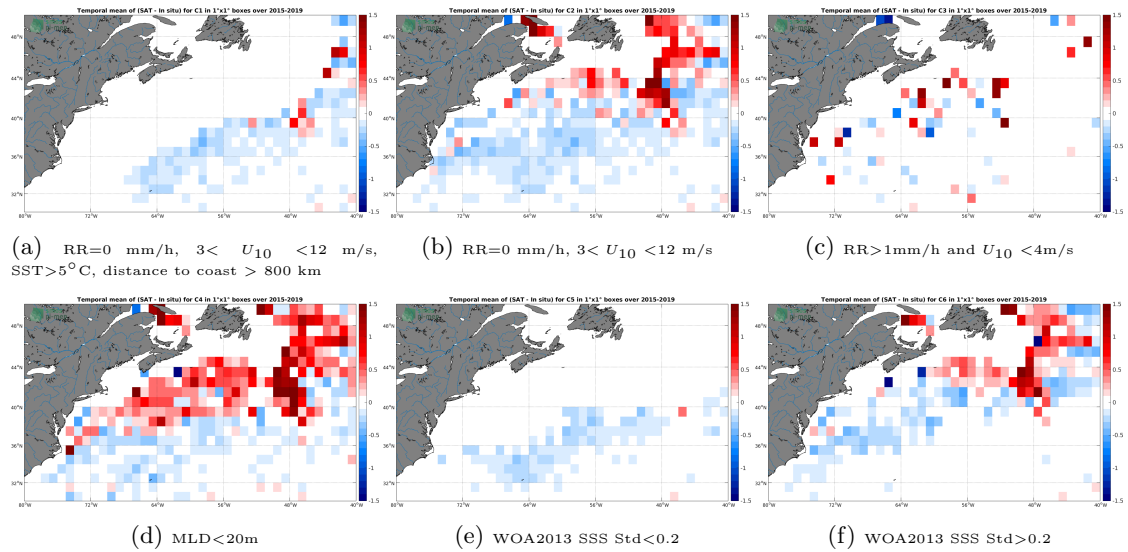
Figure 12: Temporal mean gridded over spatial boxes of size 1^\circ \times 1^\circ of \Delta SSS (SMAP-L3-JPL-V4.3-MONTHLY-60KM - Argo) for 6 different subdatasets corresponding to:RR=0 mm/h, 3 < U_{10} < 12 m/s, SST > 5^\circ\text{C} , distance to coast > 800 km (a), RR=0 mm/h, 3 < U_{10} < 12 m/s (b), RR > 1 mm/h and U_{10} < 4 m/s (c),MLD < 20 m (d),WOA2013 SSS Std < 0.2 (e),WOA2013 SSS Std > 0.2 (f).
