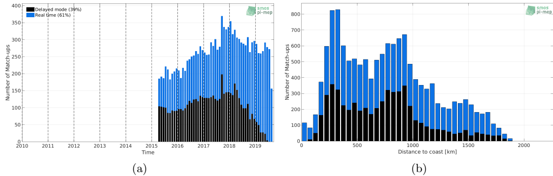
Figure 1: Number of match-ups between Argo and SMAP-L3-JPL-V4.3-MONTHLY-60KM SSS as a function of time (a) and as function of the distance to coast (b) over the Gulf Stream Pi-MEP region and for the full satellite product period.
