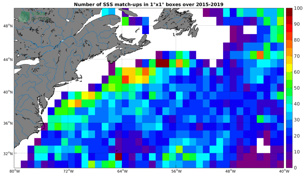
Figure 4: Number of SSS match-ups between Argo SSS and the SMAP-L3-JPL-V4.3-MONTHLY-60KM SSS product for the Gulf Stream Pi-MEP region over 1^\circ \times 1^\circ boxes and for the full satellite product period.
