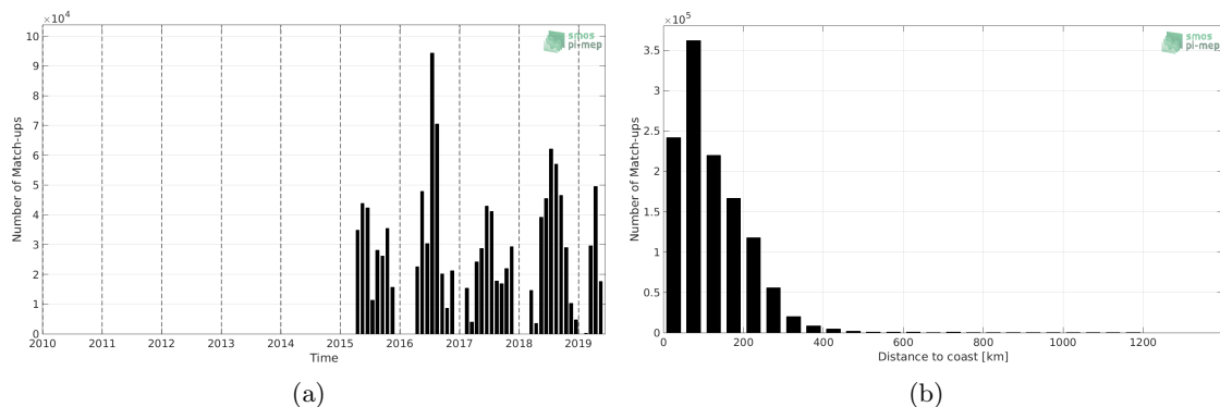
Figure 1: Number of match-ups between TSG-SAMOS and SMAP-L3-JPL-V4.2-8DAY-RUNNING-60KM SSS as a function of time (a) and as function of the distance to coast (b) over the Gulf Stream Pi-MEP region and for the full satellite product period.
