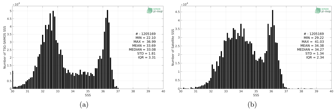
Figure 2: Histograms of SSS from TSG-SAMOS (a) and SMAP-L3-JPL-V4.2-8DAY-RUNNING-60KM (b) considering all match-up pairs per bins of 0.1 over the Gulf Stream Pi-MEP region and for the full satellite product period.
