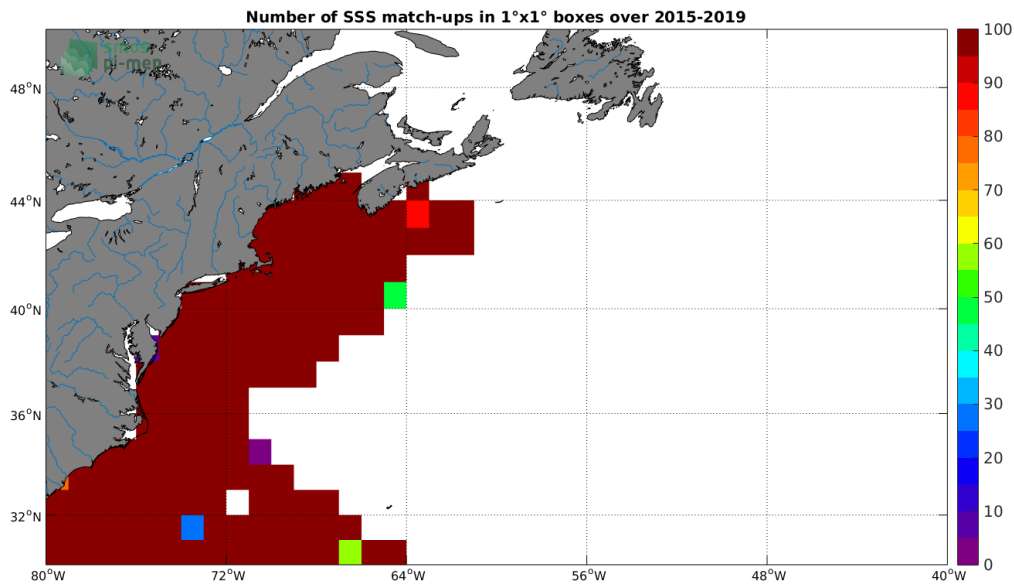
Figure 4: Number of SSS match-ups between TSG-SAMOS SSS and the SMAP-L3-JPL-V4.2-8DAY-RUNNING-60KM SSS product for the Gulf Stream Pi-MEP region over 1^\circ \times 1^\circ boxes and for the full satellite product period.
