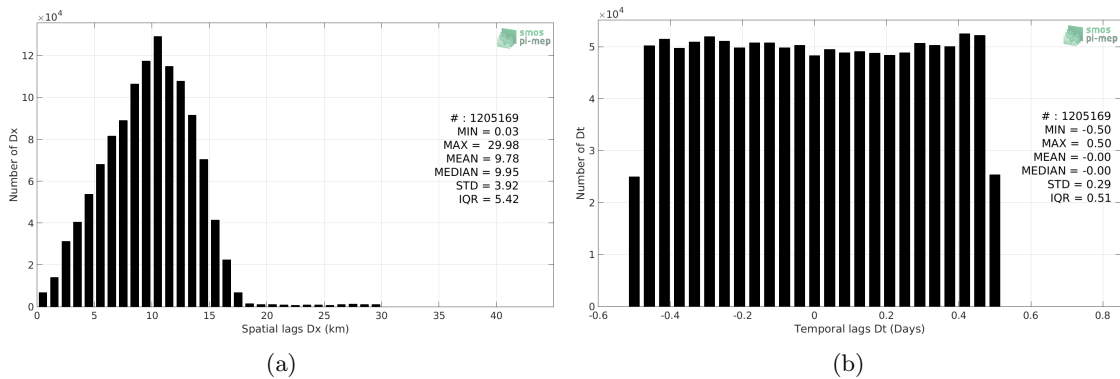
Figure 5: Histograms of the spatial (a) and temporal (b) lags between the time of the TSG-SAMOS measurements and the date of the corresponding SMAP-L3-JPL-V4.2-8DAY-RUNNING-60KM SSS product.
