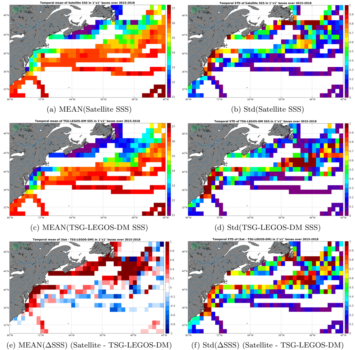
Figure 6: Temporal mean (left) and Std (right) of SSS from SMAP-L3-JPL-V4.2-8DAY-RUNNING-60KM (top), TSG-LEGOS-DM (middle), and of \Delta SSS (Satellite - TSG-LEGOS-DM). Only match-up pairs are used to generate these maps.
