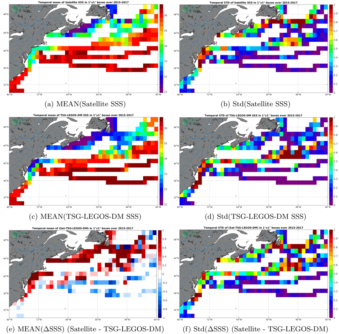
Figure 6: Temporal mean (left) and Std (right) of SSS from SMAP-L3-JPL-V4.2-8DAY-RUNNING-60KM (top), TSG-LEGOS-DM (middle), and of \Delta\text{SSS} (Satellite - TSG-LEGOS-DM). Only match-up pairs are used to generate these maps.
