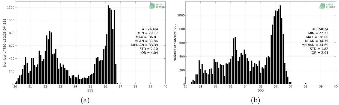
Figure 2: Histograms of SSS from TSG-LEGOS-DM (a) and SMAP-L3-JPL-V4.2-8DAY-RUNNING-60KM (b) considering all match-up pairs per bins of 0.1 over the Gulf Stream Pi-MEP region and for the full satellite product period.
