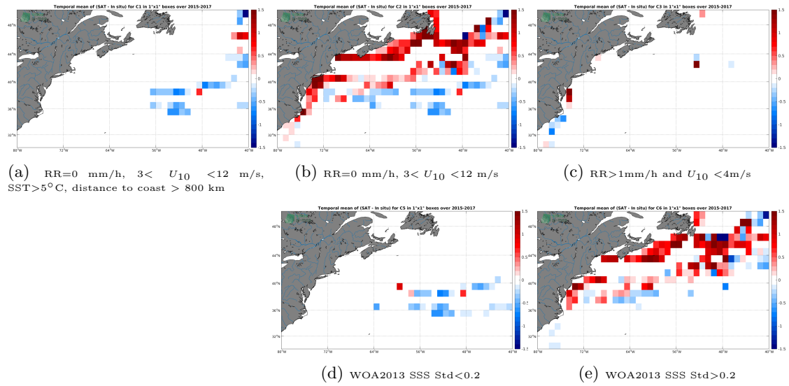
Figure 12: Temporal mean gridded over spatial boxes of size 1^\circ \times 1^\circ of \Delta SSS (SMAP-L3-JPL-V4.2-8DAY-RUNNING-60KM - TSG-LEGOS-DM) for 5 different subdatasets corresponding to:RR=0 mm/h, 3 < U_{10} < 12 m/s, SST >5^\circ C, distance to coast > 800 km (a), RR=0 mm/h, 3 < U_{10} < 12 m/s (b), RR >1 mm/h and U_{10} < 4 m/s (c), WOA2013 SSS Std <0.2 (d), WOA2013 SSS Std >0.2 (e).
