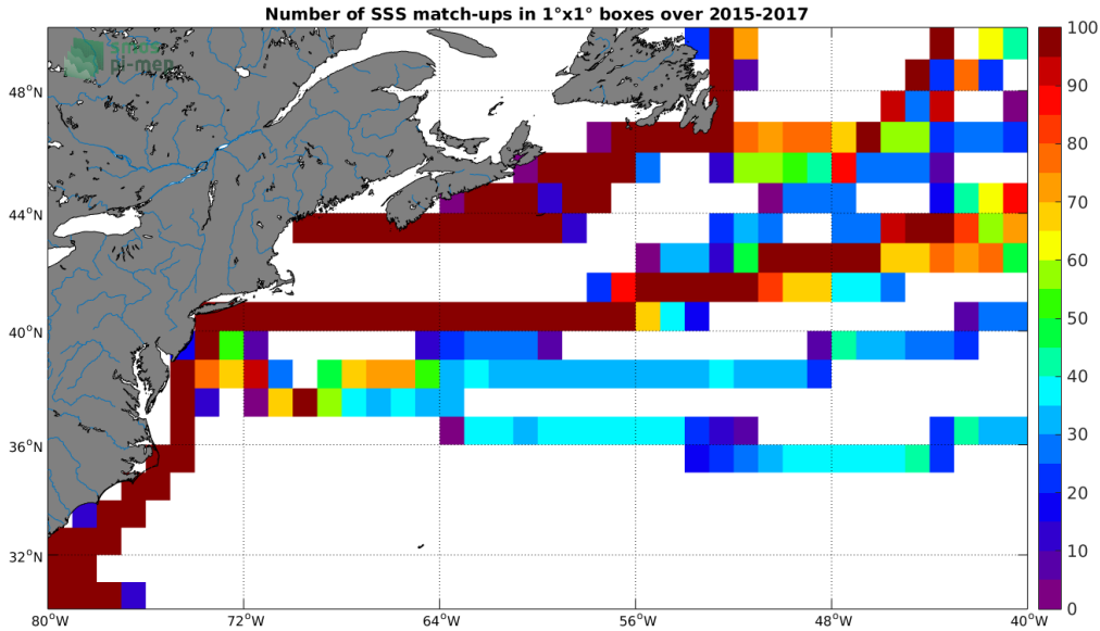
Figure 4: Number of SSS match-ups between TSG-LEGOS-DM SSS and the SMAP-L3-JPL-V4.2-8DAY-RUNNING-60KM SSS product for the Gulf Stream Pi-MEP region over 1^\circ \times 1^\circ boxes and for the full satellite product period.
