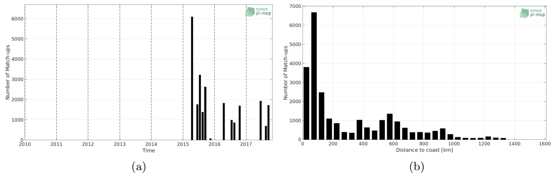
Figure 1: Number of match-ups between TSG-LEGOS-DM and SMAP-L3-JPL-V4.2-8DAY-RUNNING-60KM SSS as a function of time (a) and as function of the distance to coast (b) over the Gulf Stream Pi-MEP region and for the full satellite product period.
