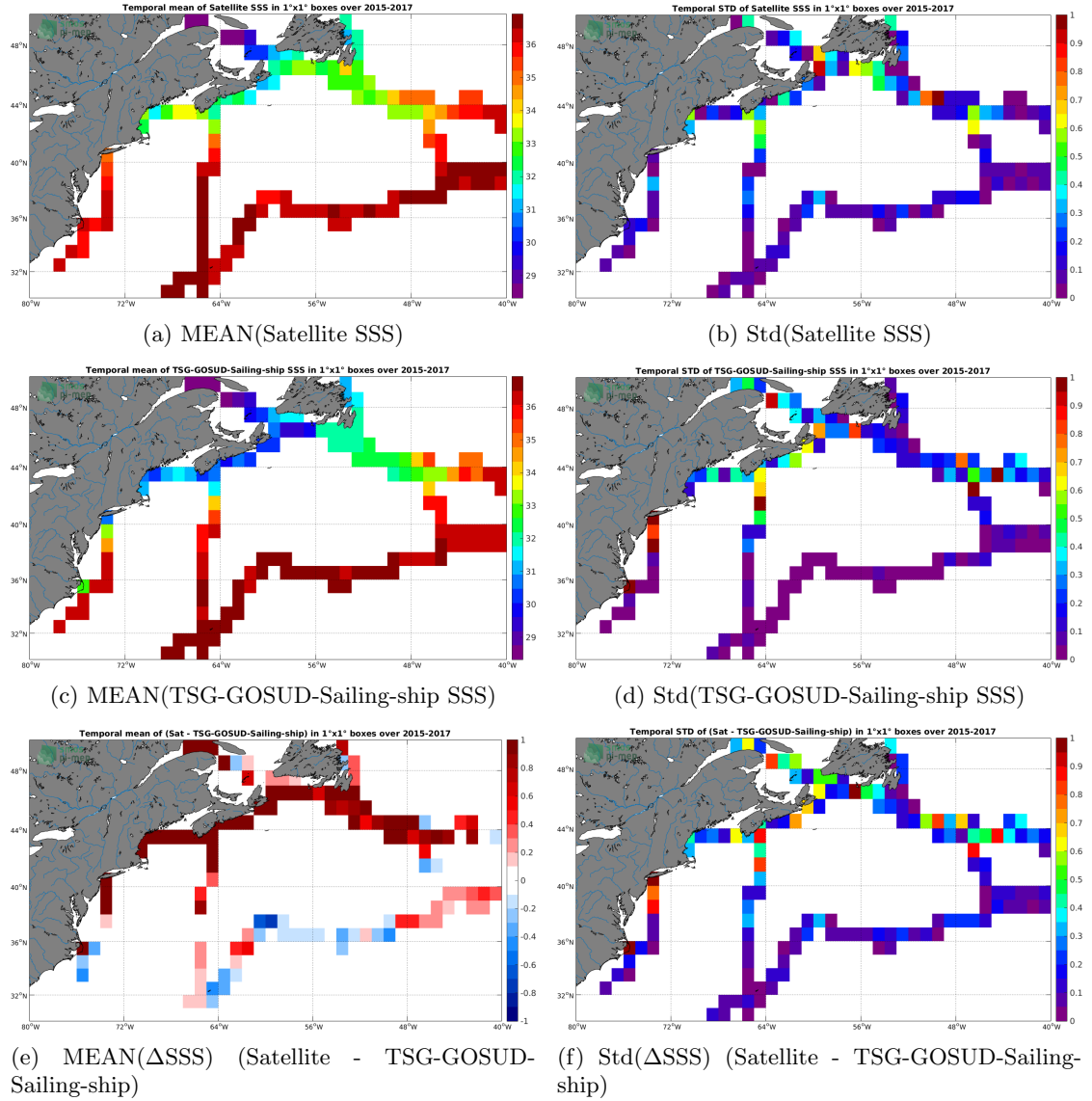
Figure 6: Temporal mean (left) and Std (right) of SSS from SMAP-L3-JPL-V4.2-8DAY-RUNNING-60KM (top), TSG-GOSUD-Sailing-ship (middle), and of \Delta\text{SSS} (Satellite - TSG-GOSUD-Sailing-ship). Only match-up pairs are used to generate these maps.
