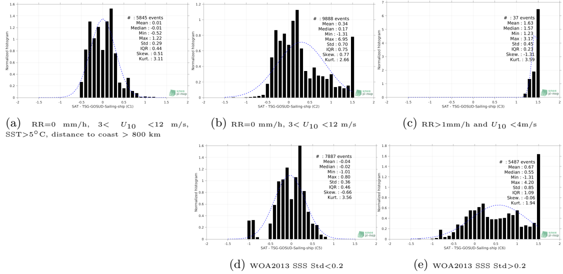
Figure 13: Normalized histogram of \Delta SSS (SMAP-L3-JPL-V4.2-8DAY-RUNNING-60KM - TSG-GOSUD-Sailing-ship) for 5 different subdatasets corresponding to: RR=0 mm/h, 3 < U_{10} < 12 m/s, SST>5°C, distance to coast > 800 km (a), RR=0 mm/h, 3 < U_{10} < 12 m/s (b), RR>1mm/h and U_{10} < 4 m/s (c), WOA2013 SSS Std<0.2 (d), WOA2013 SSS Std>0.2 (e).
