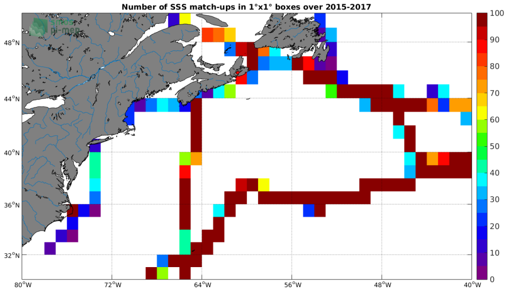
Figure 4: Number of SSS match-ups between TSG-GOSUD-Sailing-ship SSS and the SMAP-L3-JPL-V4.2-8DAY-RUNNING-60KM SSS product for the Gulf Stream Pi-MEP region over 1^\circ \times 1^\circ boxes and for the full satellite product period.
