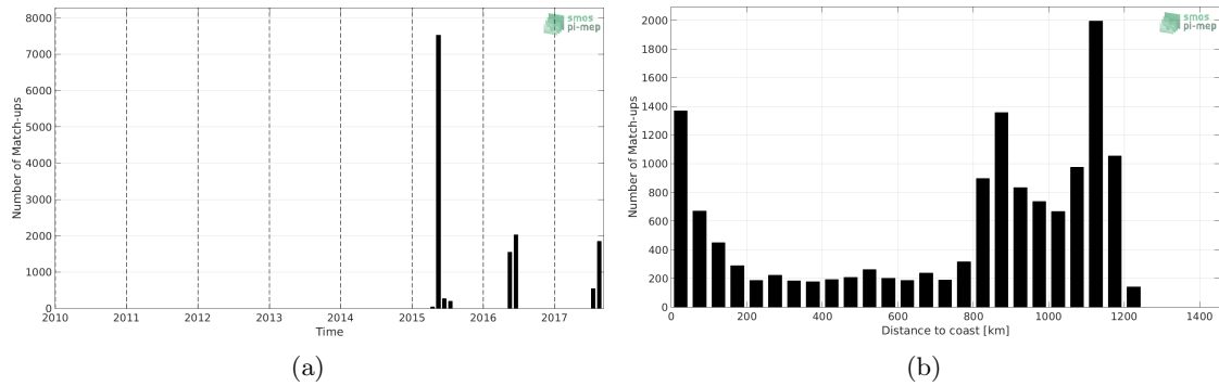
Figure 1: Number of match-ups between TSG-GOSUD-Sailing-ship and SMAP-L3-JPL-V4.2-8DAY-RUNNING-60KM SSS as a function of time (a) and as function of the distance to coast (b) over the Gulf Stream Pi-MEP region and for the full satellite product period.
