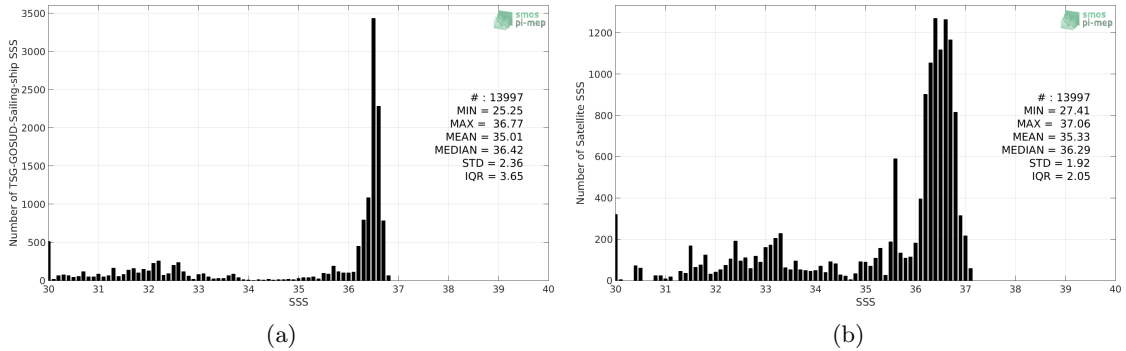
Figure 2: Histograms of SSS from TSG-GOSUD-Sailing-ship (a) and SMAP-L3-JPL-V4.2-8DAY-RUNNING-60KM (b) considering all match-up pairs per bins of 0.1 over the Gulf Stream Pi-MEP region and for the full satellite product period.
