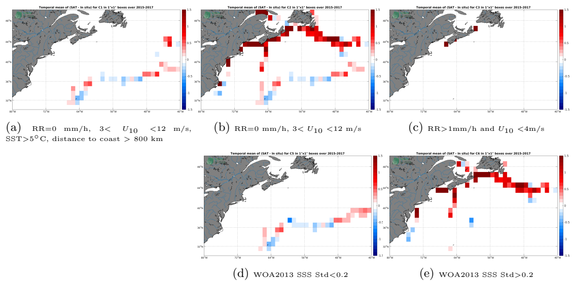
Figure 12: Temporal mean gridded over spatial boxes of size 1^\circ \times 1^\circ of \Delta SSS (SMAP-L3-JPL-V4.2-8DAY-RUNNING-60KM - TSG-GOSUD-Sailing-ship) for 5 different subdatasets corresponding to:RR=0 mm/h, 3 < U_{10} < 12 m/s, SST>5°C, distance to coast > 800 km (a), RR=0 mm/h, 3 < U_{10} < 12 m/s (b), RR>1mm/h and U_{10} < 4 m/s (c), WOA2013 SSS Std<0.2 (d), WOA2013 SSS Std>0.2 (e).
