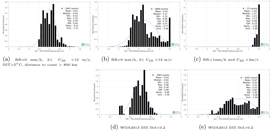
Figure 13: Normalized histogram of \Delta\text{SSS} (SMAP-L3-JPL-V4.2-8DAY-RUNNING-60KM - TSG-GOSUD-Sailing-ship) for 5 different subdatasets corresponding to: RR=0 mm/h, 3 < U_{10} < 12 m/s, SST > 5^{\circ}\text{C} , distance to coast > 800 km (a), RR=0 mm/h, 3 < U_{10} < 12 m/s (b), RR > 1\text{mm/h} and U_{10} < 4\text{m/s} (c), WOA2013 SSS Std < 0.2 (d), WOA2013 SSS Std > 0.2 (e).
