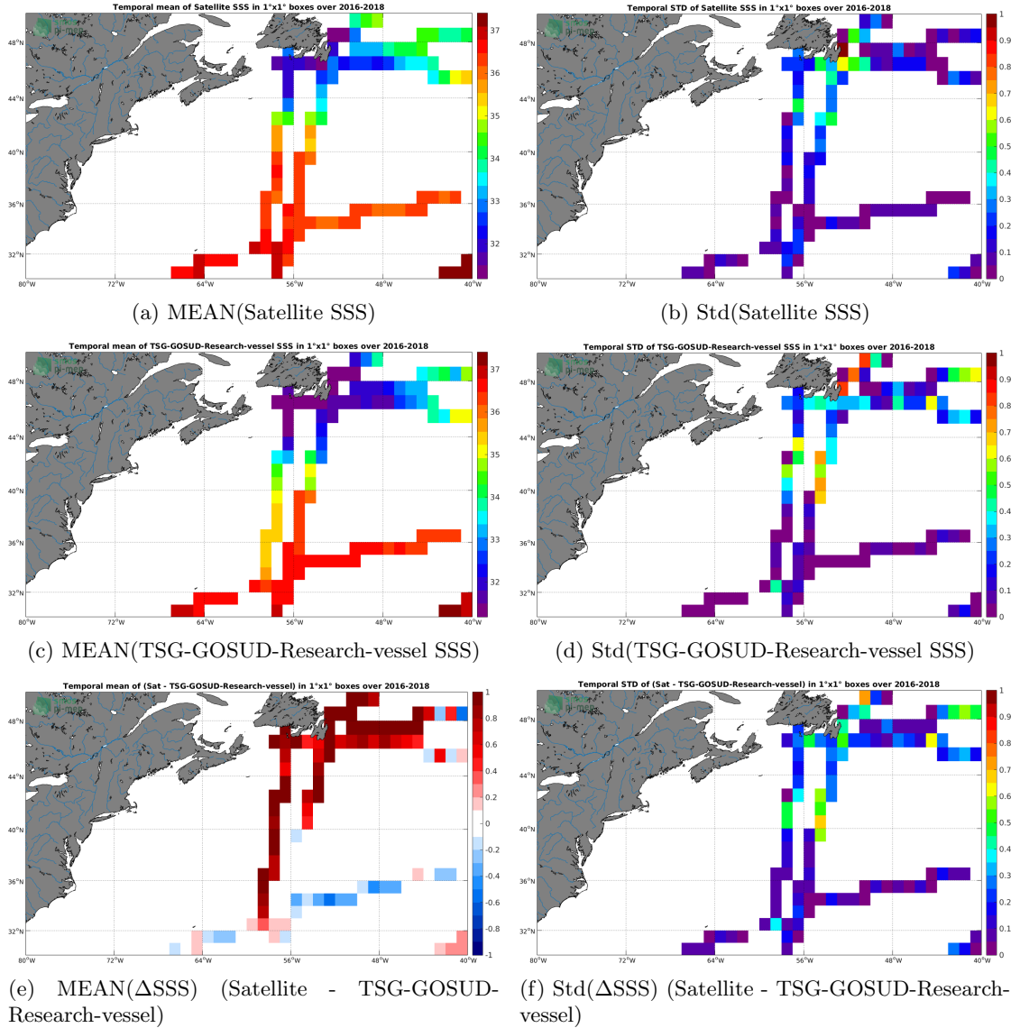
Figure 6: Temporal mean (left) and Std (right) of SSS from SMAP-L3-JPL-V4.2-8DAY-RUNNING-60KM (top), TSG-GOSUD-Research-vessel (middle), and of \Delta SSS (Satellite - TSG-GOSUD-Research-vessel). Only match-up pairs are used to generate these maps.
