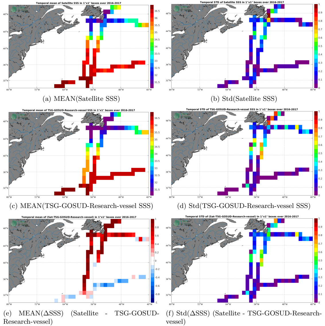
Figure 6: Temporal mean (left) and Std (right) of SSS from SMAP-L3-JPL-V4.2-8DAY-RUNNING-60KM (top), TSG-GOSUD-Research-vessel (middle), and of \Delta\text{SSS} (Satellite - TSG-GOSUD-Research-vessel). Only match-up pairs are used to generate these maps.
