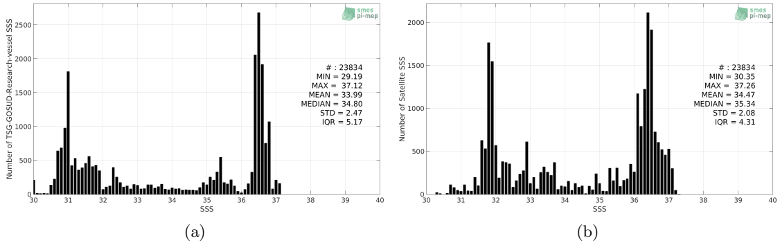
Figure 2: Histograms of SSS from TSG-GOSUD-Research-vessel (a) and SMAP-L3-JPL-V4.2-8DAY-RUNNING-60KM (b) considering all match-up pairs per bins of 0.1 over the Gulf Stream Pi-MEP region and for the full satellite product period.
