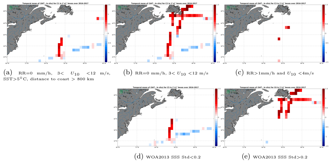
Figure 12: Temporal mean gridded over spatial boxes of size 1^\circ \times 1^\circ of \Delta SSS (SMAP-L3-JPL-V4.2-8DAY-RUNNING-60KM - TSG-GOSUD-Research-vessel) for 5 different subdatasets corresponding to: RR=0 mm/h, 3 < U_{10} < 12 m/s, SST > 5^\circ C , distance to coast > 800 km (a), RR=0 mm/h, 3 < U_{10} < 12 m/s (b), RR > 1 mm/h and U_{10} < 4 m/s (c), WOA2013 SSS Std < 0.2 (d), WOA2013 SSS Std > 0.2 (e).
