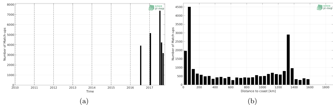
Figure 1: Number of match-ups between TSG-GOSUD-Research-vessel and SMAP-L3-JPL-V4.2-8DAY-RUNNING-60KM SSS as a function of time (a) and as function of the distance to coast (b) over the Gulf Stream Pi-MEP region and for the full satellite product period.
