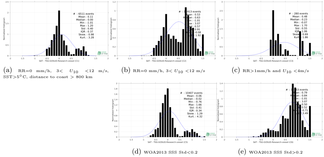
Figure 13: Normalized histogram of \Delta SSS (SMAP-L3-JPL-V4.2-8DAY-RUNNING-60KM - TSG-GOSUD-Research-vessel) for 5 different subdatasets corresponding to: RR=0 mm/h, 3 < U_{10} < 12 m/s, SST >5^{\circ} C, distance to coast > 800 km (a), RR=0 mm/h, 3 < U_{10} < 12 m/s (b), RR >1 mm/h and U_{10} < 4 m/s (c), WOA2013 SSS Std <0.2 (d), WOA2013 SSS Std >0.2 (e).
