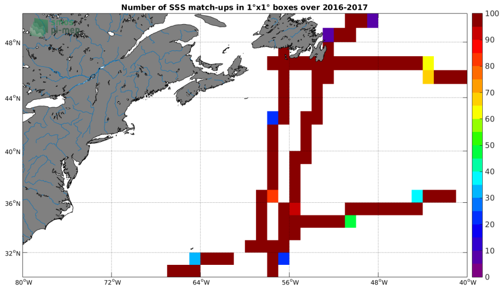
Figure 4: Number of SSS match-ups between TSG-GOSUD-Research-vessel SSS and the SMAP-L3-JPL-V4.2-8DAY-RUNNING-60KM SSS product for the Gulf Stream Pi-MEP region over 1^\circ \times 1^\circ boxes and for the full satellite product period.
