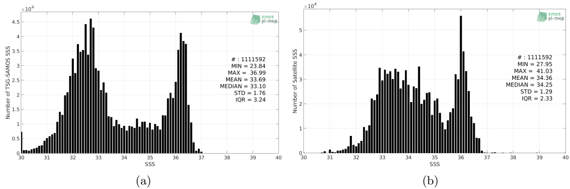
Figure 2: Histograms of SSS from TSG-SAMOS (a) and SMAP-L3-JPL-V4.2-MONTHLY-60KM (b) considering all match-up pairs per bins of 0.1 over the Gulf Stream Pi-MEP region and for the full satellite product period.
