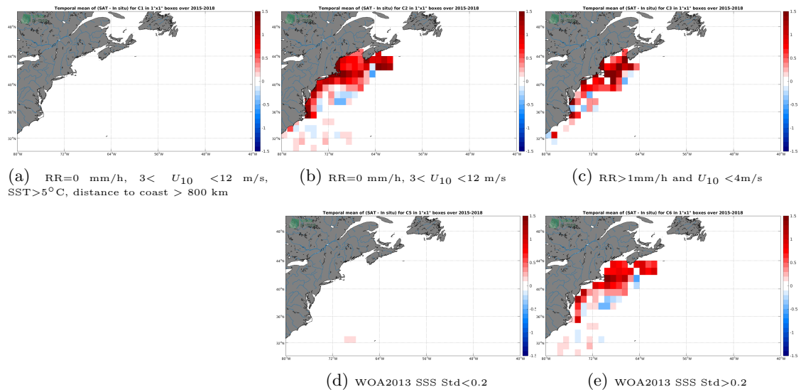
Figure 12: Temporal mean gridded over spatial boxes of size 1^\circ \times 1^\circ of \Delta SSS (SMAP-L3-JPL-V4.2-MONTHLY-60KM - TSG-SAMOS) for 5 different subdatasets corresponding to:RR=0 mm/h, 3 < U_{10} < 12 m/s, SST >5^\circ C, distance to coast > 800 km (a), RR=0 mm/h, 3 < U_{10} < 12 m/s (b), RR >1 mm/h and U_{10} < 4 m/s (c), WOA2013 SSS Std <0.2 (d), WOA2013 SSS Std >0.2 (e).
