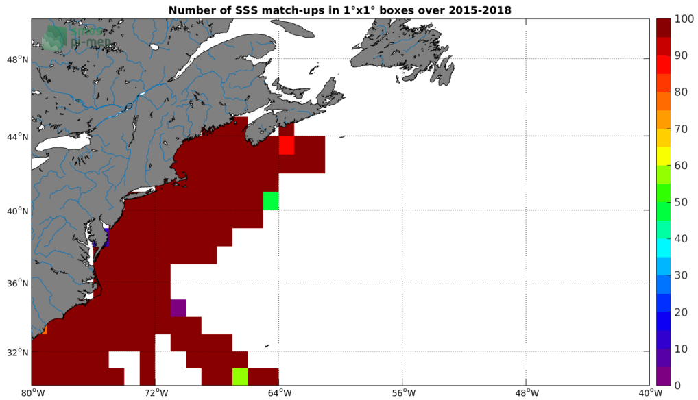
Figure 4: Number of SSS match-ups between TSG-SAMOS SSS and the SMAP-L3-JPL-V4.2-MONTHLY-60KM SSS product for the Gulf Stream Pi-MEP region over 1^\circ \times 1^\circ boxes and for the full satellite product period.
