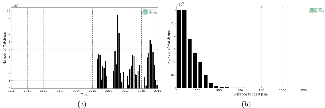
Figure 1: Number of match-ups between TSG-SAMOS and SMAP-L3-JPL-V4.2-MONTHLY-60KM SSS as a function of time (a) and as function of the distance to coast (b) over the Gulf Stream Pi-MEP region and for the full satellite product period.
