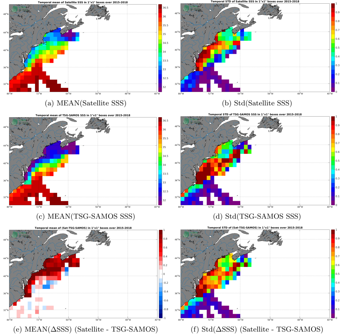
Figure 6: Temporal mean (left) and Std (right) of SSS from SMAP-L3-JPL-V4.2-MONTHLY-60KM (top), TSG-SAMOS (middle), and of \Delta SSS (Satellite - TSG-SAMOS). Only match-up pairs are used to generate these maps.
