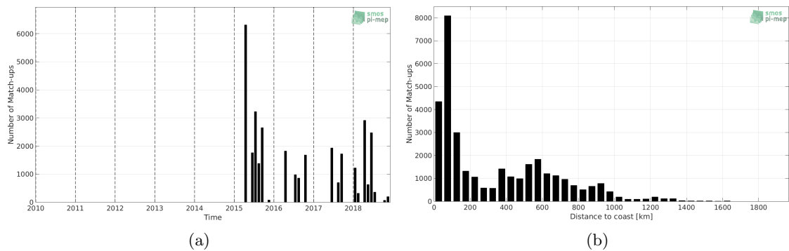
Figure 1: Number of match-ups between TSG-LEGOS-DM and SMAP-L3-JPL-V4.2-MONTHLY-60KM SSS as a function of time (a) and as function of the distance to coast (b) over the Gulf Stream Pi-MEP region and for the full satellite product period.
