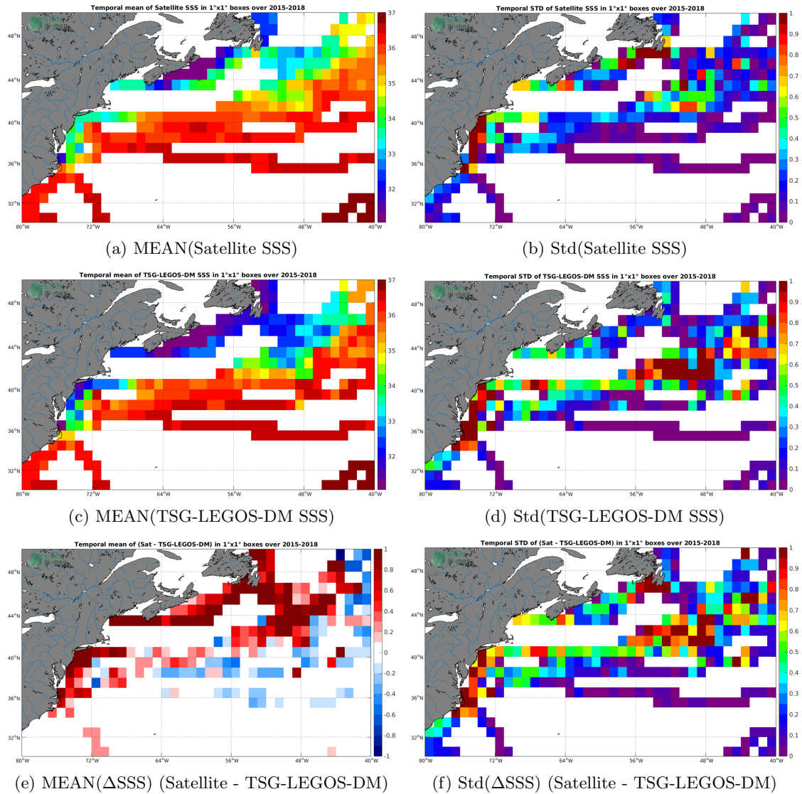
Figure 6: Temporal mean (left) and Std (right) of SSS from SMAP-L3-JPL-V4.2-MONTHLY-60KM (top), TSG-LEGOS-DM (middle), and of \Delta SSS (Satellite - TSG-LEGOS-DM). Only match-up pairs are used to generate these maps.
