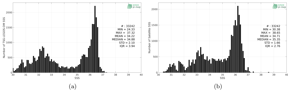
Figure 2: Histograms of SSS from TSG-LEGOS-DM (a) and SMAP-L3-JPL-V4.2-MONTHLY-60KM (b) considering all match-up pairs per bins of 0.1 over the Gulf Stream Pi-MEP region and for the full satellite product period.
