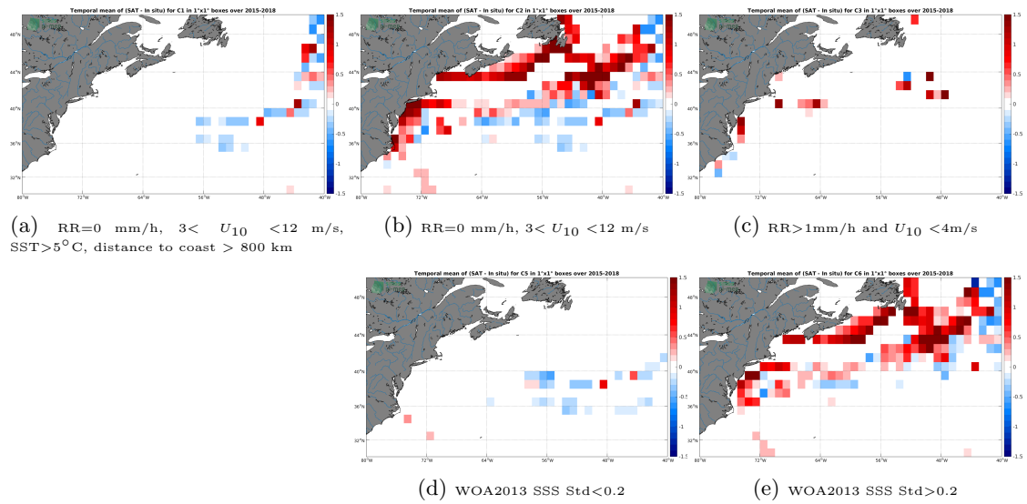
Figure 12: Temporal mean gridded over spatial boxes of size 1^\circ \times 1^\circ of \Delta SSS (SMAP-L3-JPL-V4.2-MONTHLY-60KM - TSG-LEGOS-DM) for 5 different subdatasets corresponding to:RR=0 mm/h, 3 < U_{10} < 12 m/s, SST >5^\circ C, distance to coast > 800 km (a), RR=0 mm/h, 3 < U_{10} < 12 m/s (b), RR >1 mm/h and U_{10} < 4 m/s (c), WOA2013 SSS Std <0.2 (d), WOA2013 SSS Std >0.2 (e).
