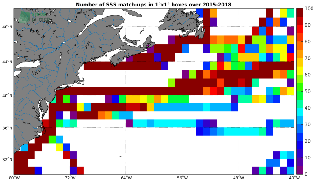
Figure 4: Number of SSS match-ups between TSG-LEGOS-DM SSS and the SMAP-L3-JPL-V4.2-MONTHLY-60KM SSS product for the Gulf Stream Pi-MEP region over 1^\circ \times 1^\circ boxes and for the full satellite product period.
