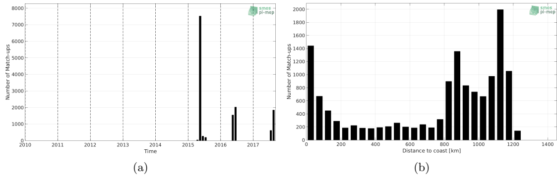
Figure 1: Number of match-ups between TSG-GOSUD-Sailing-ship and SMAP-L3-JPL-V4.2-MONTHLY-60KM SSS as a function of time (a) and as function of the distance to coast (b) over the Gulf Stream Pi-MEP region and for the full satellite product period.
