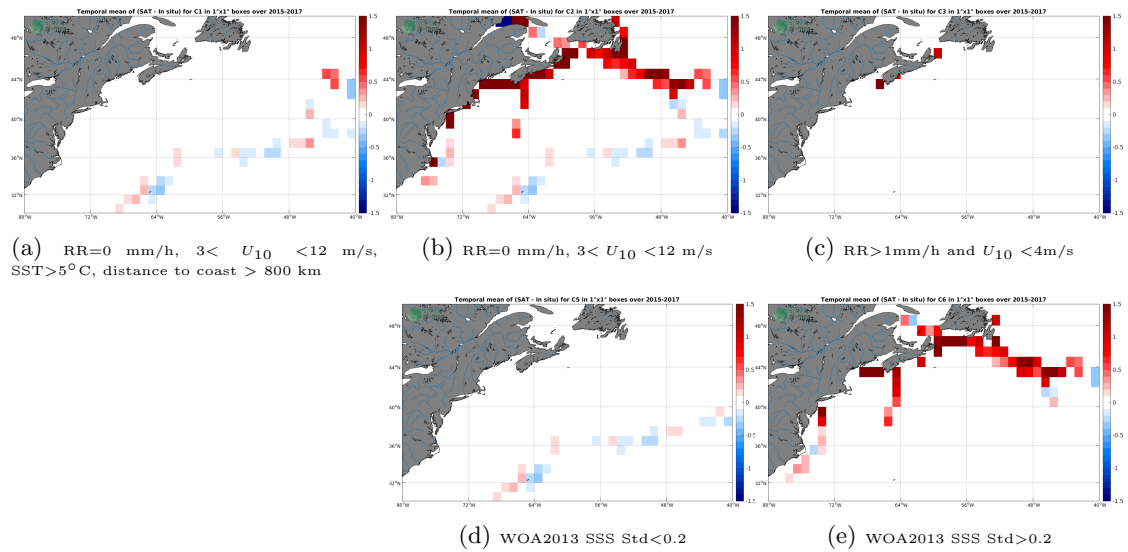
Figure 12: Temporal mean gridded over spatial boxes of size 1^\circ \times 1^\circ of \Delta SSS (SMAP-L3-JPL-V4.2-MONTHLY-60KM - TSG-GOSUD-Sailing-ship) for 5 different subdatasets corresponding to:RR=0 mm/h, 3 < U_{10} < 12 m/s, SST >5^\circ C, distance to coast > 800 km (a), RR=0 mm/h, 3 < U_{10} < 12 m/s (b), RR >1 mm/h and U_{10} < 4 m/s (c), WOA2013 SSS Std <0.2 (d), WOA2013 SSS Std >0.2 (e).
