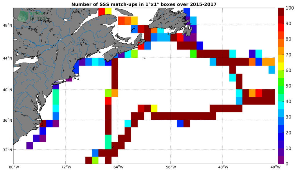
Figure 4: Number of SSS match-ups between TSG-GOSUD-Sailing-ship SSS and the SMAP-L3-JPL-V4.2-MONTHLY-60KM SSS product for the Gulf Stream Pi-MEP region over 1^\circ \times 1^\circ boxes and for the full satellite product period.
