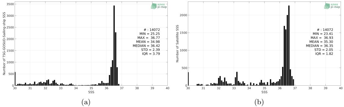
Figure 2: Histograms of SSS from TSG-GOSUD-Sailing-ship (a) and SMAP-L3-JPL-V4.2-MONTHLY-60KM (b) considering all match-up pairs per bins of 0.1 over the Gulf Stream Pi-MEP region and for the full satellite product period.
