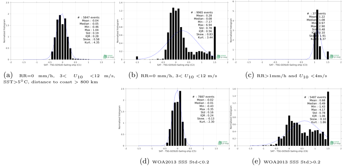
Figure 13: Normalized histogram of \Delta SSS (SMAP-L3-JPL-V4.2-MONTHLY-60KM - TSG-GOSUD-Sailing-ship) for 5 different subdatasets corresponding to: RR=0 mm/h, 3 < U_{10} < 12 m/s, SST>5°C, distance to coast > 800 km (a), RR=0 mm/h, 3 < U_{10} < 12 m/s (b), RR>1mm/h and U_{10} < 4 m/s (c), WOA2013 SSS Std<0.2 (d), WOA2013 SSS Std>0.2 (e).
