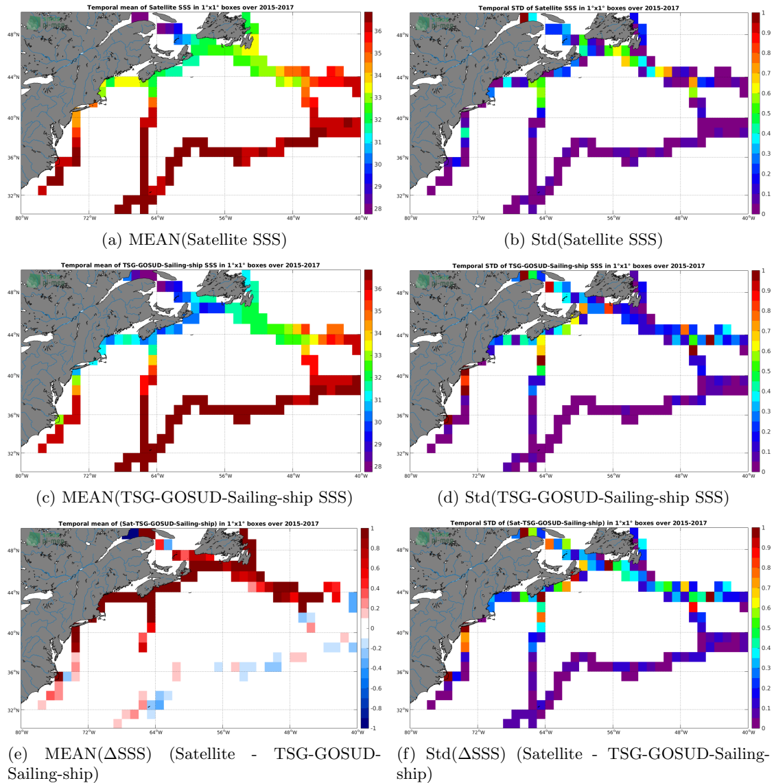
Figure 6: Temporal mean (left) and Std (right) of SSS from SMAP-L3-JPL-V4.2-MONTHLY-60KM (top), TSG-GOSUD-Sailing-ship (middle), and of \Delta SSS (Satellite - TSG-GOSUD-Sailing-ship). Only match-up pairs are used to generate these maps.
