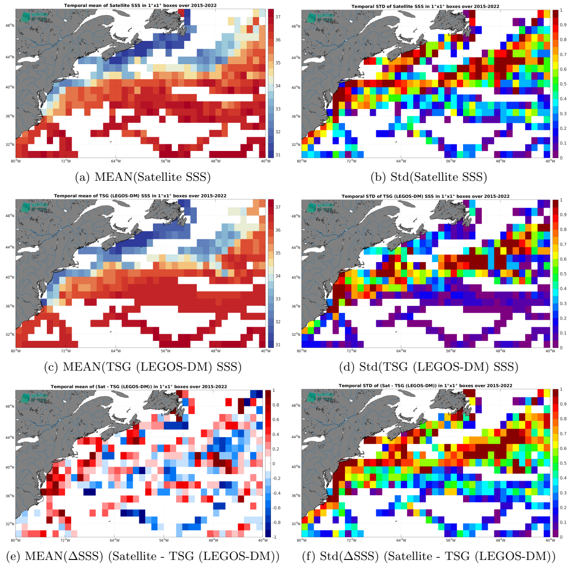
Figure 7: Temporal mean (left) and Std (right) of SSS from SMAP SSS L2 v6 (RSS) (top), TSG (LEGOS-DM) (middle), and of \Delta SSS (Satellite - TSG (LEGOS-DM)). Only match-up pairs are used to generate these maps.
