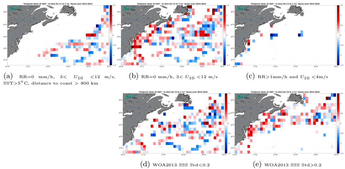
Figure 14: Temporal mean gridded over spatial boxes of size 1^\circ \times 1^\circ of \Delta SSS (SMAP SSS L2 v6 (RSS) - TSG (LEGOS-DM)) for 5 different subdatasets corresponding to:RR=0 mm/h, 3 < U_{10} < 12 m/s, SST > 5^\circ C , distance to coast > 800 km (a), RR=0 mm/h, 3 < U_{10} < 12 m/s (b), RR>1mm/h and U_{10} < 4 m/s (c), WOA2013 SSS Std<0.2 (d), WOA2013 SSS Std>0.2 (e).
