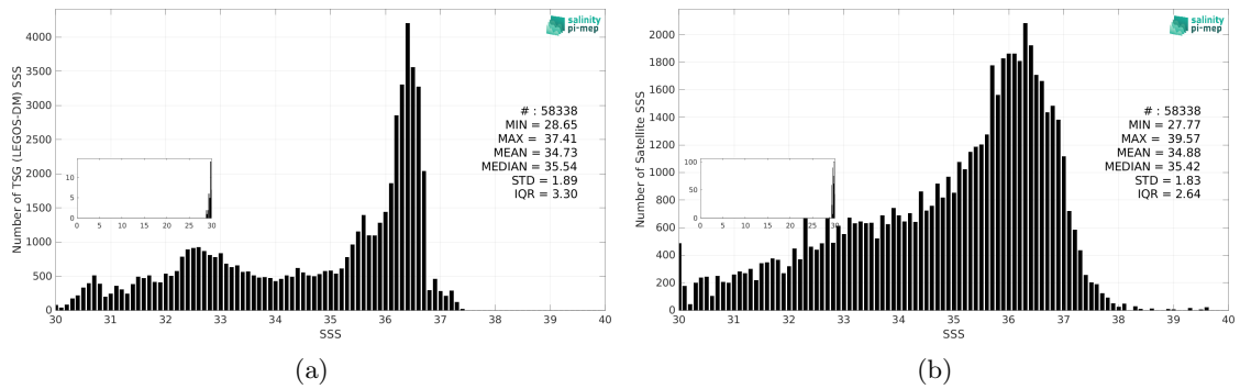
Figure 3: Histograms of SSS from TSG (LEGOS-DM) (a) and SMAP SSS L2 v6 (RSS) (b) considering all match-up pairs per bins of 0.1 over the Gulf Stream Pi-MEP region and for the full satellite product period.
