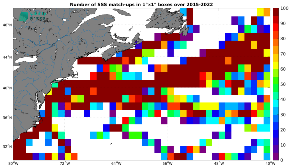
Figure 5: Number of SSS match-ups between TSG (LEGOS-DM) SSS and the SMAP SSS L2 v6 (RSS) SSS product for the Gulf Stream Pi-MEP region over 1^\circ \times 1^\circ boxes and for the full satellite product period.
