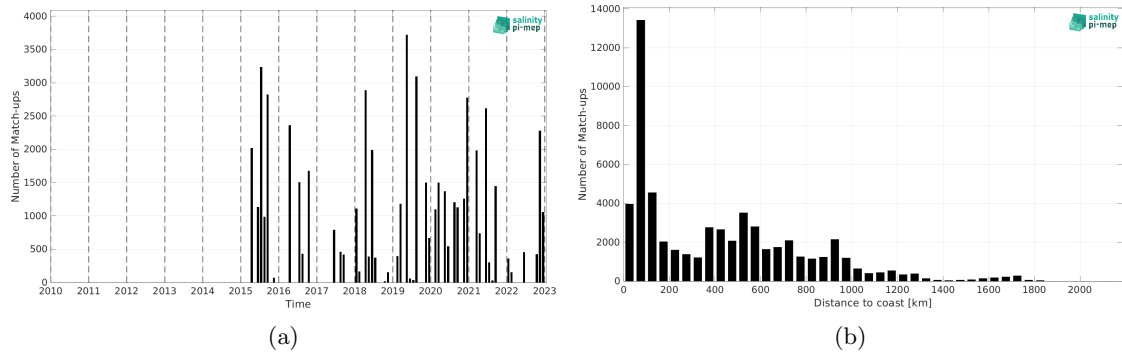
Figure 2: Number of match-ups between TSG (LEGOS-DM) and SMAP SSS L2 v6 (RSS) SSS as a function of time (a) and as function of the distance to coast (b) over the Gulf Stream Pi-MEP region and for the full satellite product period.
