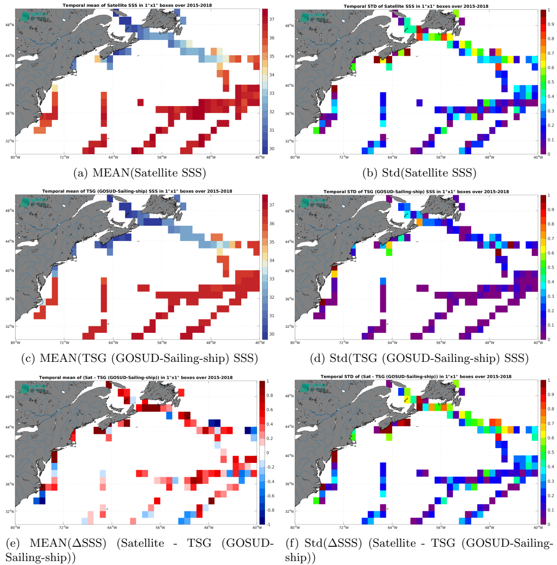
Figure 7: Temporal mean (left) and Std (right) of SSS from SMAP SSS L2 v6 (RSS) (top), TSG (GOSUD-Sailing-ship) (middle), and of \Delta SSS (Satellite - TSG (GOSUD-Sailing-ship)). Only match-up pairs are used to generate these maps.
