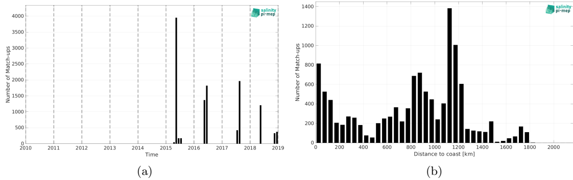
Figure 2: Number of match-ups between TSG (GOSUD-Sailing-ship) and SMAP SSS L2 v6 (RSS) SSS as a function of time (a) and as function of the distance to coast (b) over the Gulf Stream Pi-MEP region and for the full satellite product period.
