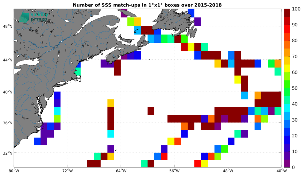
Figure 5: Number of SSS match-ups between TSG (GOSUD-Sailing-ship) SSS and the SMAP SSS L2 v6 (RSS) SSS product for the Gulf Stream Pi-MEP region over 1^\circ \times 1^\circ boxes and for the full satellite product period.
