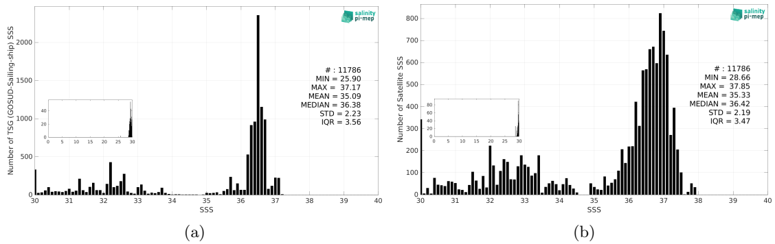
Figure 3: Histograms of SSS from TSG (GOSUD-Sailing-ship) (a) and SMAP SSS L2 v6 (RSS) (b) considering all match-up pairs per bins of 0.1 over the Gulf Stream Pi-MEP region and for the full satellite product period.
