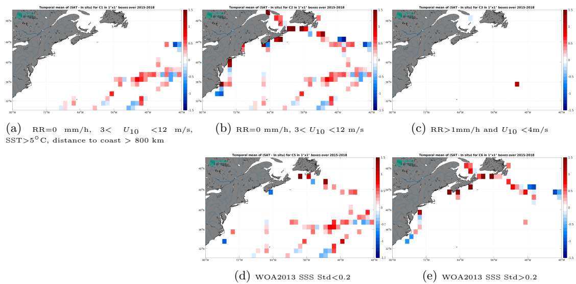
Figure 14: Temporal mean gridded over spatial boxes of size 1^\circ \times 1^\circ of \Delta SSS (SMAP SSS L2 v6 (RSS) - TSG (GOSUD-Sailing-ship)) for 5 different subdatasets corresponding to:RR=0 mm/h, 3 < U_{10} < 12 m/s, SST>5°C, distance to coast > 800 km (a), RR=0 mm/h, 3 < U_{10} < 12 m/s (b), RR>1mm/h and U_{10} < 4 m/s (c), WOA2013 SSS Std<0.2 (d), WOA2013 SSS Std>0.2 (e).
