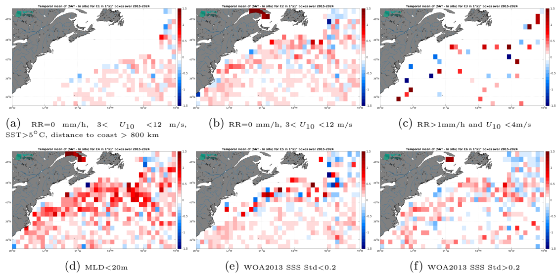
Figure 14: Temporal mean gridded over spatial boxes of size 1^\circ \times 1^\circ of \Delta SSS (SMAP SSS L2 v6 (RSS) - Argo) for 6 different subdatasets corresponding to:RR=0 mm/h, 3 < U_{10} < 12 m/s, SST > 5^\circ\text{C} , distance to coast > 800 km (a), RR=0 mm/h, 3 < U_{10} < 12 m/s (b), RR > 1 mm/h and U_{10} < 4 m/s (c),MLD < 20 m (d),WOA2013 SSS Std < 0.2 (e),WOA2013 SSS Std > 0.2 (f).
