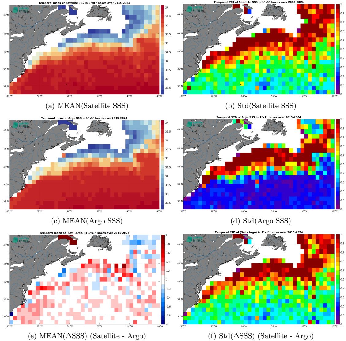
Figure 7: Temporal mean (left) and Std (right) of SSS from SMAP SSS L2 v6 (RSS) (top), Argo (middle), and of \Delta SSS (Satellite - Argo). Only match-up pairs are used to generate these maps.
