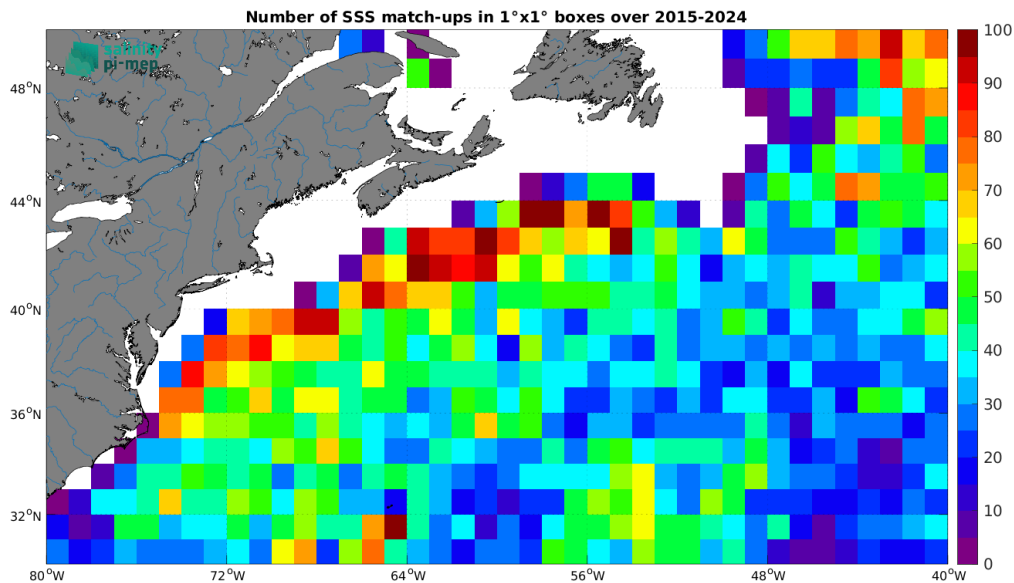
Figure 5: Number of SSS match-ups between Argo SSS and the SMAP SSS L2 v6 (RSS) SSS product for the Gulf Stream Pi-MEP region over 1^\circ \times 1^\circ boxes and for the full satellite product period.
