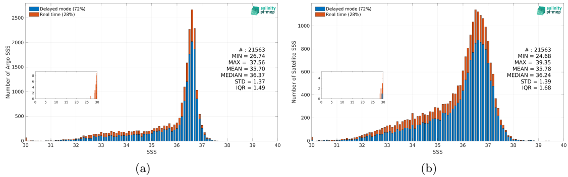
Figure 3: Histograms of SSS from Argo (a) and SMAP SSS L2 v6 (RSS) (b) considering all match-up pairs per bins of 0.1 over the Gulf Stream Pi-MEP region and for the full satellite product period.
