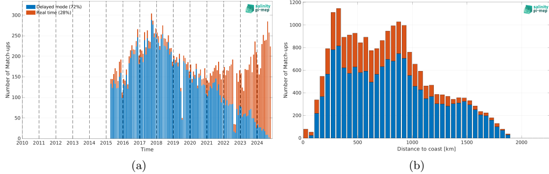
Figure 2: Number of match-ups between Argo and SMAP SSS L2 v6 (RSS) SSS as a function of time (a) and as function of the distance to coast (b) over the Gulf Stream Pi-MEP region and for the full satellite product period.
