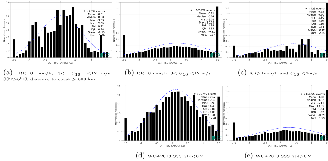
Figure 15: Normalized histogram of \Delta SSS (SMAP SSS L2 v6 - 40 km (RSS) - TSG (SAMOS)) for 5 different subdatasets corresponding to: RR=0 mm/h, 3 < U_{10} < 12 m/s, SST > 5°C, distance to coast > 800 km (a), RR=0 mm/h, 3 < U_{10} < 12 m/s (b), RR > 1mm/h and U_{10} < 4 m/s (c), WOA2013 SSS Std < 0.2 (d), WOA2013 SSS Std > 0.2 (e).
