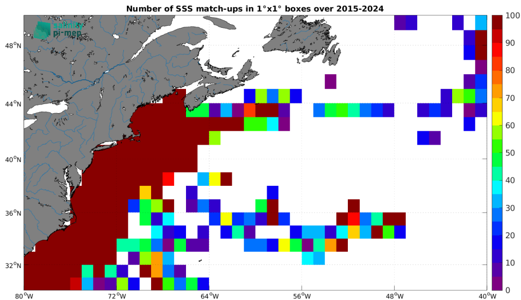
Figure 5: Number of SSS match-ups between TSG (SAMOS) SSS and the SMAP SSS L2 v6 - 40 km (RSS) SSS product for the Gulf Stream Pi-MEP region over 1^\circ \times 1^\circ boxes and for the full satellite product period.
