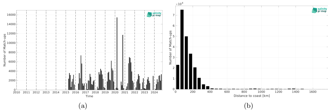
Figure 2: Number of match-ups between TSG (SAMOS) and SMAP SSS L2 v6 - 40 km (RSS) SSS as a function of time (a) and as function of the distance to coast (b) over the Gulf Stream Pi-MEP region and for the full satellite product period.
