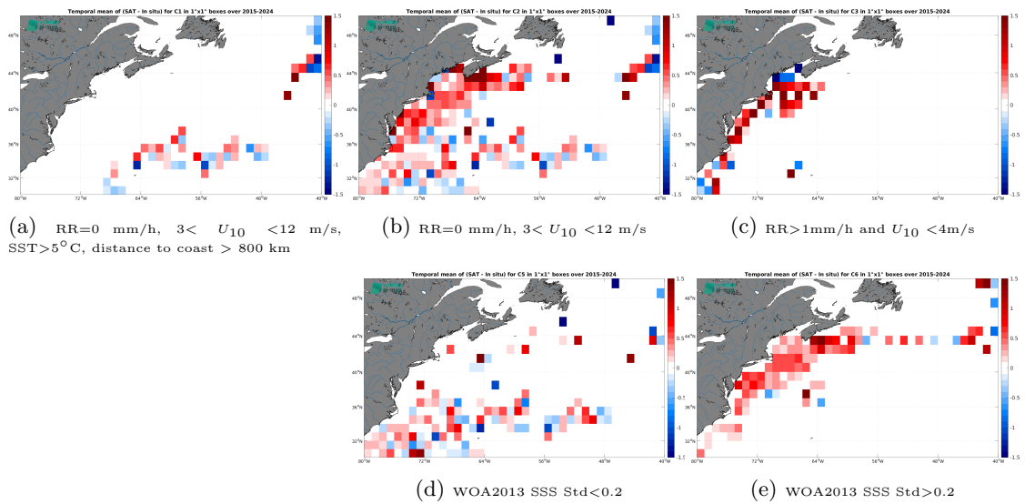
Figure 14: Temporal mean gridded over spatial boxes of size 1^\circ \times 1^\circ of \Delta SSS (SMAP SSS L2 v6 - 40 km (RSS) - TSG (SAMOS)) for 5 different subdatasets corresponding to:RR=0 mm/h, 3 < U_{10} < 12 m/s, SST > 5^\circ C , distance to coast > 800 km (a), RR=0 mm/h, 3 < U_{10} < 12 m/s (b), RR>1mm/h and U_{10} < 4 m/s (c), WOA2013 SSS Std<0.2 (d), WOA2013 SSS Std>0.2 (e).
