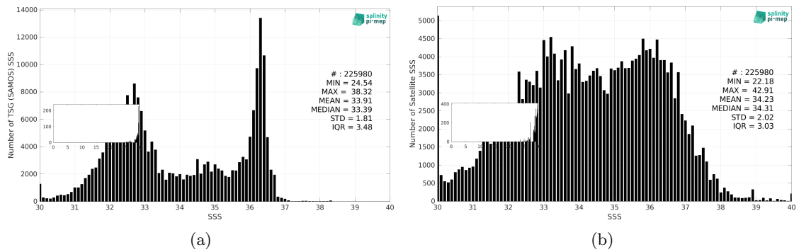
Figure 3: Histograms of SSS from TSG (SAMOS) (a) and SMAP SSS L2 v6 - 40 km (RSS) (b) considering all match-up pairs per bins of 0.1 over the Gulf Stream Pi-MEP region and for the full satellite product period.
