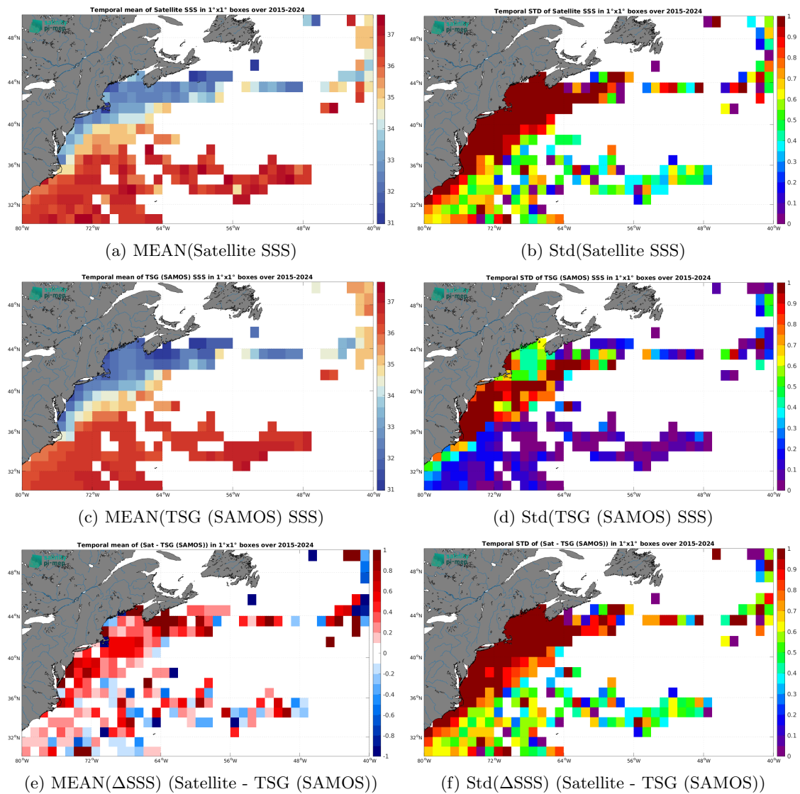
Figure 7: Temporal mean (left) and Std (right) of SSS from SMAP SSS L2 v6 - 40 km (RSS) (top), TSG (SAMOS) (middle), and of \Delta SSS (Satellite - TSG (SAMOS)). Only match-up pairs are used to generate these maps.
